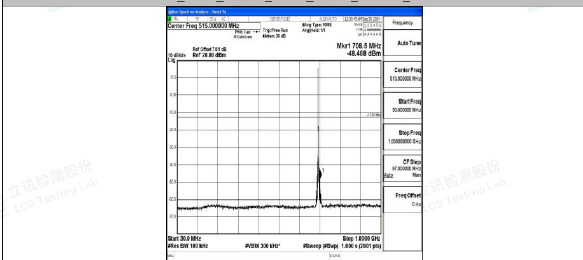
Band12_3MHz_16QAM_23025_1RB#0_30~1000_30~1000
