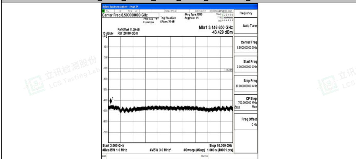
Band12_5MHz_16QAM_23155_1RB#0_3000~10000_3000~10000
