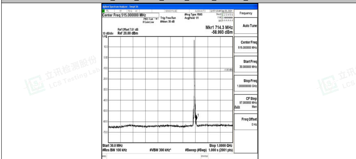
Band12_5MHz_QPSK_23035_1RB#0_30~1000_30~1000
