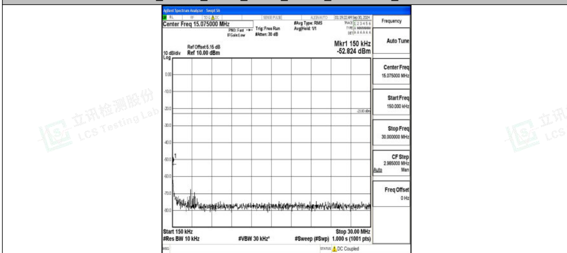
Band12_10MHz_QPSK_23095_1RB#0_0.15~30_0.15~30
