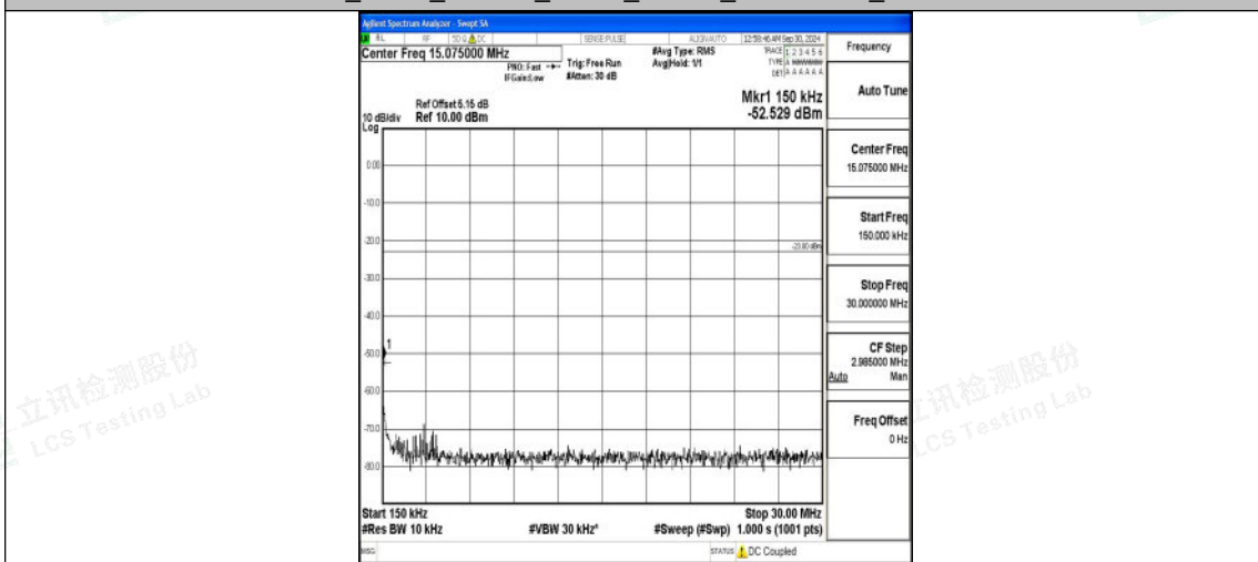
Band12_5MHz_16QAM_23095_1RB#0_0.15~30_0.15~30
