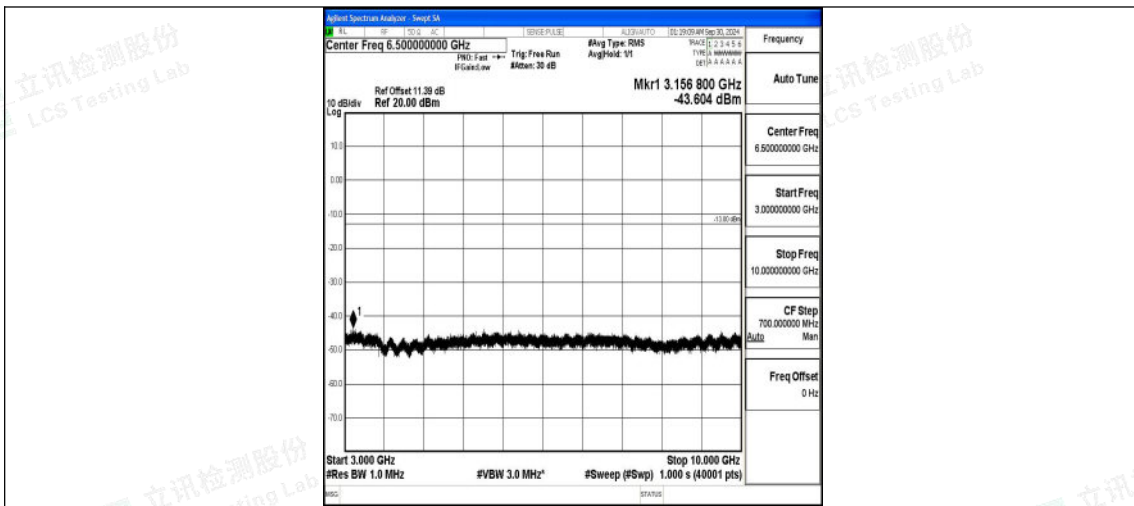
Band12_10MHz_16QAM_23060_1RB#0_3000~10000_3000~10000
