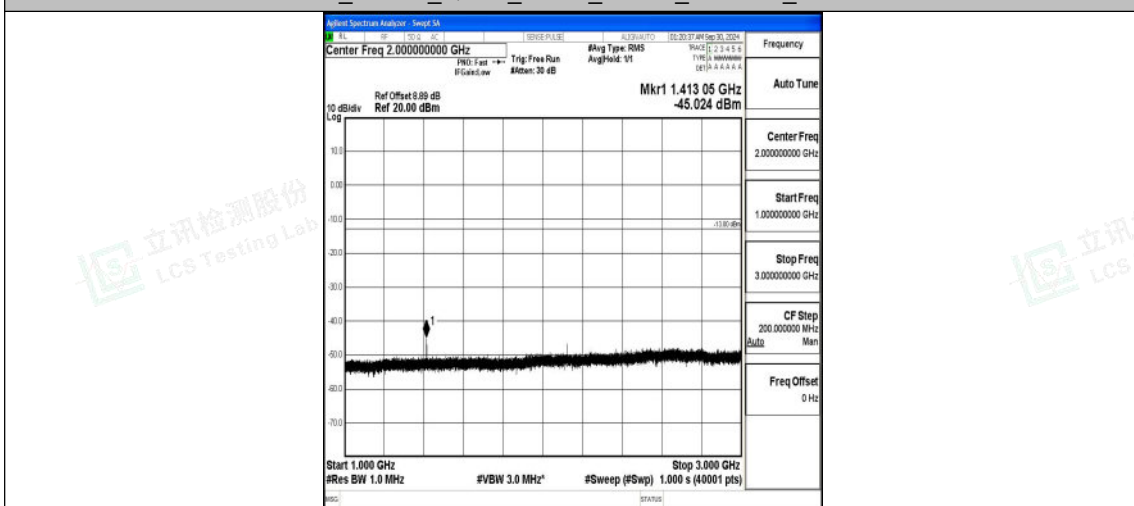
Band12_10MHz_QPSK_23130_1RB#0_1000~3000_1000~3000
