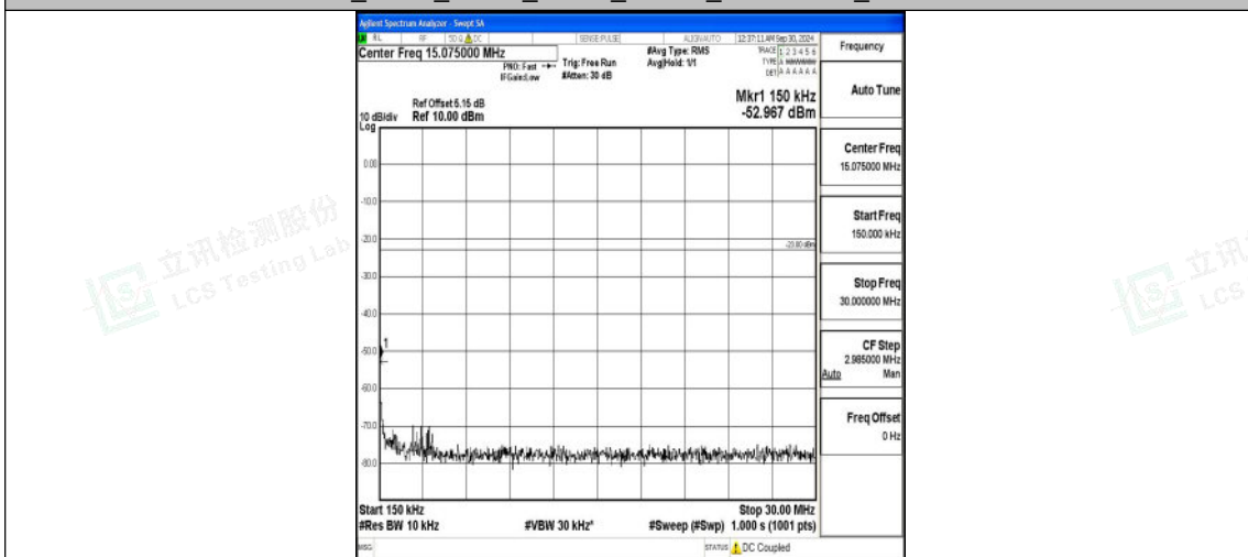
Band12_3MHz_QPSK_23095_1RB#0_0.15~30_0.15~30
