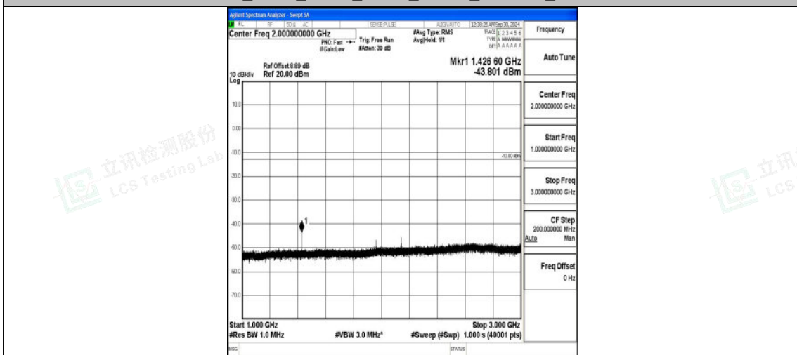
Band12_3MHz_QPSK_23165_1RB#0_1000~3000_1000~3000
