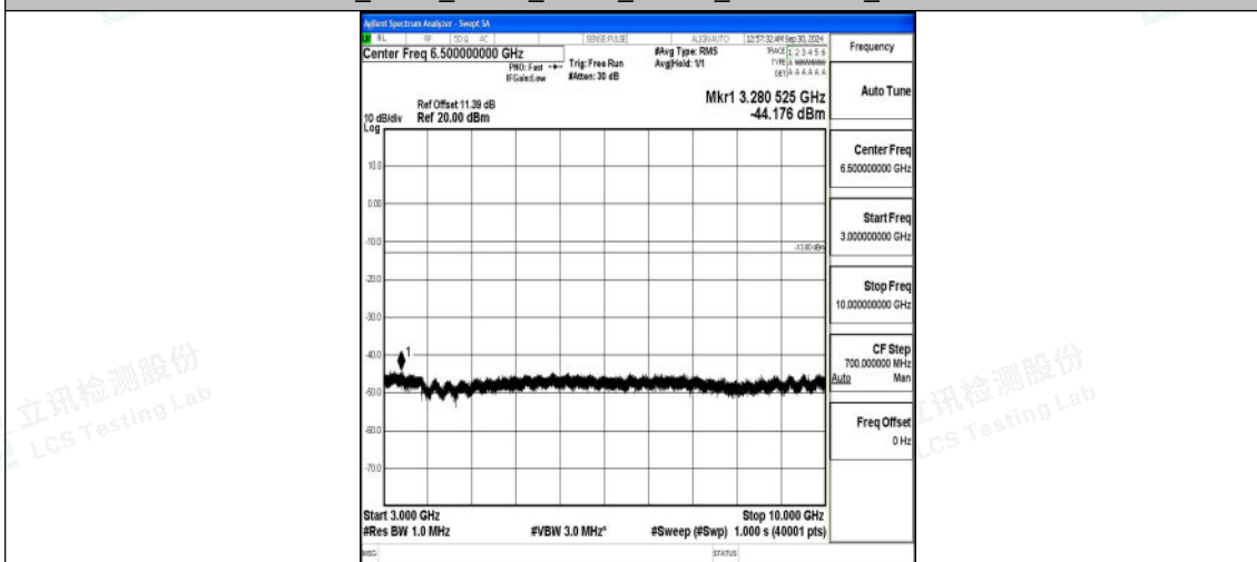
Band12_5MHz_QPSK_23035_1RB#0_3000~10000_3000~10000
