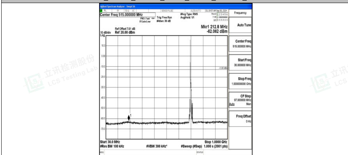
Band12_10MHz_16QAM_23095_1RB#0_30~1000_30~1000
