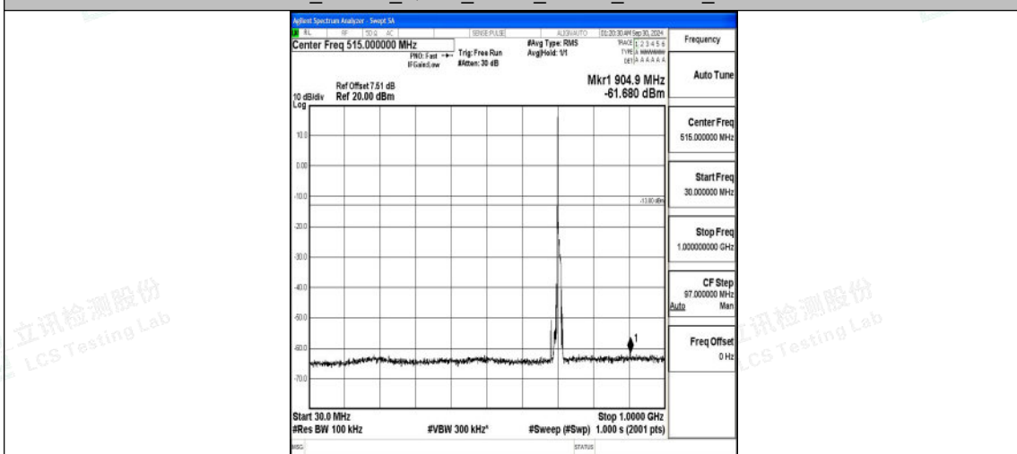
Band12_10MHz_QPSK_23130_1RB#0_30~1000_30~1000
