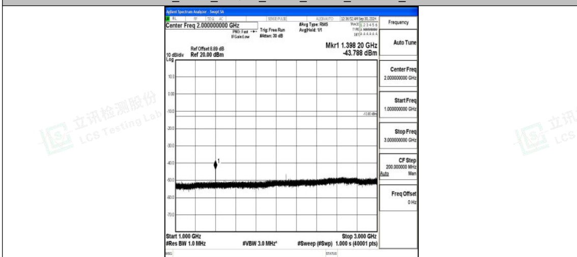
Band12_3MHz_16QAM_23025_1RB#0_1000~3000_1000~3000
