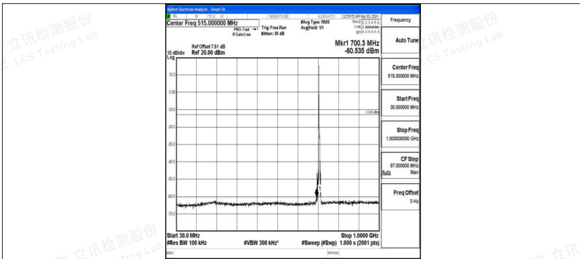
Band12_5MHz_16QAM_23155_1RB#0_30~1000_30~1000
