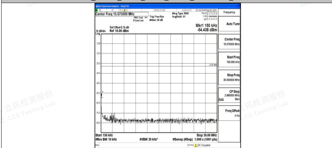
Band12_10MHz_QPSK_23060_1RB#0_0.15~30_0.15~30
