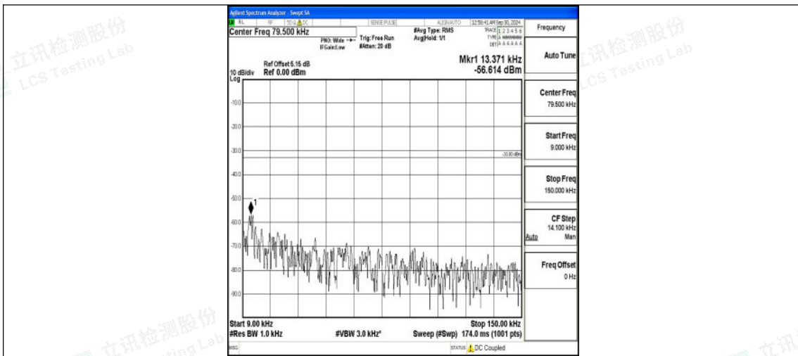
Band12_5MHz_16QAM_23095_1RB#0_0.009~0.15_0.009~0.15
