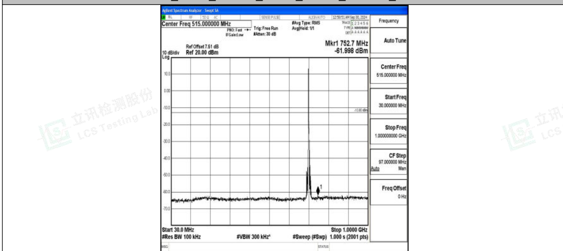
Band12_5MHz_16QAM_23095_1RB#0_30~1000_30~1000
