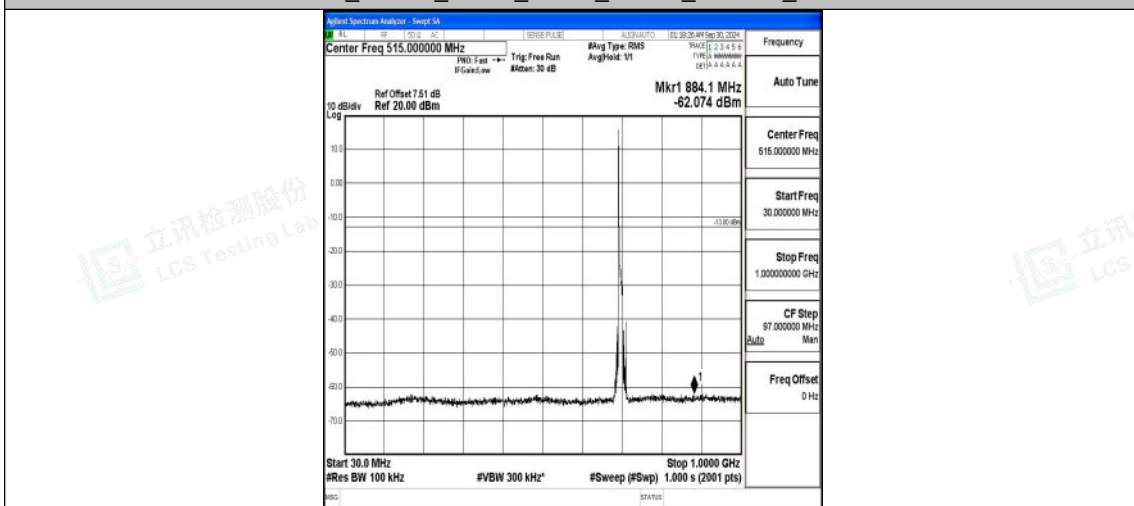
Band12_10MHz_QPSK_23060_1RB#0_30~1000_30~1000
