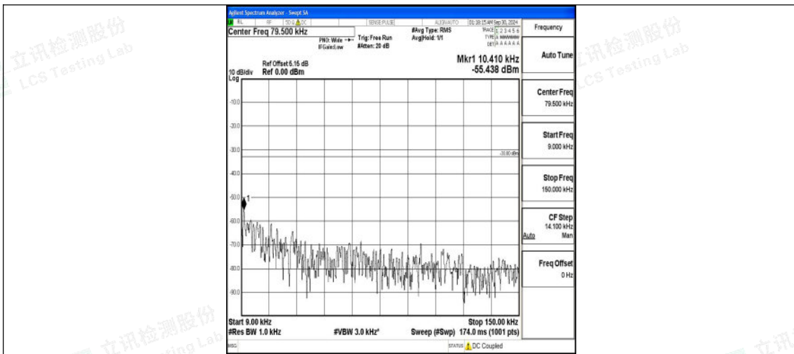
Band12_10MHz_QPSK_23060_1RB#0_0.009~0.15_0.009~0.15
