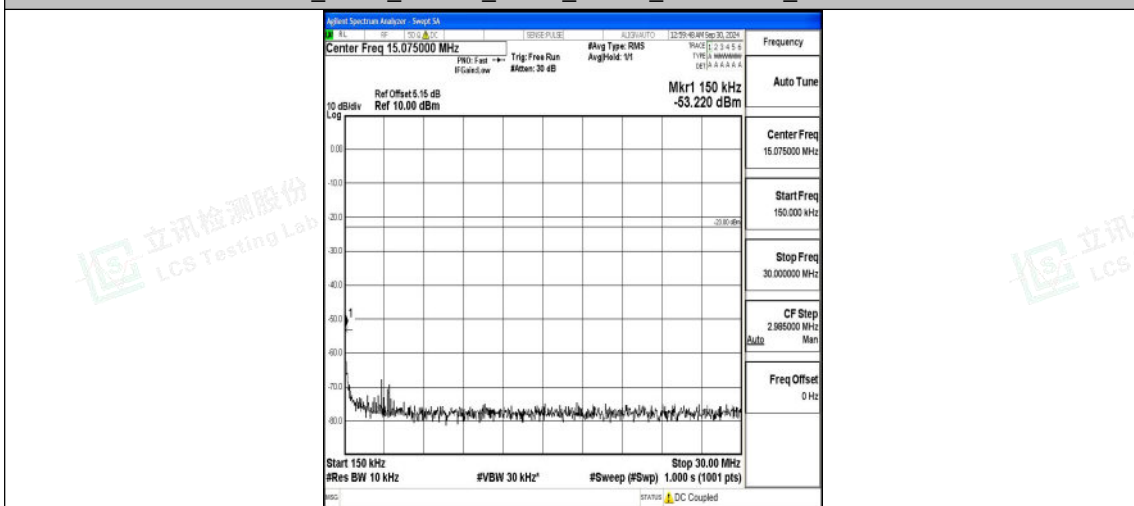
Band12_5MHz_16QAM_23155_1RB#0_0.15~30_0.15~30
