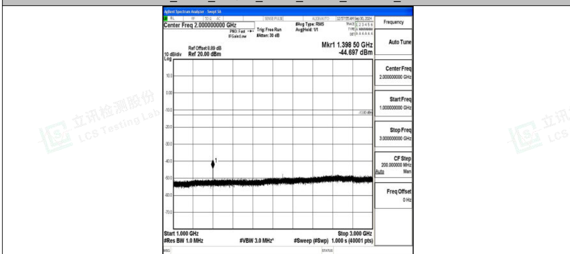
Band12_5MHz_16QAM_23035_1RB#0_1000~3000_1000~3000
