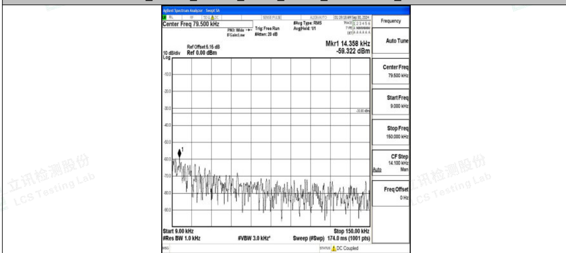
Band12_10MHz_QPSK_23095_1RB#0_0.009~0.15_0.009~0.15
