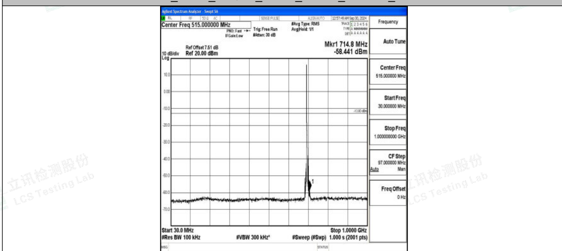
Band12_5MHz_16QAM_23035_1RB#0_30~1000_30~1000
