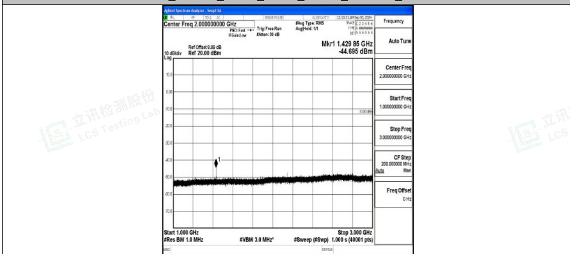
Band12_1.4MHz_QPSK_23173_1RB#0_1000~3000_1000~3000
