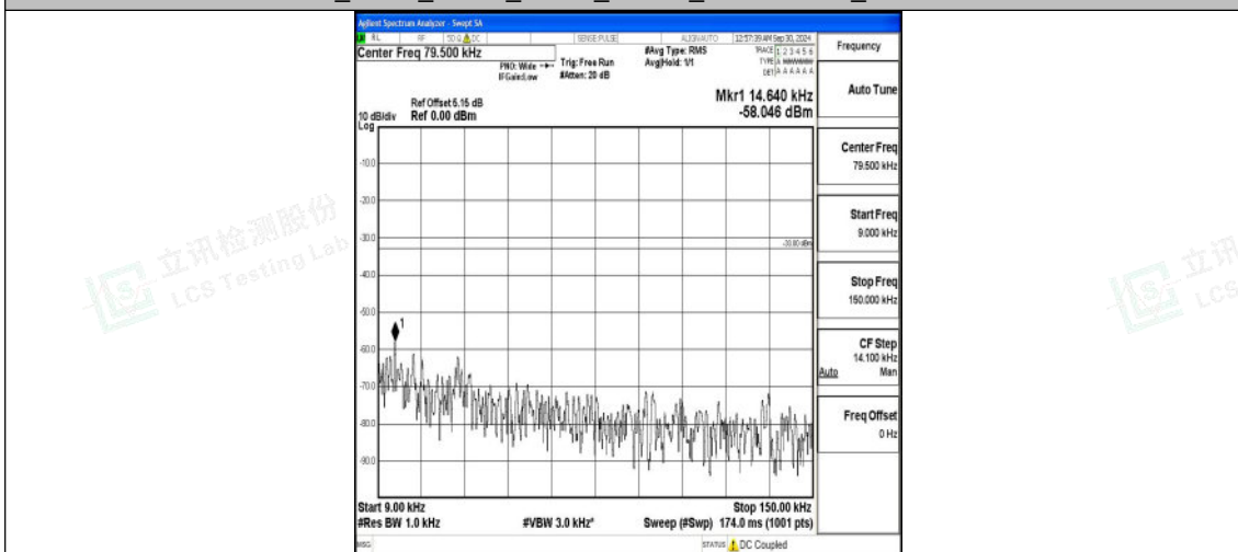
Band12_5MHz_16QAM_23035_1RB#0_0.009~0.15_0.009~0.15
