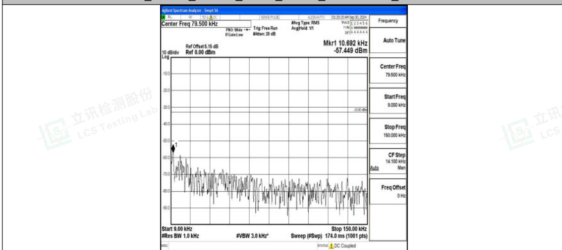
Band12_10MHz_QPSK_23130_1RB#0_0.009~0.15_0.009~0.15
