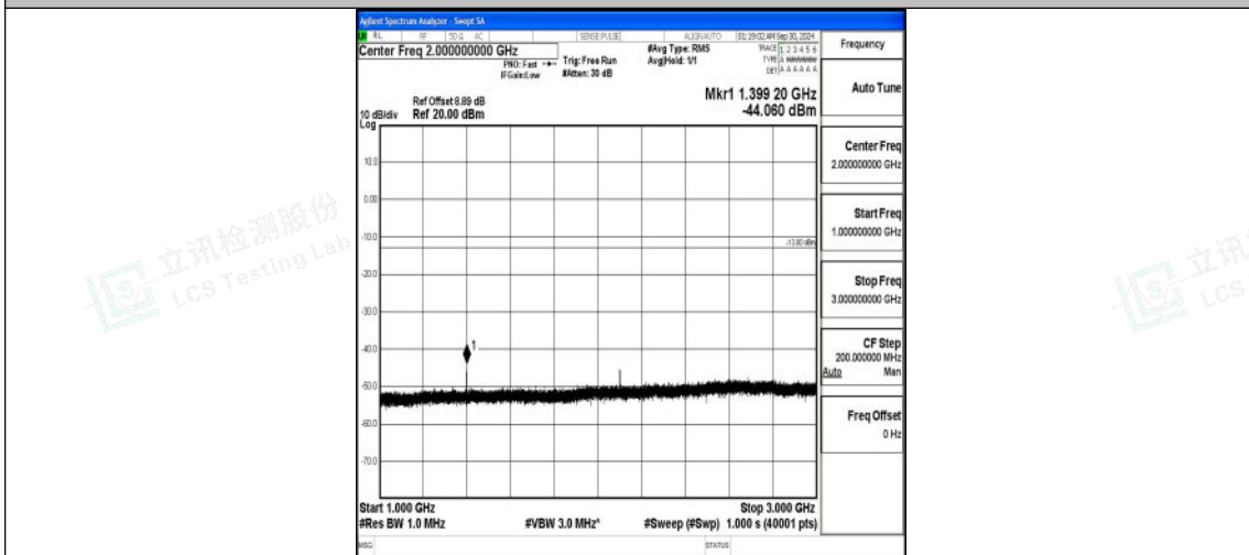
Band12_10MHz_16QAM_23060_1RB#0_1000~3000_1000~3000
