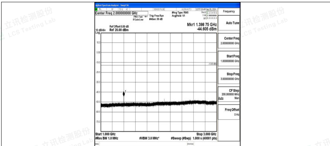
Band12_5MHz_QPSK_23035_1RB#0_1000~3000_1000~3000
