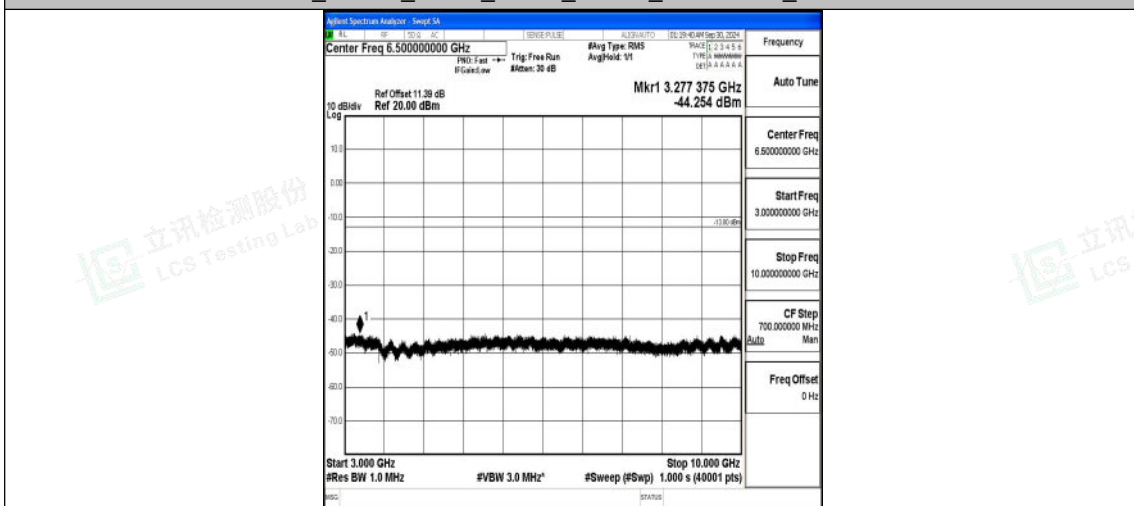
Band12_10MHz_QPSK_23095_1RB#0_3000~10000_3000~10000
