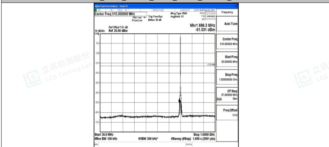
Band12_3MHz_16QAM_23095_1RB#0_30~1000_30~1000
