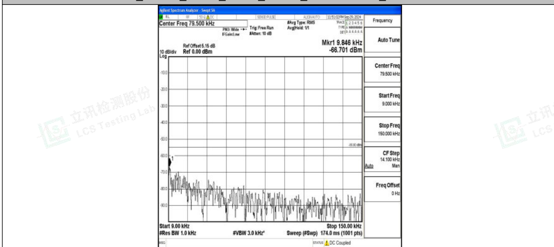
Band7_20MHz_16QAM_20850_1RB#0_0.009~0.15_0.009~0.15
