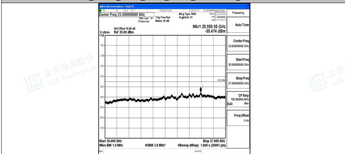
Band7_10MHz_QPSK_21100_1RB#0_20000~27000_20000~27000
