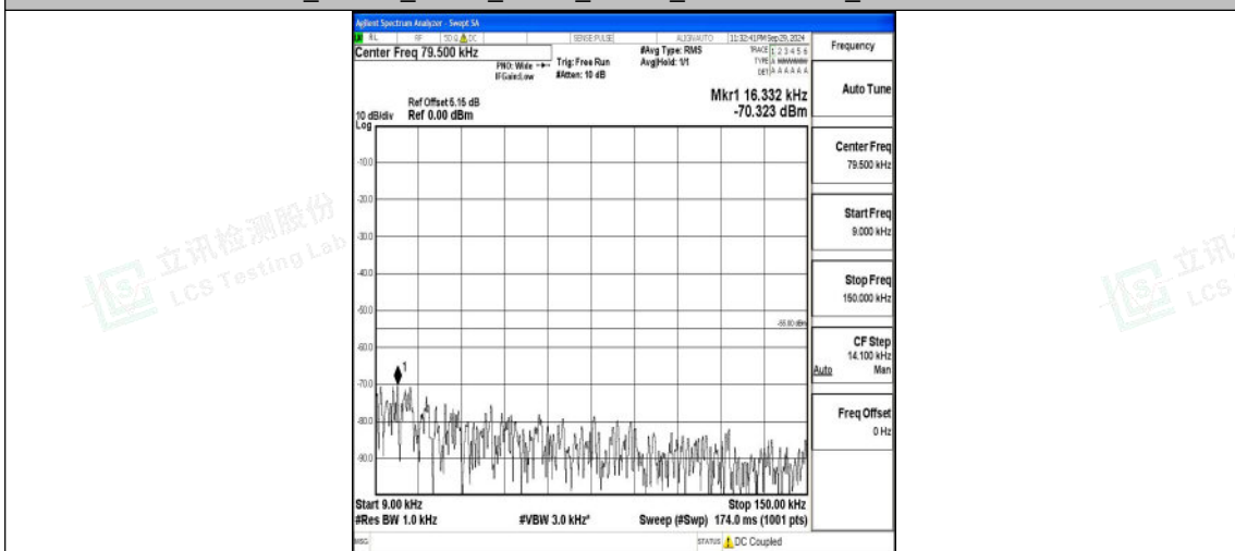
Band7_15MHz_16QAM_20825_1RB#0_0.009~0.15_0.009~0.15
