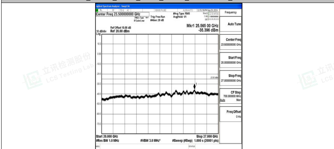
Band7_20MHz_QPSK_21100_1RB#0_20000~27000_20000~27000
