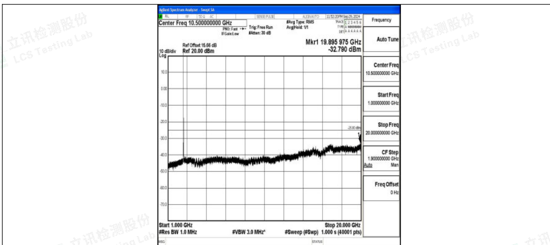
Band7_20MHz_16QAM_21100_1RB#0_1000~20000_1000~20000
