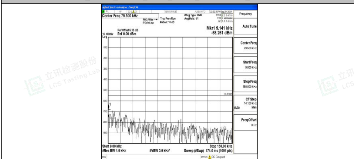
Band7_20MHz_QPSK_21350_1RB#0_0.009~0.15_0.009~0.15
