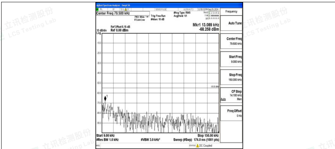
Band7_20MHz_QPSK_20850_1RB#0_0.009~0.15_0.009~0.15
