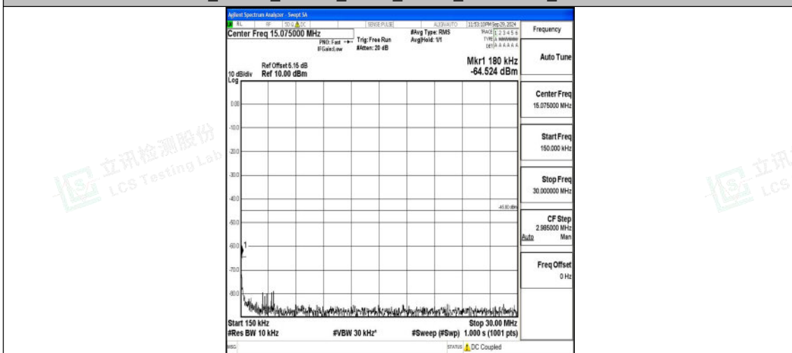
Band7_20MHz_16QAM_21350_1RB#0_0.15~30_0.15~30
