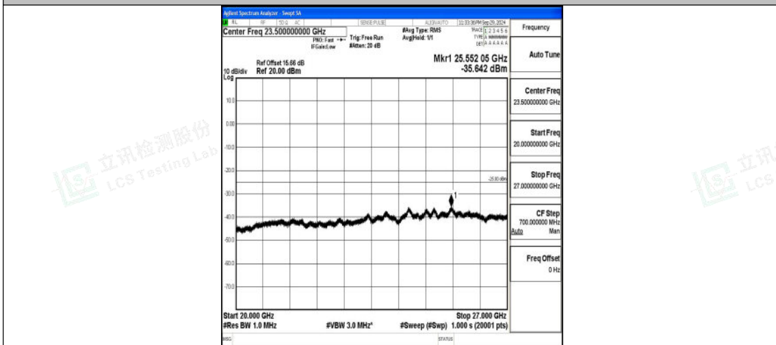
Band7_15MHz_QPSK_21100_1RB#0_20000~27000_20000~27000
