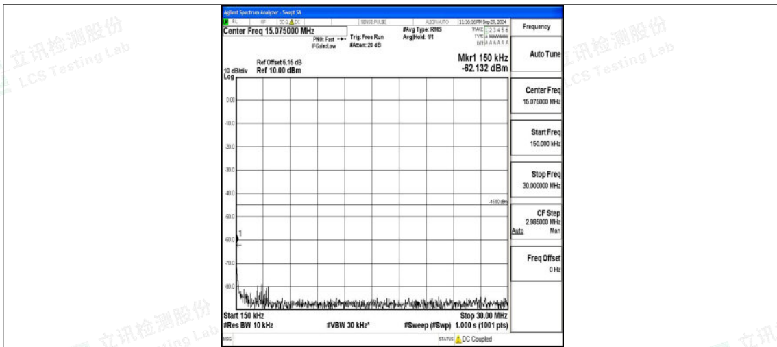
Band7_10MHz_QPSK_21400_1RB#0_0.15~30_0.15~30
