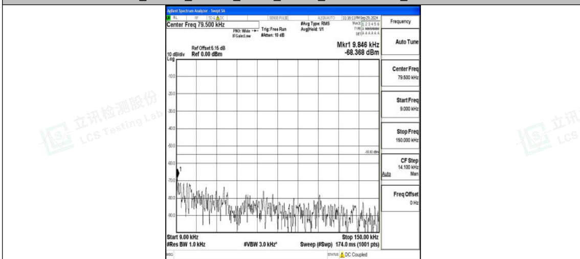
Band7_10MHz_QPSK_21400_1RB#0_0.009~0.15_0.009~0.15
