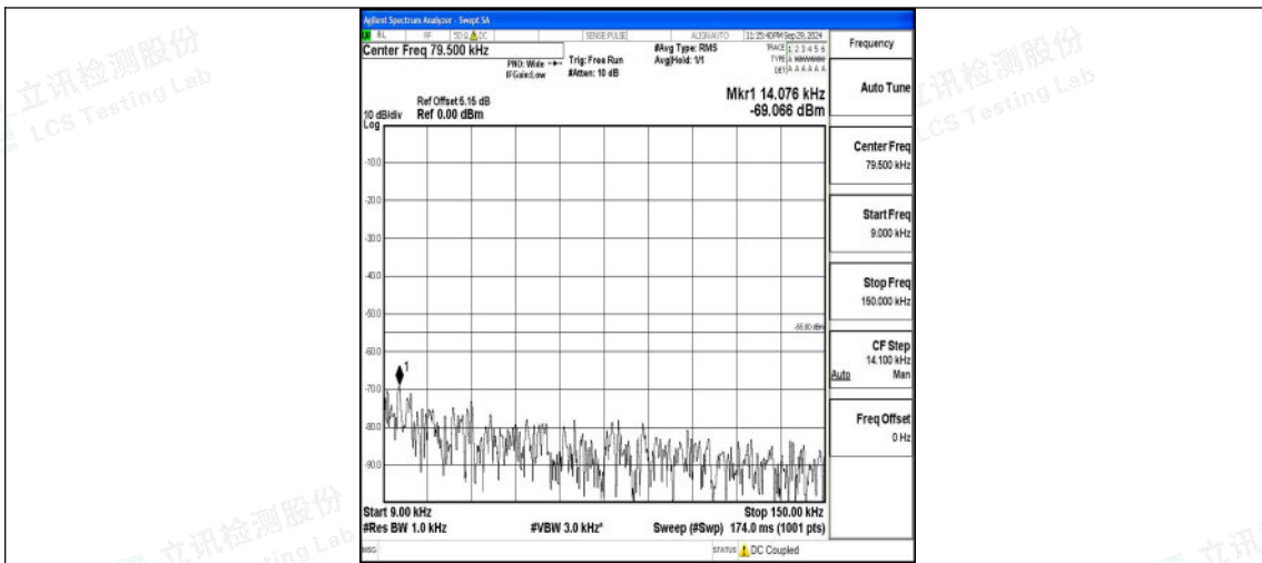
Band7_10MHz_16QAM_21100_1RB#0_0.009~0.15_0.009~0.15
