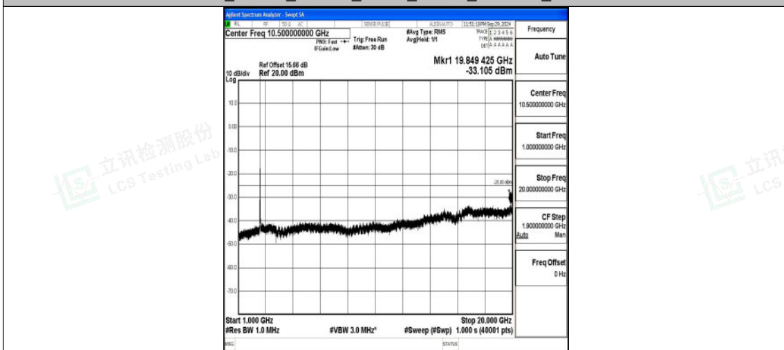
Band7_20MHz_16QAM_20850_1RB#0_1000~20000_1000~20000
