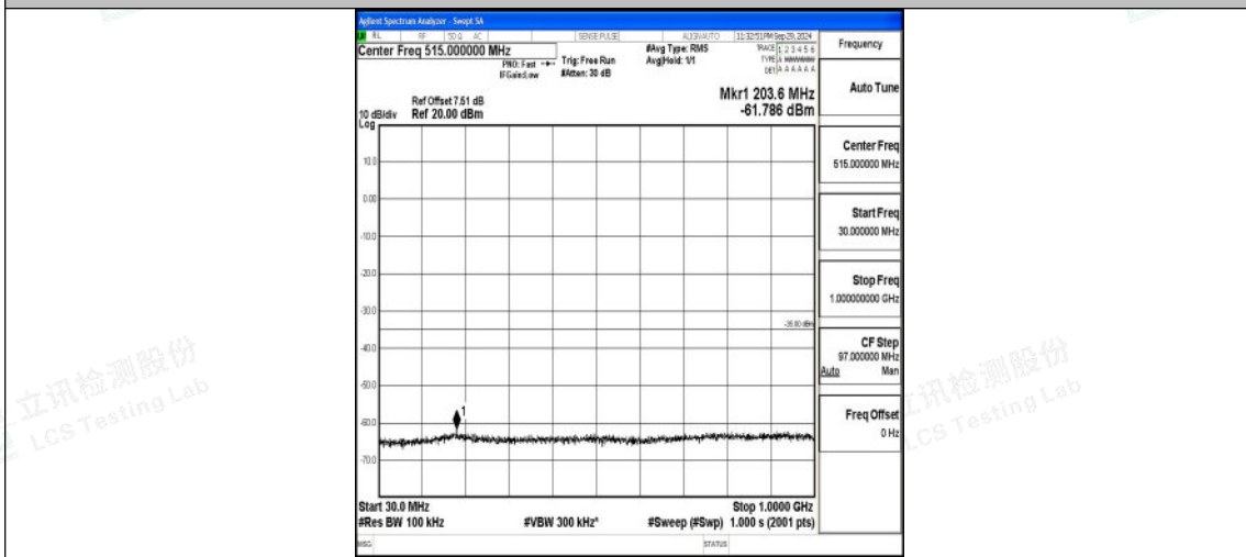
Band7_15MHz_16QAM_20825_1RB#0_30~1000_30~1000
