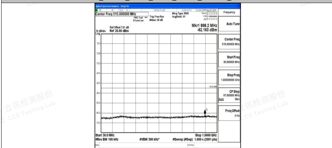
Band7_10MHz_QPSK_21400_1RB#0_30~1000_30~1000
