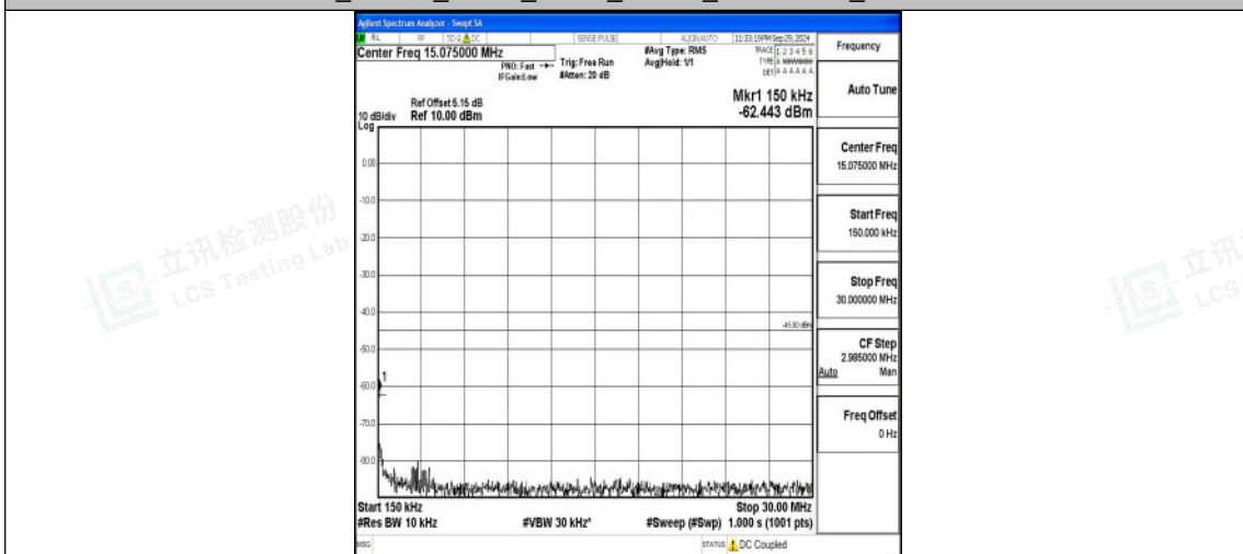
Band7_15MHz_QPSK_21100_1RB#0_0.15~30_0.15~30
