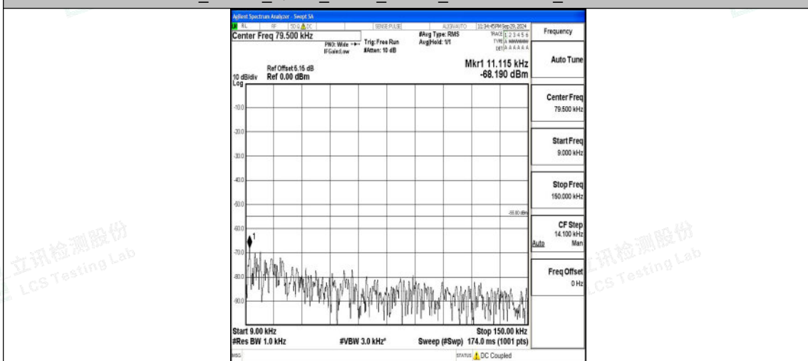
Band7_15MHz_16QAM_21375_1RB#0_0.009~0.15_0.009~0.15
