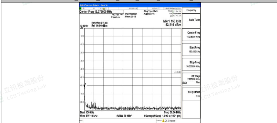
Band7_20MHz_QPSK_20850_1RB#0_0.15~30_0.15~30
