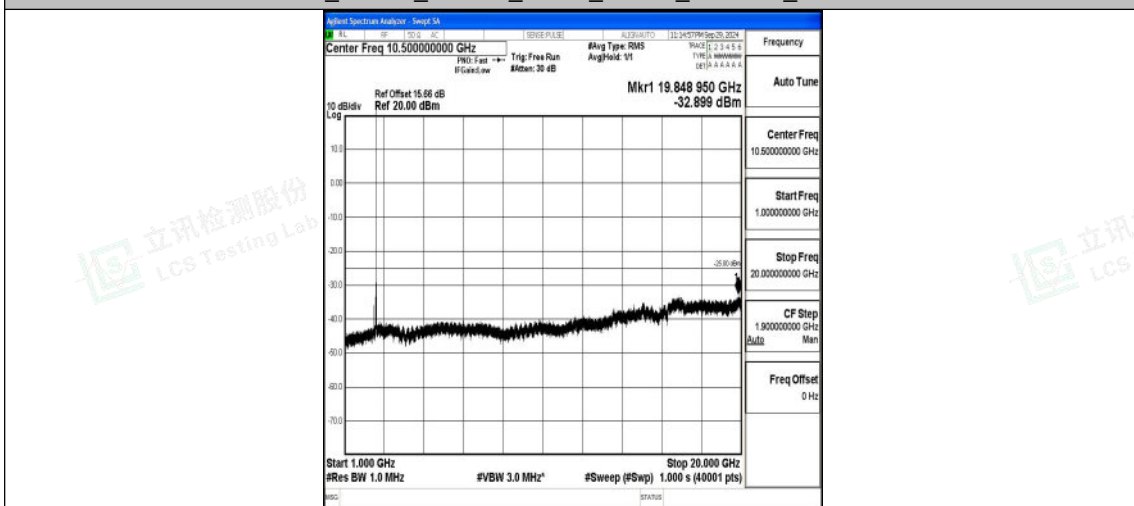
Band7_10MHz_16QAM_20800_1RB#0_1000~20000_1000~20000
