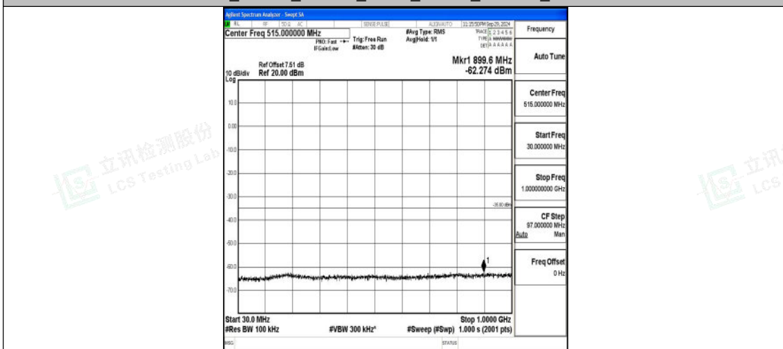
Band7_10MHz_16QAM_21100_1RB#0_30~1000_30~1000
