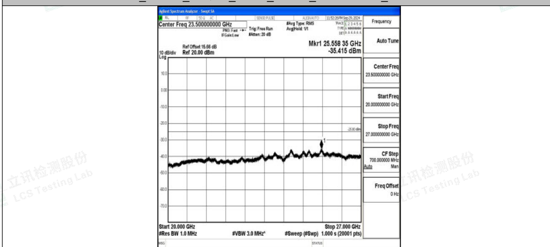
Band7_20MHz_16QAM_21100_1RB#0_20000~27000_20000~27000
