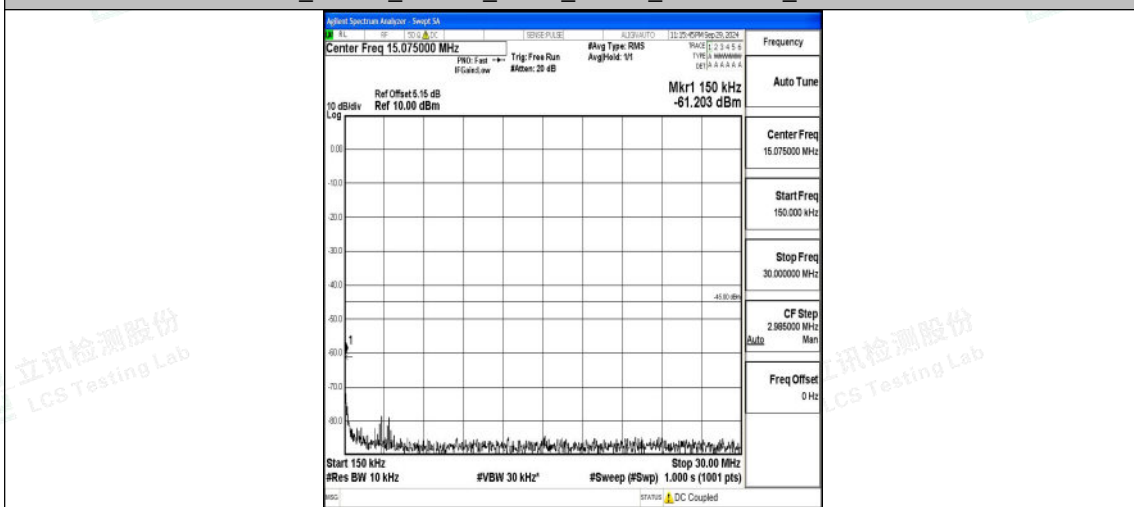
Band7_10MHz_16QAM_21100_1RB#0_0.15~30_0.15~30
