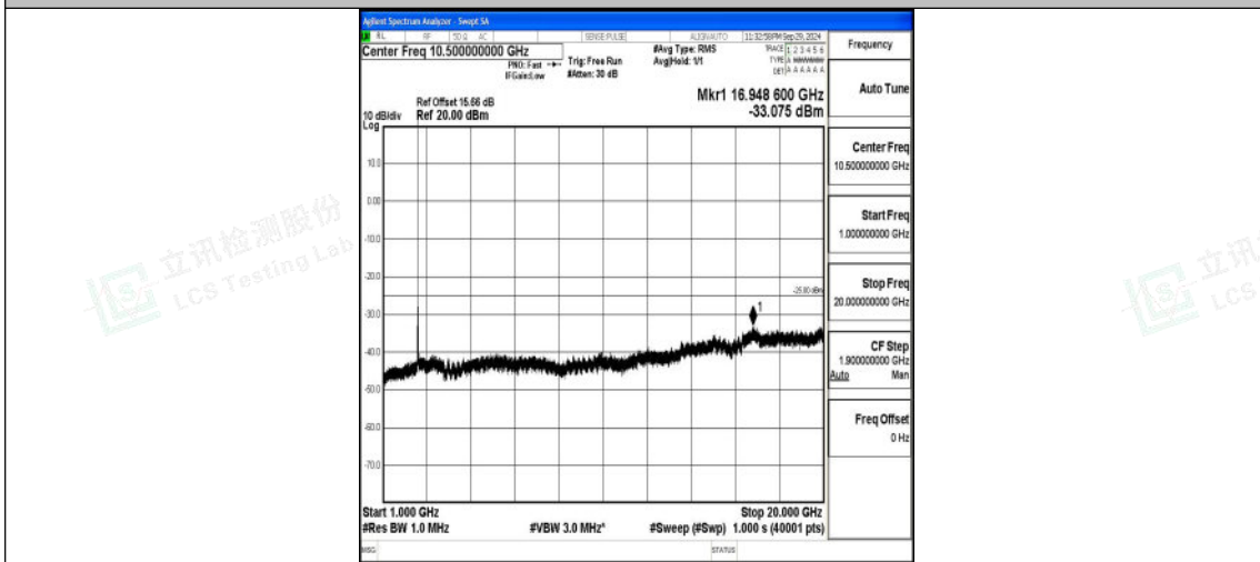
Band7_15MHz_16QAM_20825_1RB#0_1000~20000_1000~20000
