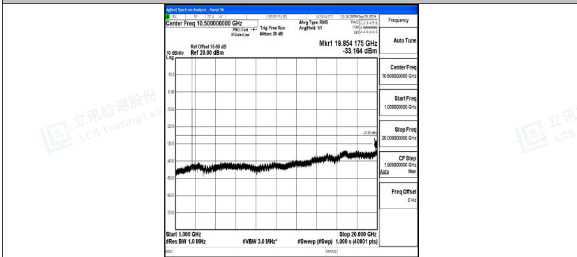
Band7_10MHz_QPSK_21400_1RB#0_1000~20000_1000~20000
