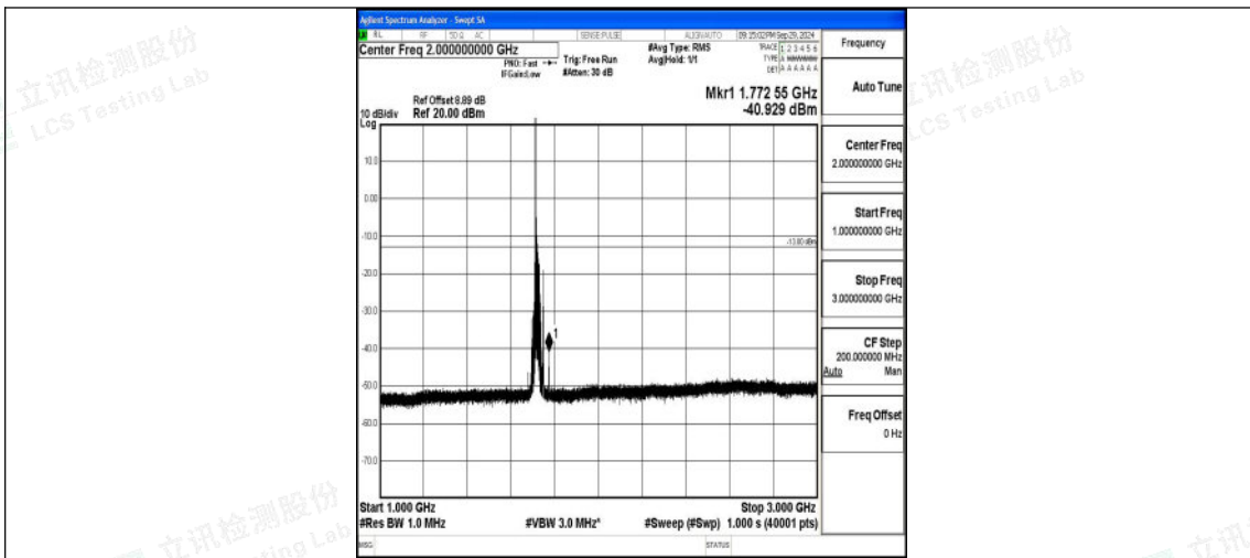
Band4_20MHz_QPSK_20050_1RB#0_1000~3000_1000~3000
