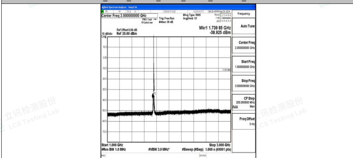
Band4_5MHz_16QAM_20375_1RB#0_1000~3000_1000~3000
