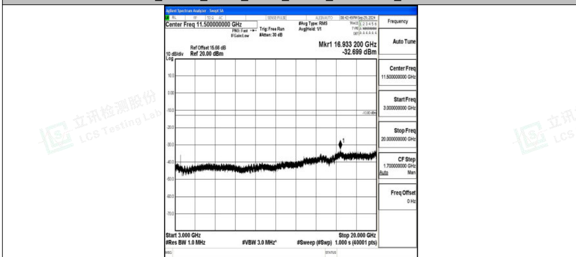
Band4_10MHz_QPSK_20175_1RB#0_3000~20000_3000~20000
