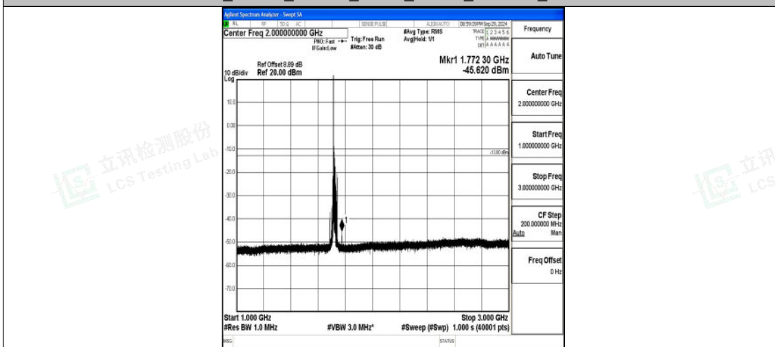
Band4_15MHz_16QAM_2025_1RB#0_1000~3000_1000~3000
