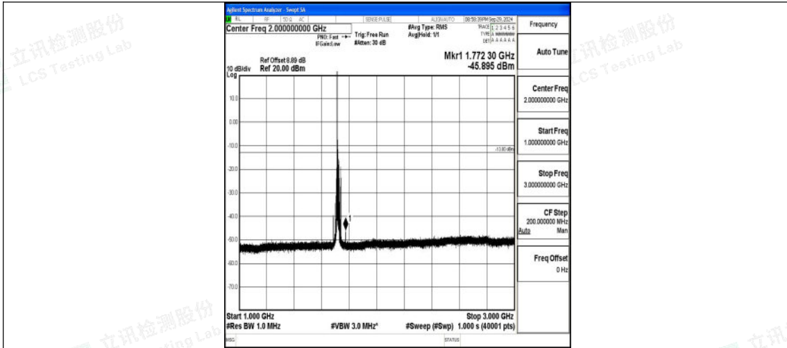
Band4_15MHz_QPSK_2025_1RB#0_1000~3000_1000~3000
