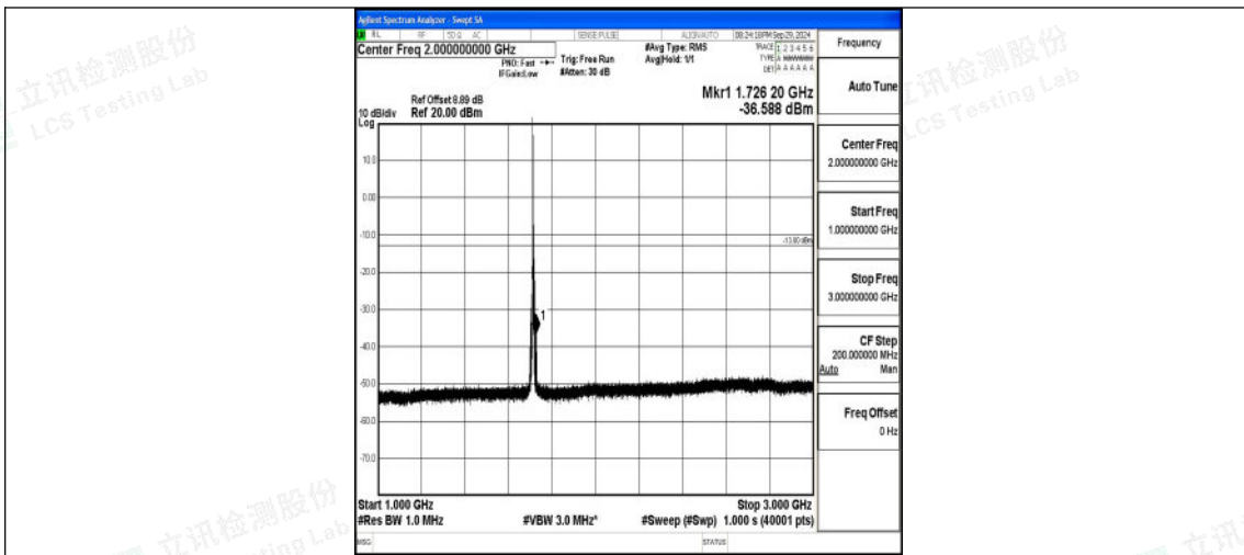
Band4_5MHz_QPSK_19975_1RB#0_1000~3000_1000~3000
