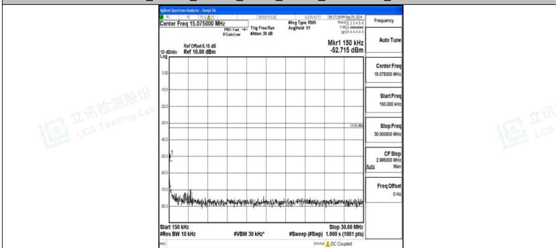
Band4_20MHz_16QAM_20300_1RB#0_0.15~30_0.15~30
