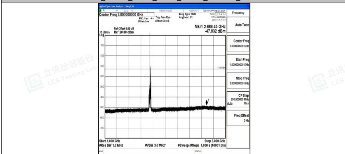
Band4_10MHz_QPSK_20350_1RB#0_1000~3000_1000~3000
