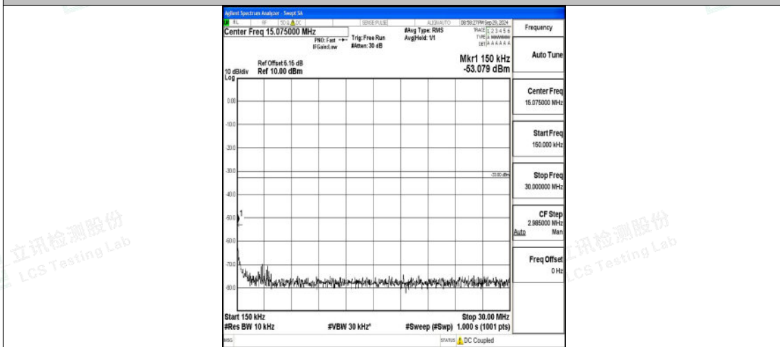
Band4_15MHz_QPSK_2025_1RB#0_0.15~30_0.15~30
