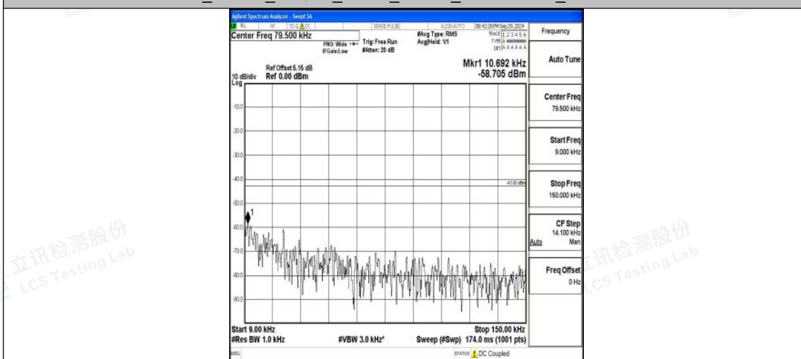
Band4_10MHz_QPSK_20175_1RB#0_0.009~0.15_0.009~0.15
