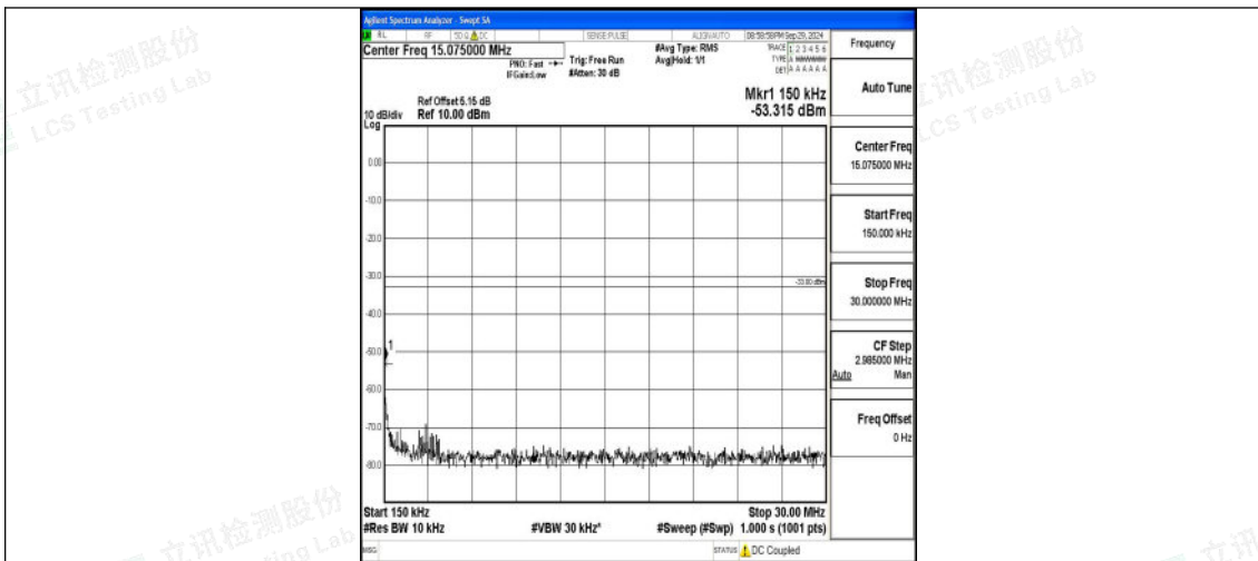
Band4_15MHz_16QAM_2025_1RB#0_0.15~30_0.15~30
