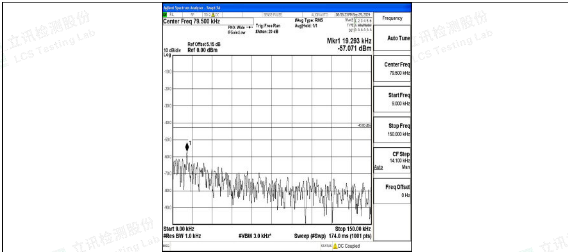
Band4_15MHz_QPSK_2025_1RB#0_0.009~0.15_0.009~0.15
