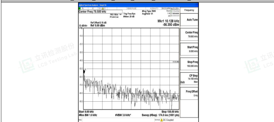
Band4_20MHz_16QAM_20050_1RB#0_0.009~0.15_0.009~0.15
