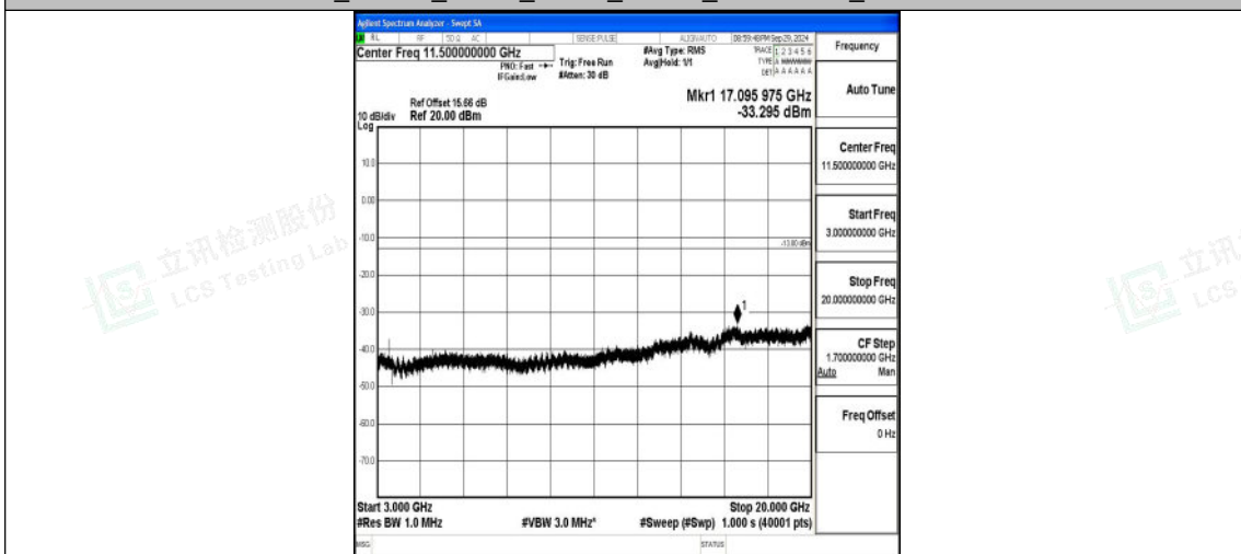
Band4_15MHz_QPSK_20175_1RB#0_3000~20000_3000~20000
