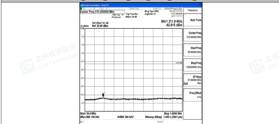
Band4_15MHz_16QAM_20175_1RB#0_30~1000_30~1000
