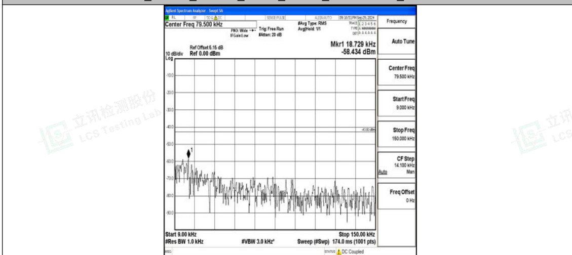
Band4_20MHz_QPSK_20300_1RB#0_0.009~0.15_0.009~0.15
