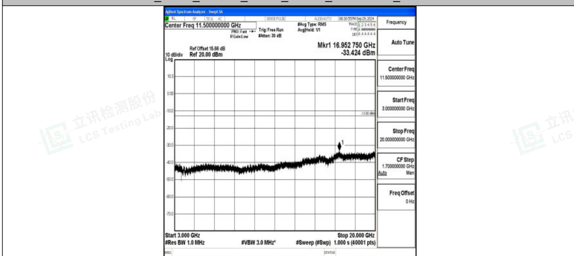
Band4_5MHz_16QAM_20375_1RB#0_3000~20000_3000~20000
