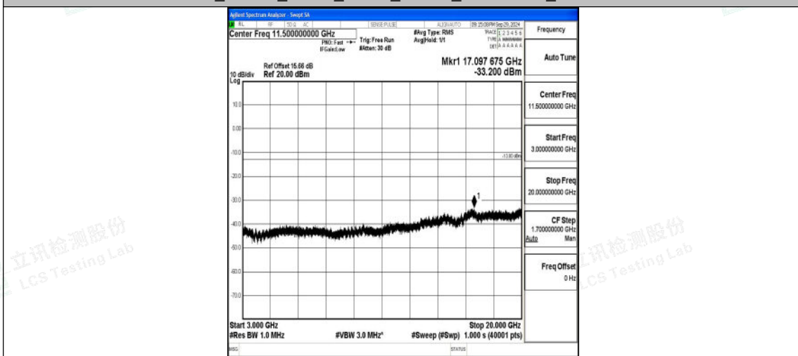
Band4_20MHz_QPSK_20050_1RB#0_3000~20000_3000~20000
