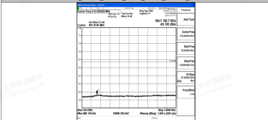
Band4_15MHz_16QAM_2025_1RB#0_30~1000_30~1000
