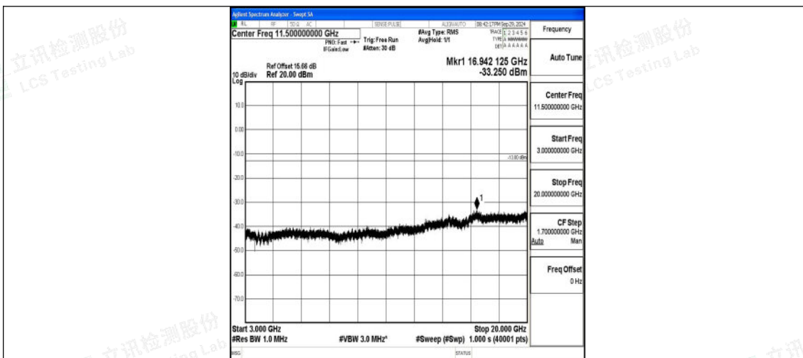
Band4_10MHz_16QAM_20000_1RB#0_3000~20000_3000~20000
