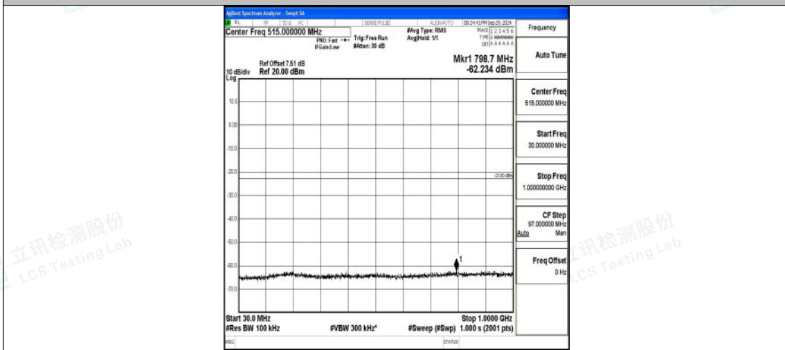
Band4_5MHz_16QAM_19975_1RB#0_30~1000_30~1000
