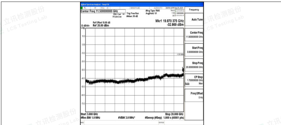
Band4_15MHz_16QAM_2025_1RB#0_3000~20000_3000~20000
