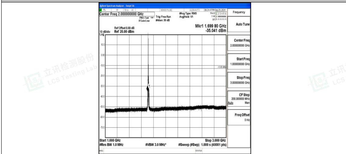
Band4_5MHz_16QAM_19975_1RB#0_1000~3000_1000~3000
