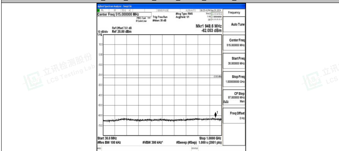
Band4_5MHz_16QAM_20175_1RB#0_30~1000_30~1000
