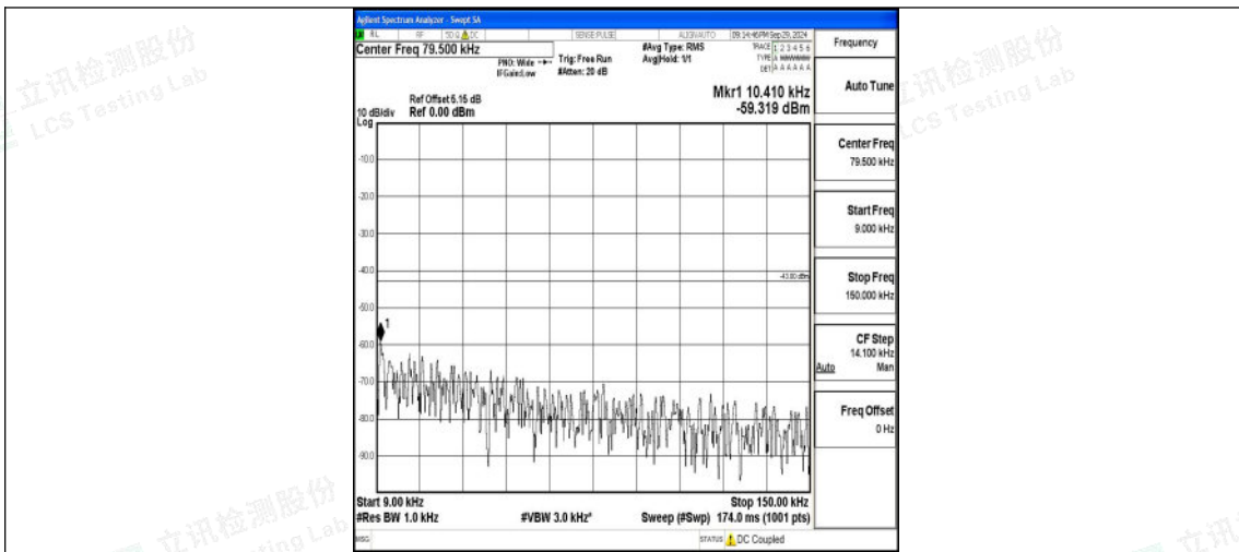
Band4_20MHz_QPSK_20050_1RB#0_0.009~0.15_0.009~0.15
