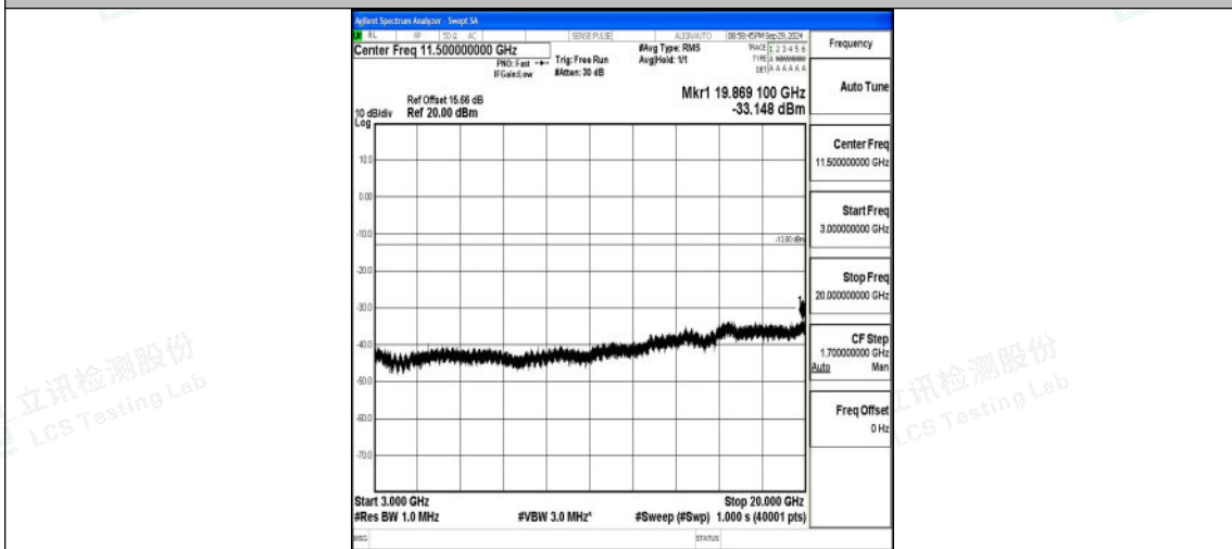
Band4_15MHz_QPSK_2025_1RB#0_3000~20000_3000~20000
