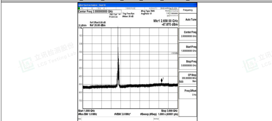
Band4_15MHz_QPSK_20325_1RB#0_1000~3000_1000~3000
