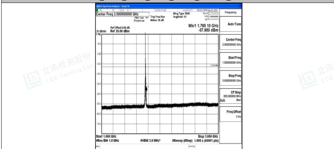
Band4_5MHz_QPSK_20375_1RB#0_1000~3000_1000~3000
