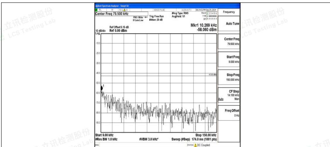
Band4_5MHz_QPSK_19975_1RB#0_0.009~0.15_0.009~0.15
