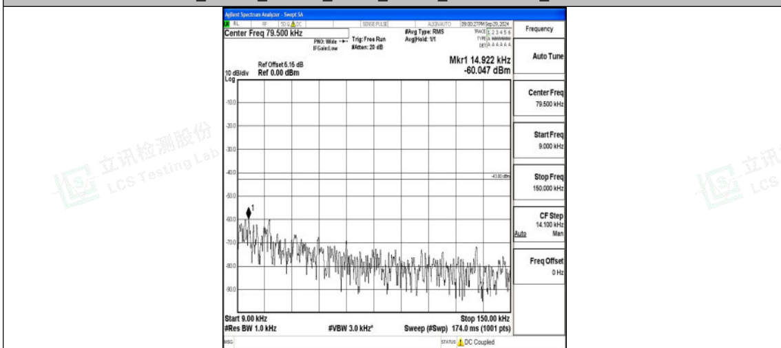
Band4_15MHz_QPSK_20325_1RB#0_0.009~0.15_0.009~0.15
