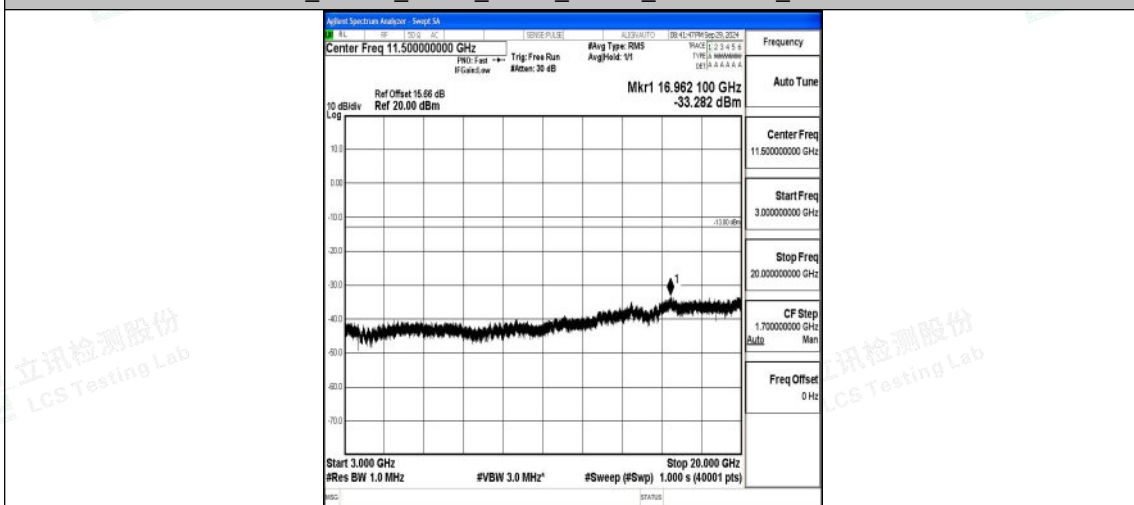
Band4_10MHz_QPSK_20000_1RB#0_3000~20000_3000~20000
