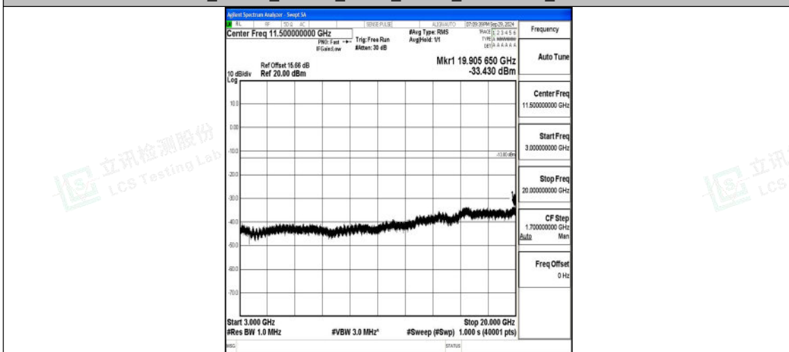
Band2_15MHz_16QAM_19125_1RB#0_3000~20000_3000~20000
