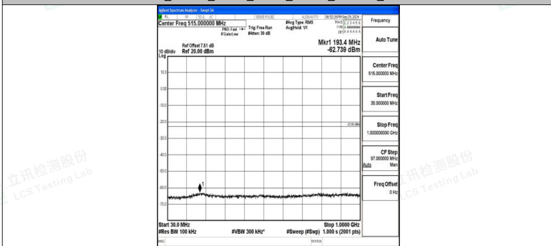
Band2_10MHz_QPSK_19150_1RB#0_30~1000_30~1000
