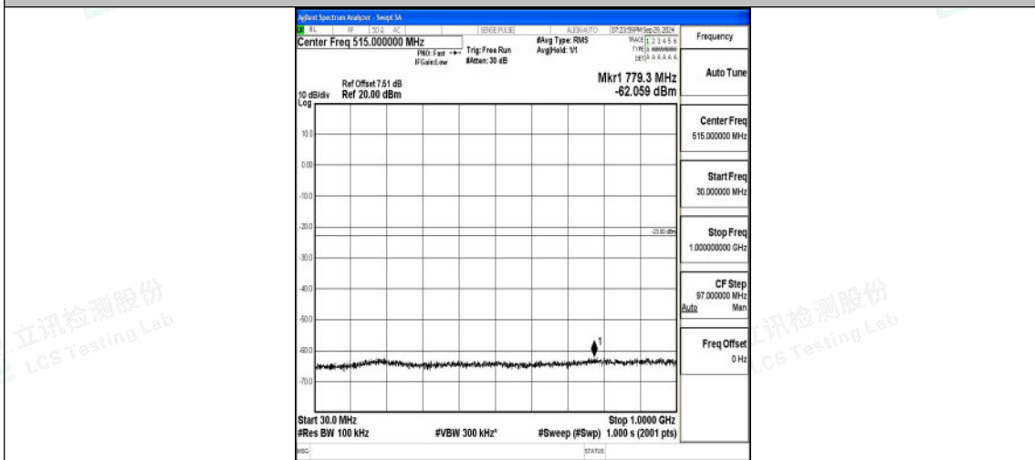
Band2_20MHz_16QAM_18700_1RB#0_30~1000_30~1000
