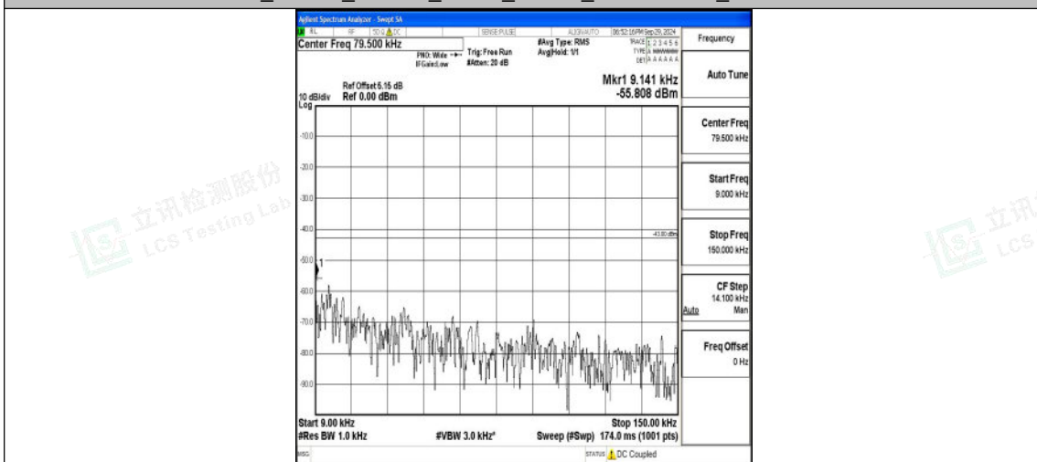
Band2_10MHz_QPSK_19150_1RB#0_0.009~0.15_0.009~0.15
