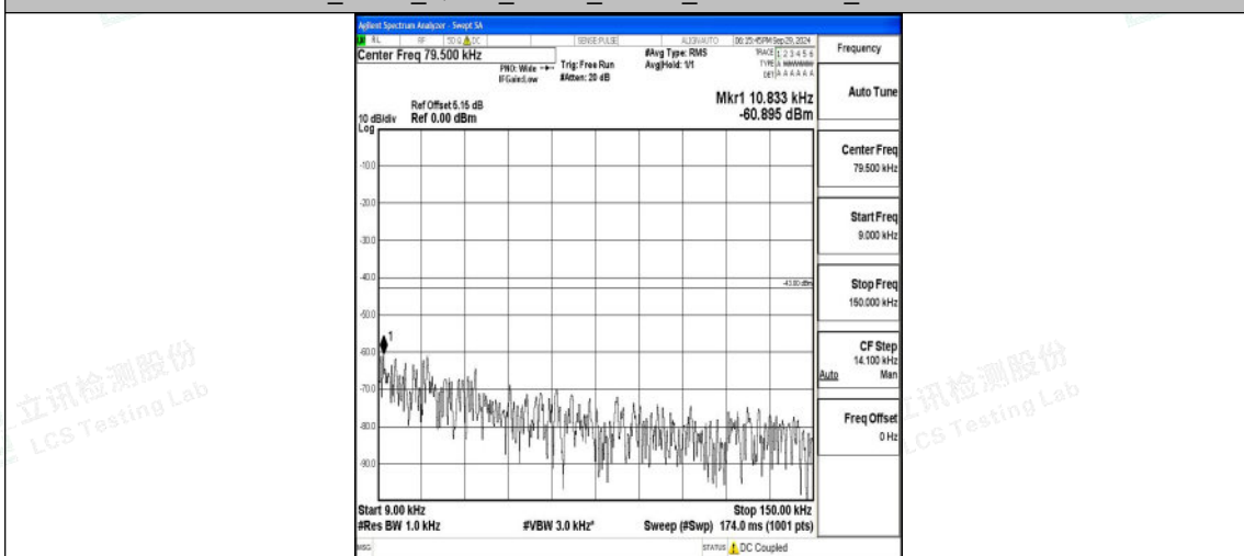
Band2_3MHz_16QAM_19185_1RB#0_0.009~0.15_0.009~0.15
