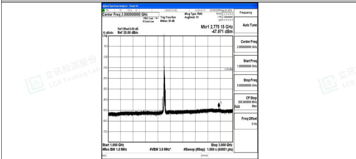
Band2_15MHz_QPSK_19125_1RB#0_1000~3000_1000~3000
