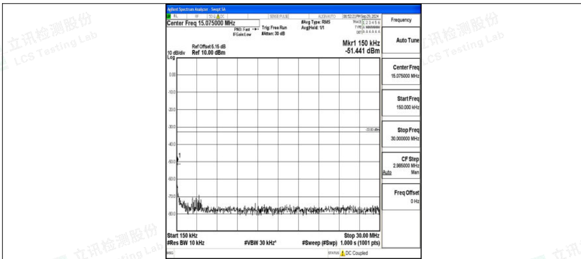
Band2_10MHz_QPSK_19150_1RB#0_0.15~30_0.15~30
