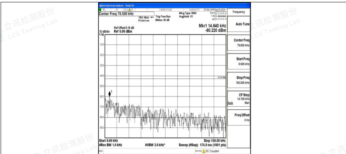
Band2_15MHz_16QAM_18900_1RB#0_0.009~0.15_0.009~0.15
