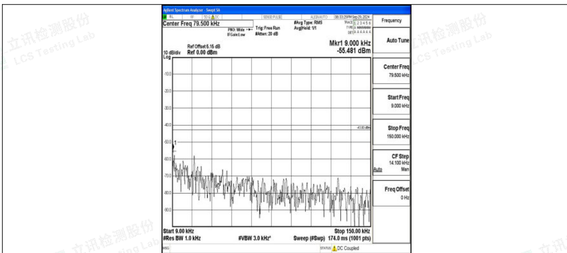
Band2_5MHz_16QAM_18900_1RB#0_0.009~0.15_0.009~0.15
