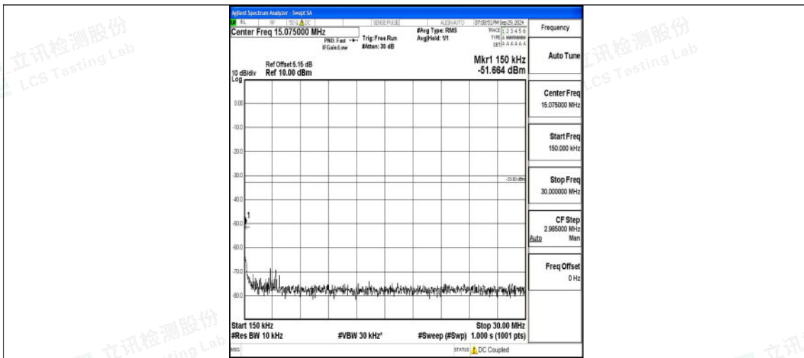
Band2_15MHz_QPSK_19125_1RB#0_0.15~30_0.15~30
