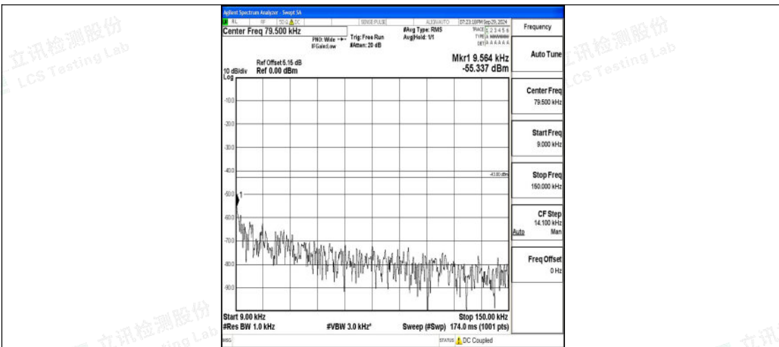
Band2_20MHz_QPSK_18700_1RB#0_0.009~0.15_0.009~0.15
