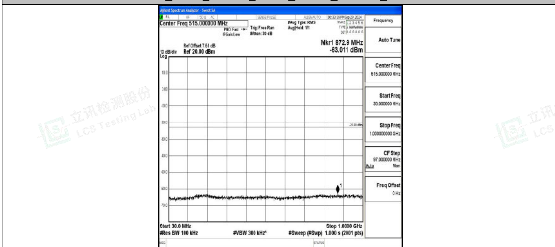
Band2_5MHz_16QAM_18900_1RB#0_30~1000_30~1000
