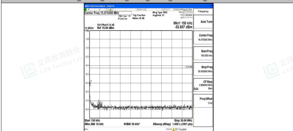
Band2_15MHz_16QAM_19125_1RB#0_0.15~30_0.15~30
