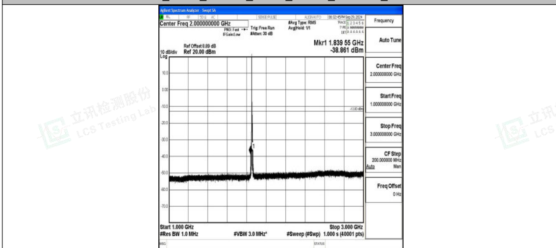
Band2_5MHz_16QAM_18625_1RB#0_1000~3000_1000~3000
