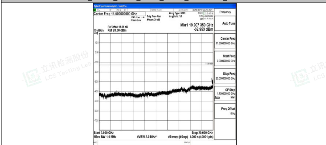
Band2_10MHz_QPSK_18900_1RB#0_3000~20000_3000~20000
