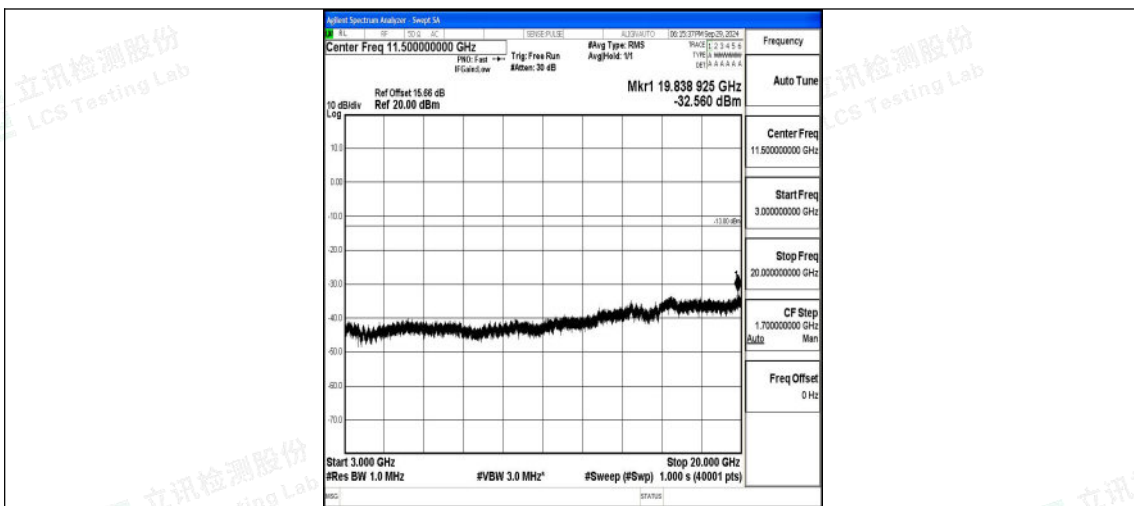
Band2_3MHz_QPSK_19185_1RB#0_3000~20000_3000~20000
