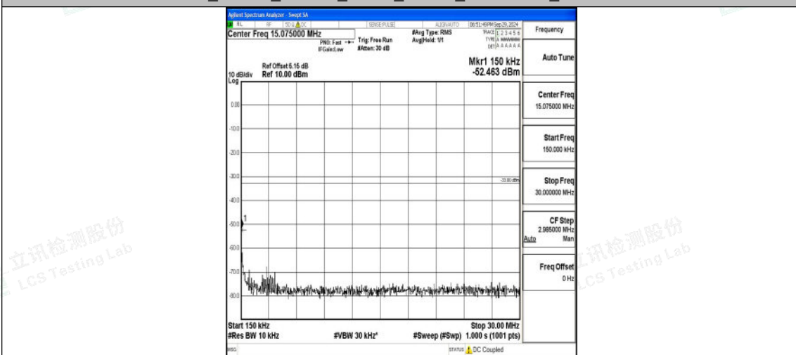
Band2_10MHz_16QAM_18900_1RB#0_0.15~30_0.15~30
