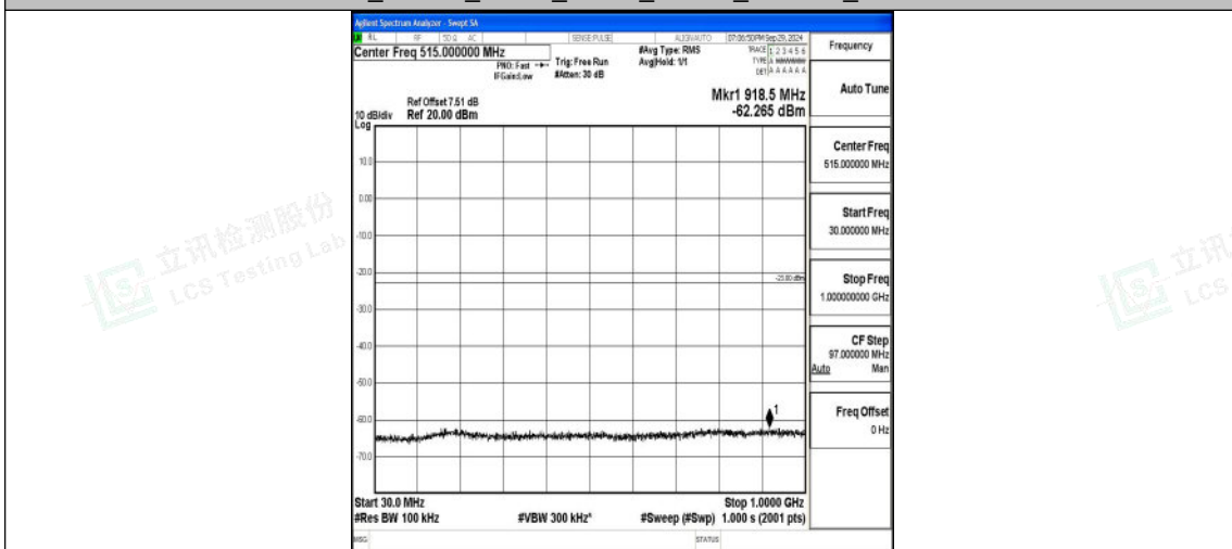
Band2_15MHz_QPSK_18675_1RB#0_30~1000_30~1000
