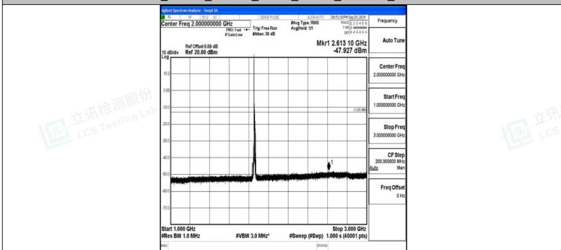
Band2_10MHz_16QAM_18650_1RB#0_1000~3000_1000~3000
