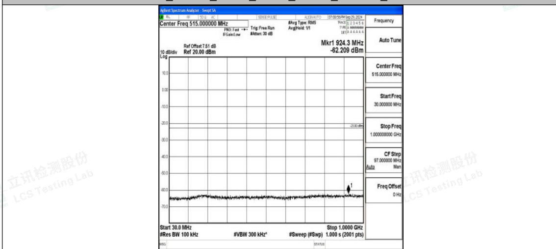
Band2_15MHz_QPSK_19125_1RB#0_30~1000_30~1000
