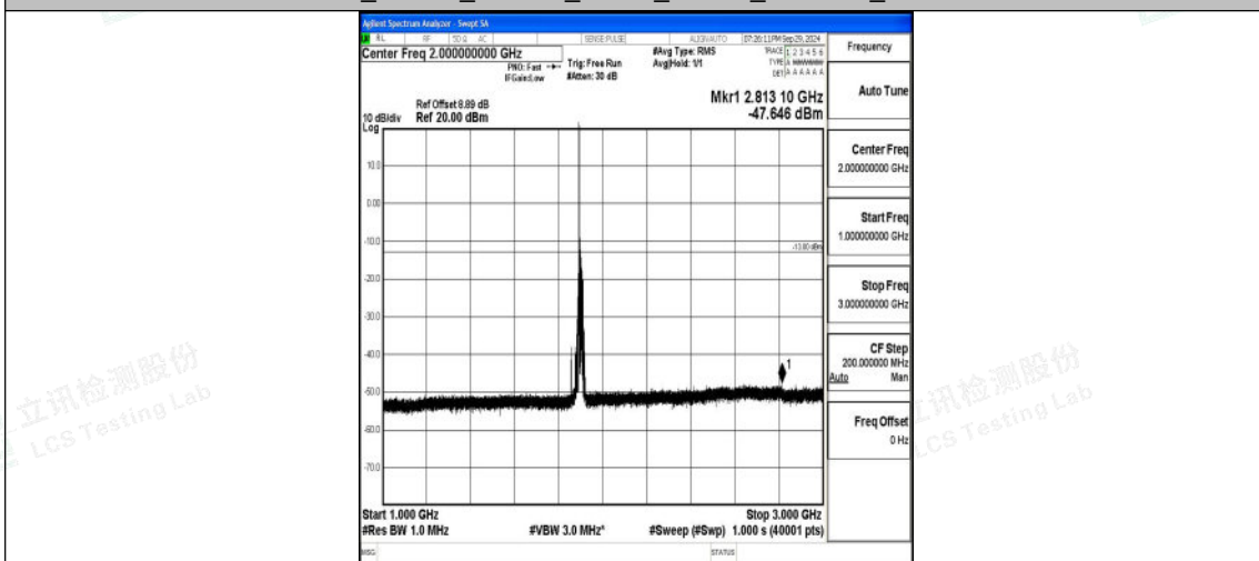
Band2_20MHz_16QAM_19100_1RB#0_1000~3000_1000~3000
