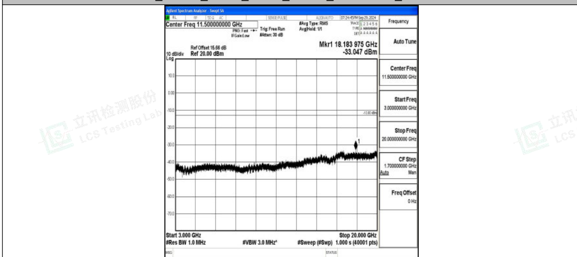
Band2_20MHz_QPSK_18900_1RB#0_3000~20000_3000~20000
