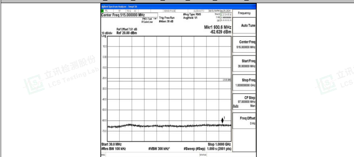
Band2_10MHz_16QAM_18900_1RB#0_30~1000_30~1000
