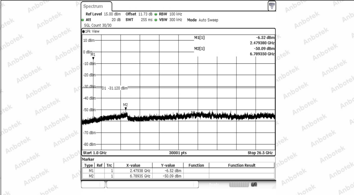
BLE_2M-Ant1-2480-1000~26500-PASS
