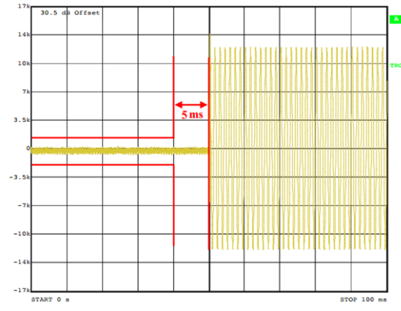
Transmitter Frequency Behavior @ 25 KHz Channel Separation-----On – Off
