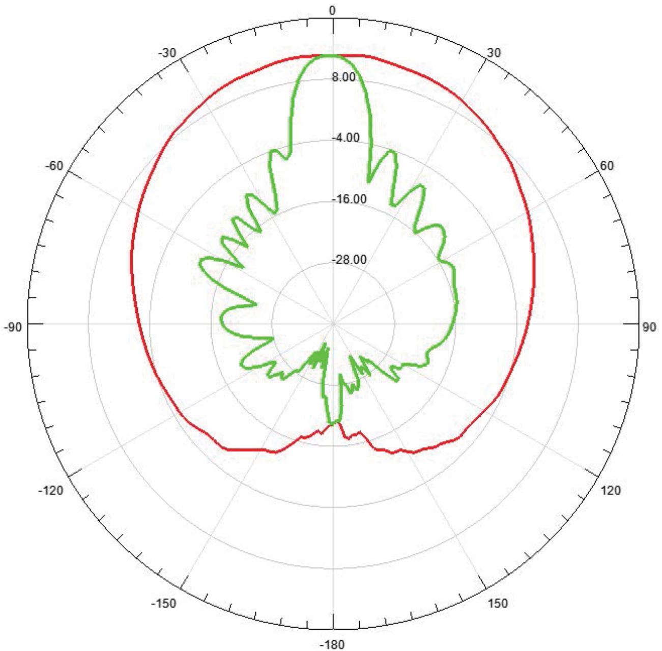
Gain Plot 1
