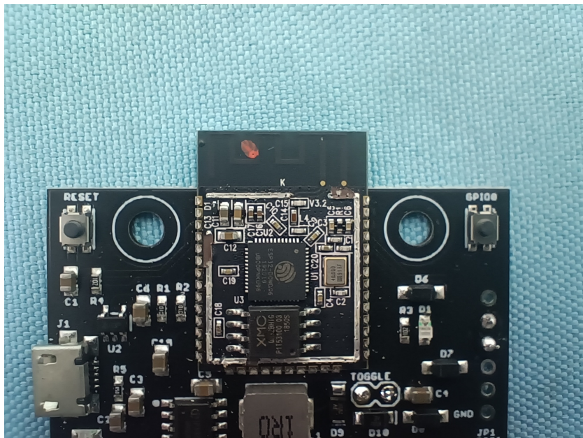
Figure 1: ESP8266 Module
