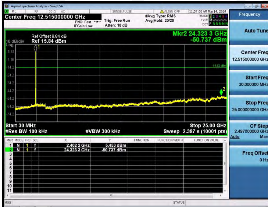
2_Spurious_Emissions_NVNT_ANT1_1-DH1_2402
