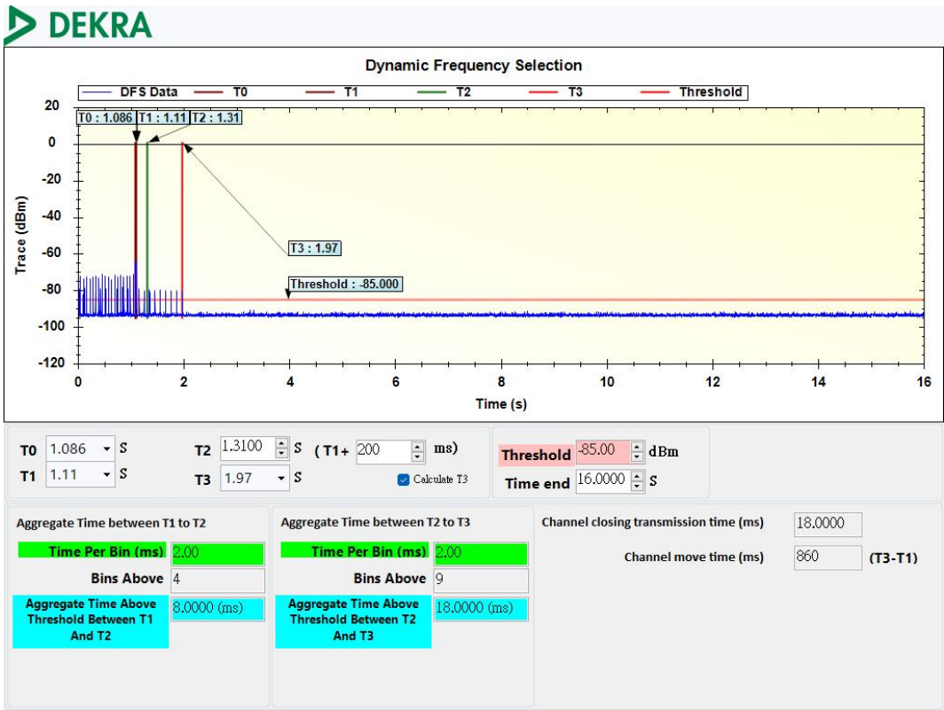
Channel Move Time and Channel Closing Transmission Time - 802.11ax (80 MHz), 5530 MHz
