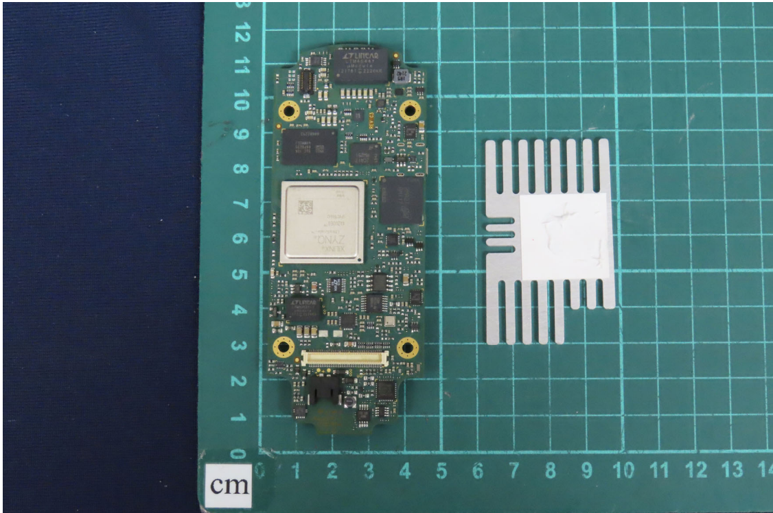
(55) EUT Photo
