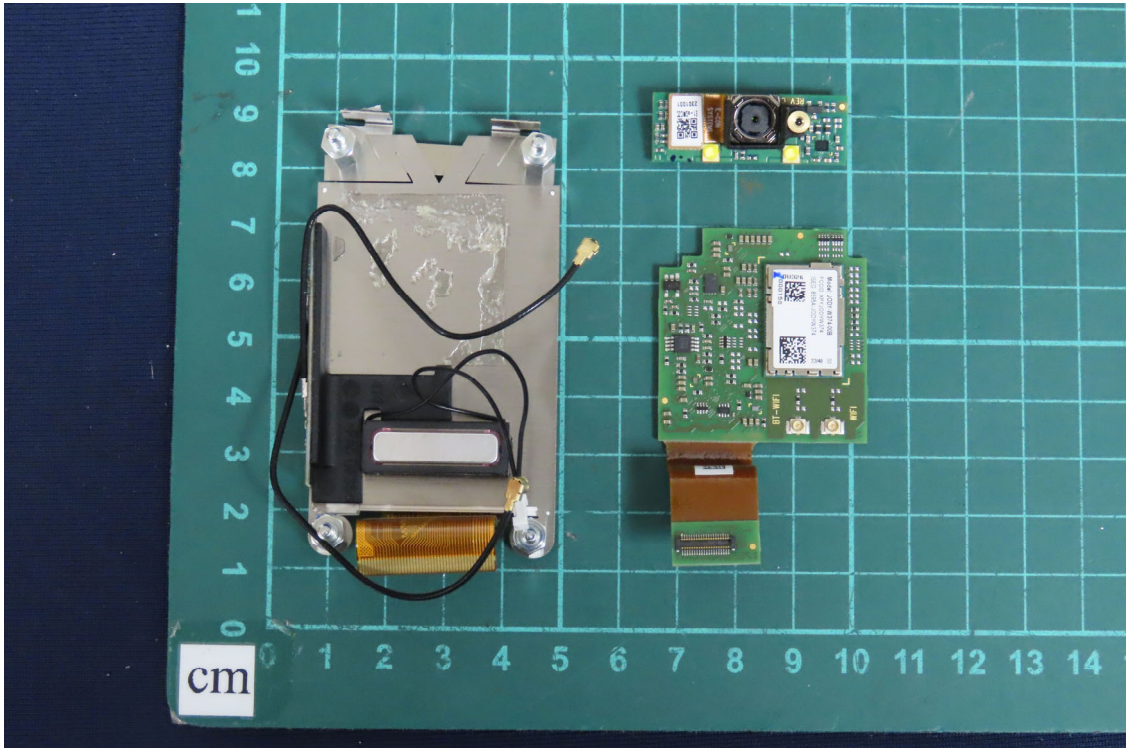
(43) EUT Photo
