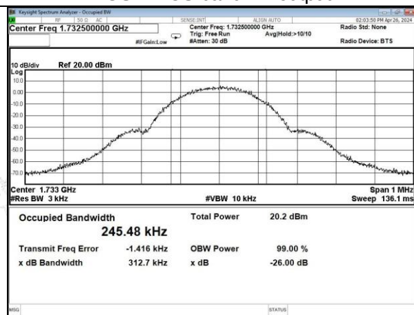
GSM-AWS band UL output
