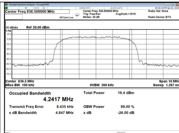
LTE-Cellular band UL output
