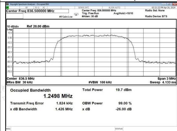
CDMA-Cellular band UL output
