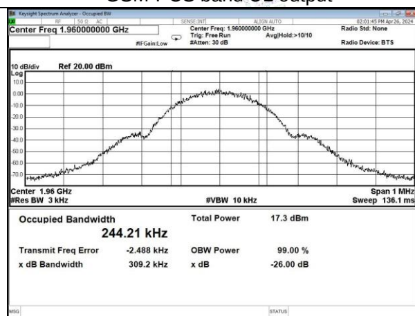
GSM-PCS band DL output
