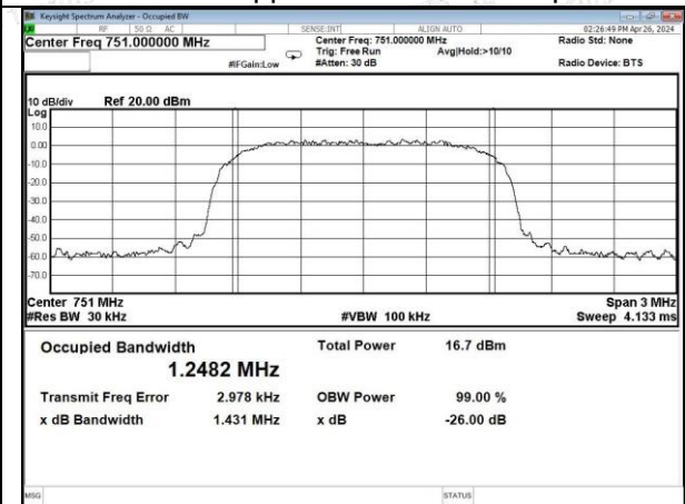
CDMA-Upper 700 band DL output
