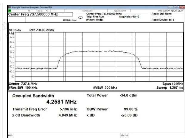
LTE-Lower 700 band DL input
