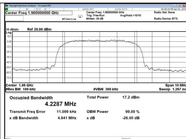
LTE-PCS band DL output
