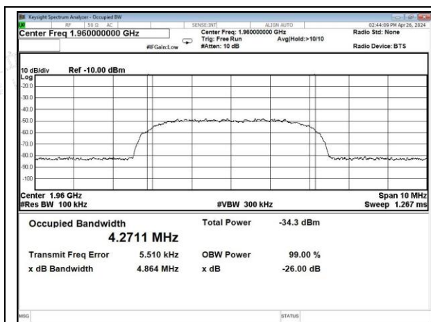
LTE-PCS band DL input
