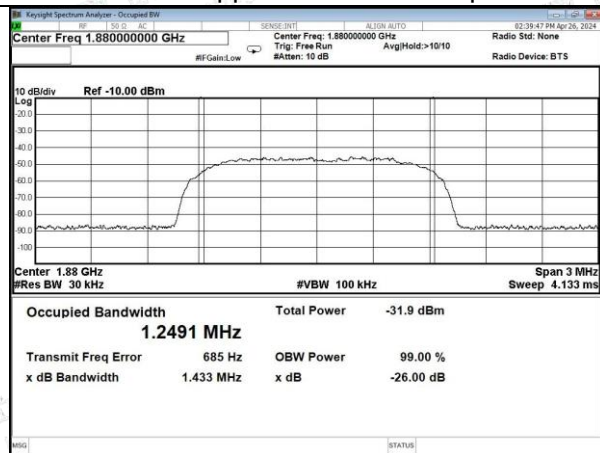
CDMA-PCS band UL input
