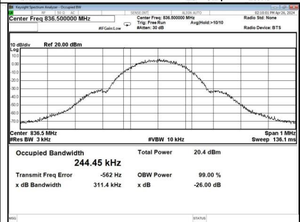
GSM-Cellular band UL output
