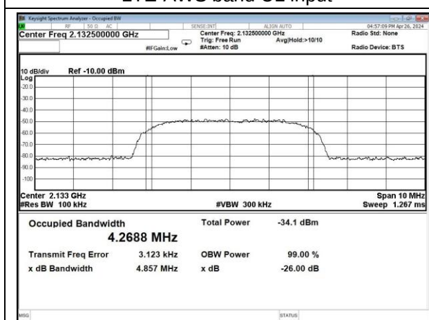
LTE-AWS band DL input
