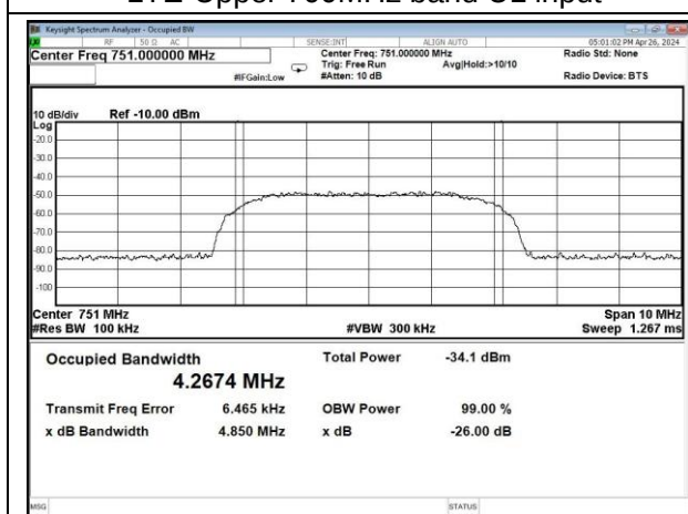
LTE-Upper 700 band DL input
