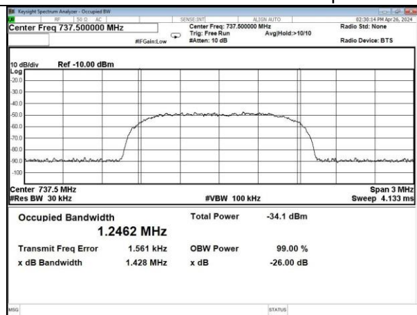
CDMA-Lower 700 band DL input
