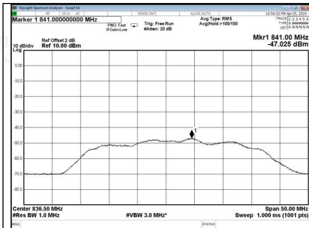
Cellular band UL
