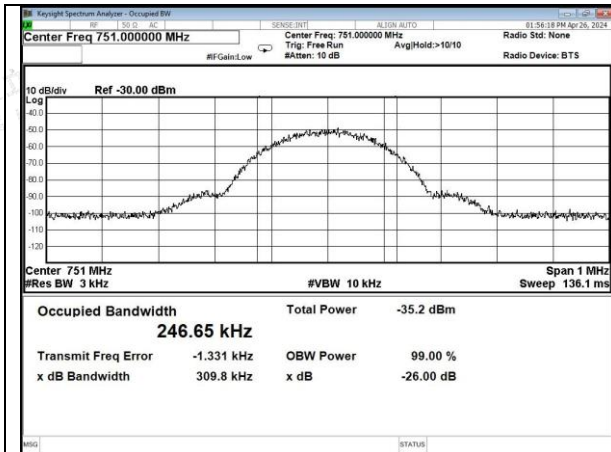
GSM-Upper 700 band DL input
