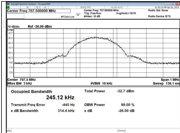
GSM-Lower 700 band UL input
