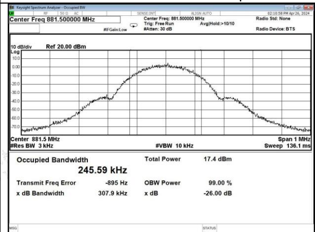
GSM-Cellular band DL output
