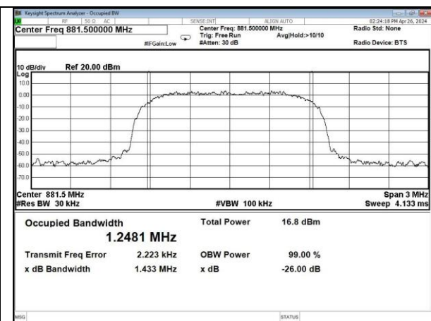
Cellular band DL output
