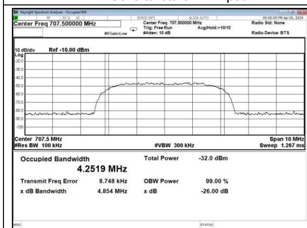
LTE-Lower 700 band UL input
