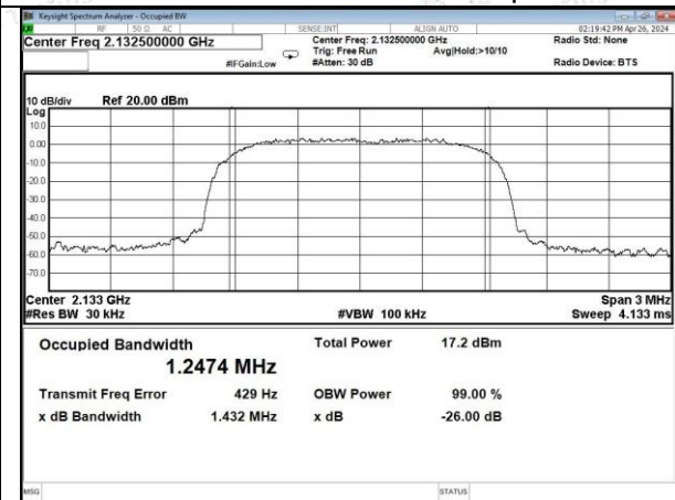
CDMA-AWS band DL output
