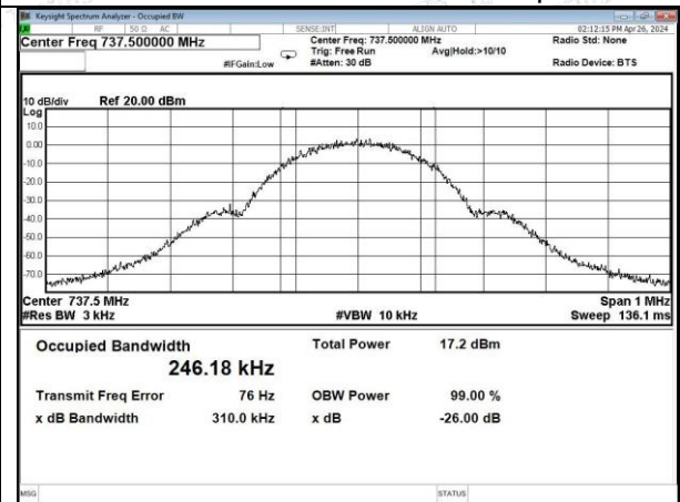
GSM-Lower 700 band DL output
