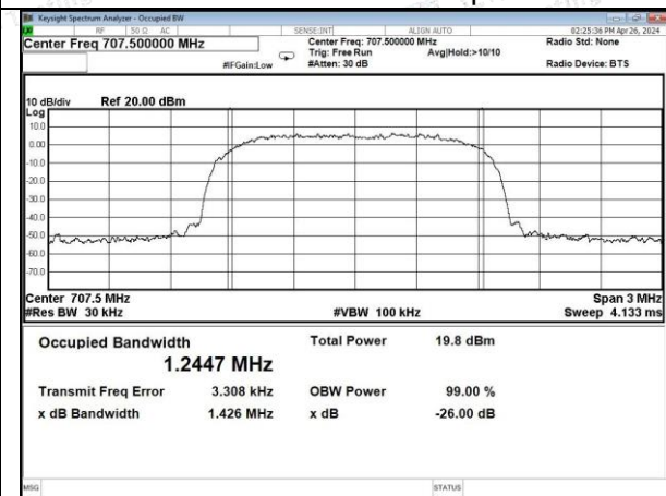
CDMA-Lower 700 band UL output
