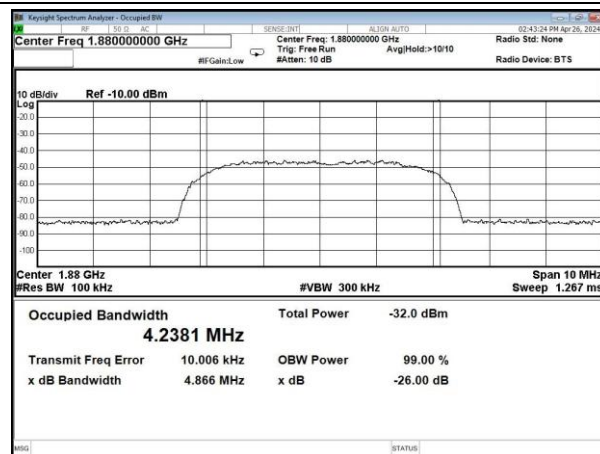
LTE-PCS band UL input
