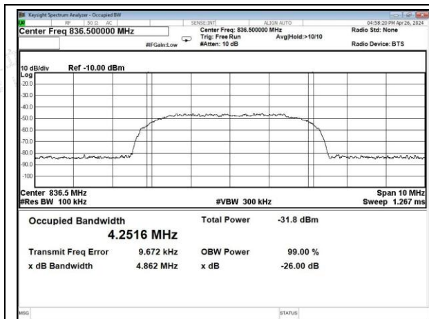
LTE-Cellular band UL input
