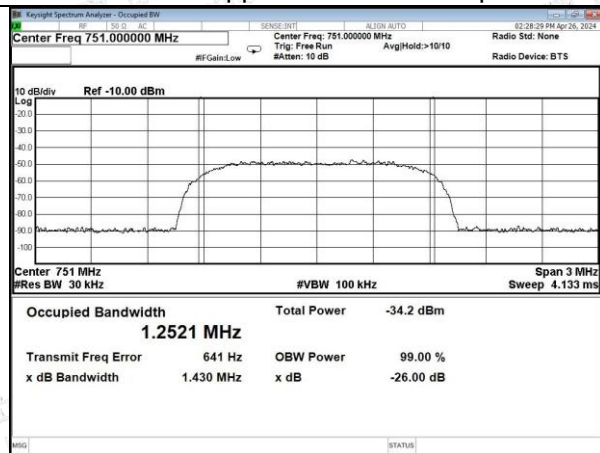
CDMA-Upper 700 band DL input
