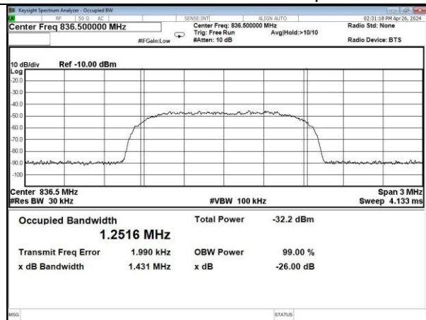
CDMA-Cellular band UL input
