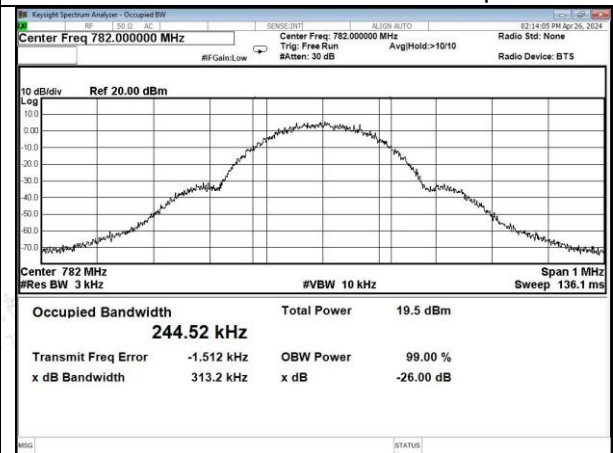
GSM-Upper 700 band UL output
