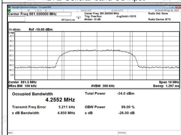
LTE-Cellular band DL input
