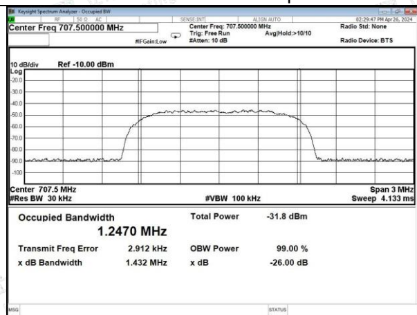
CDMA-Lower 700 band UL input
