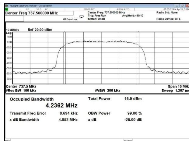
LTE-Lower 700 band DL output
