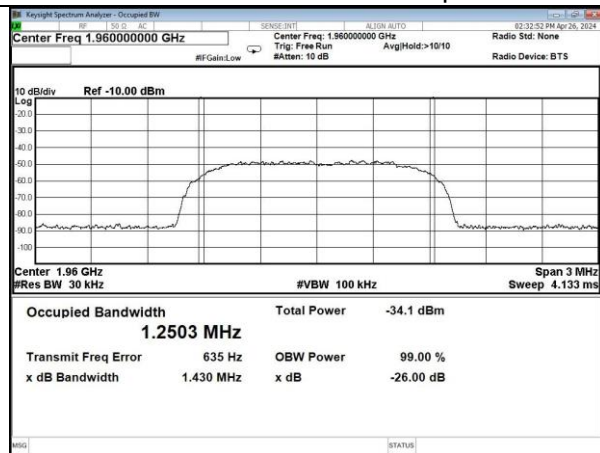
CDMA-PCS band DL input
