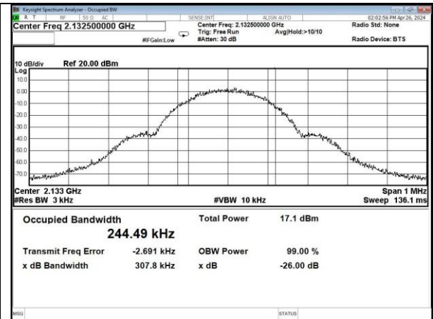
GSM-AWS band DL output
