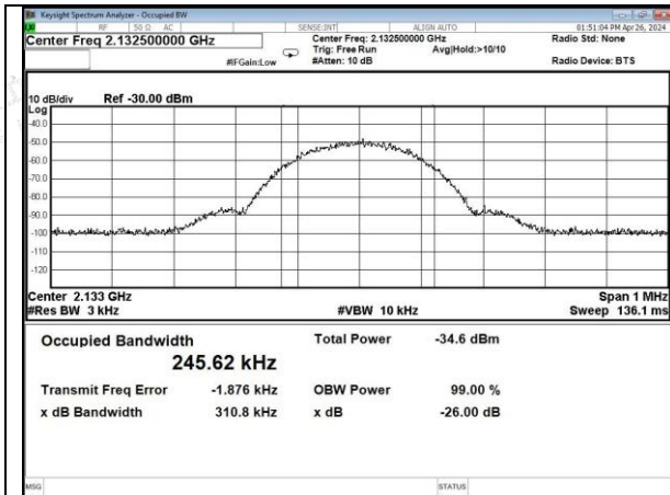
GSM-AWS band DL input
