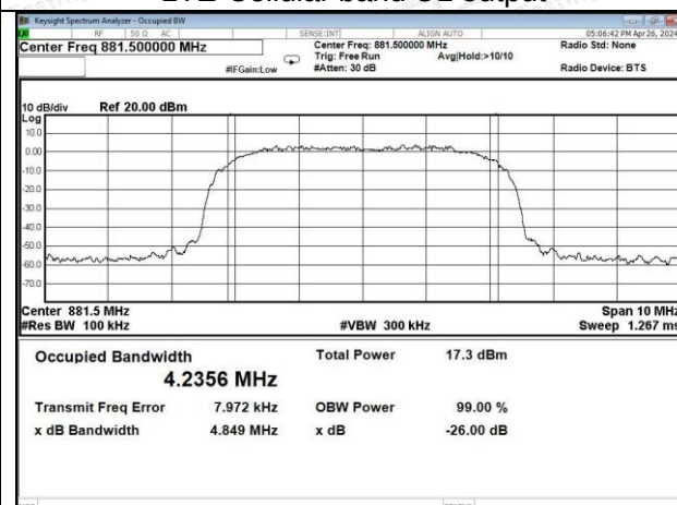
LTE-Cellular band DL output
