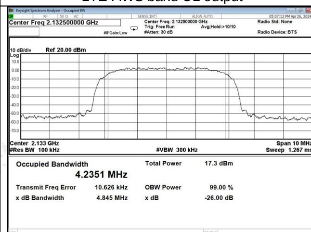
LTE-AWS band DL output
