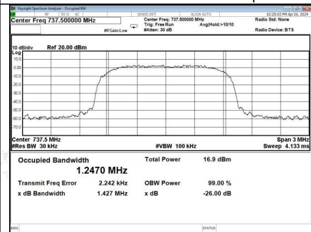
CDMA-Lower 700 band DL output
