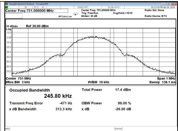
GSM-Upper 700 band DL output
