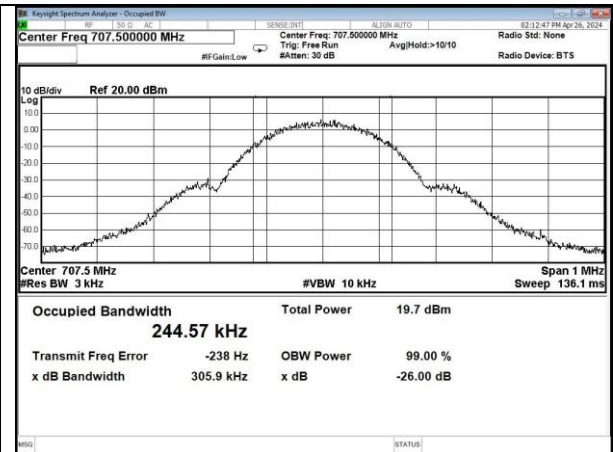
GSM-Lower 700 band UL output
