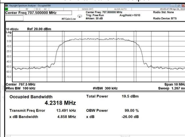
LTE-Lower 700 band UL output
