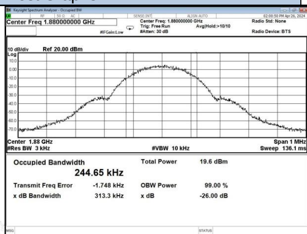
GSM-PCS band UL output
