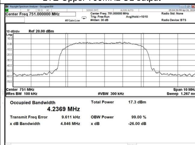
LTE-Upper 700 band DL output
