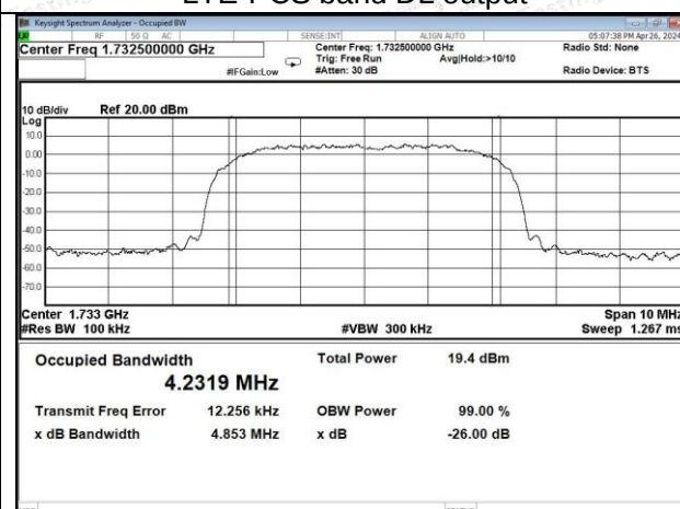
LTE-AWS band UL output
