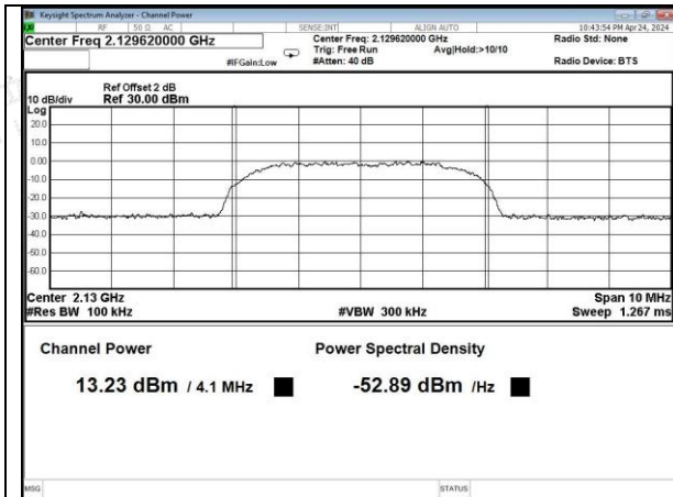
AWS Band AWGN, DL
