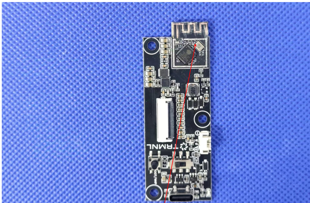
PCB antenna
