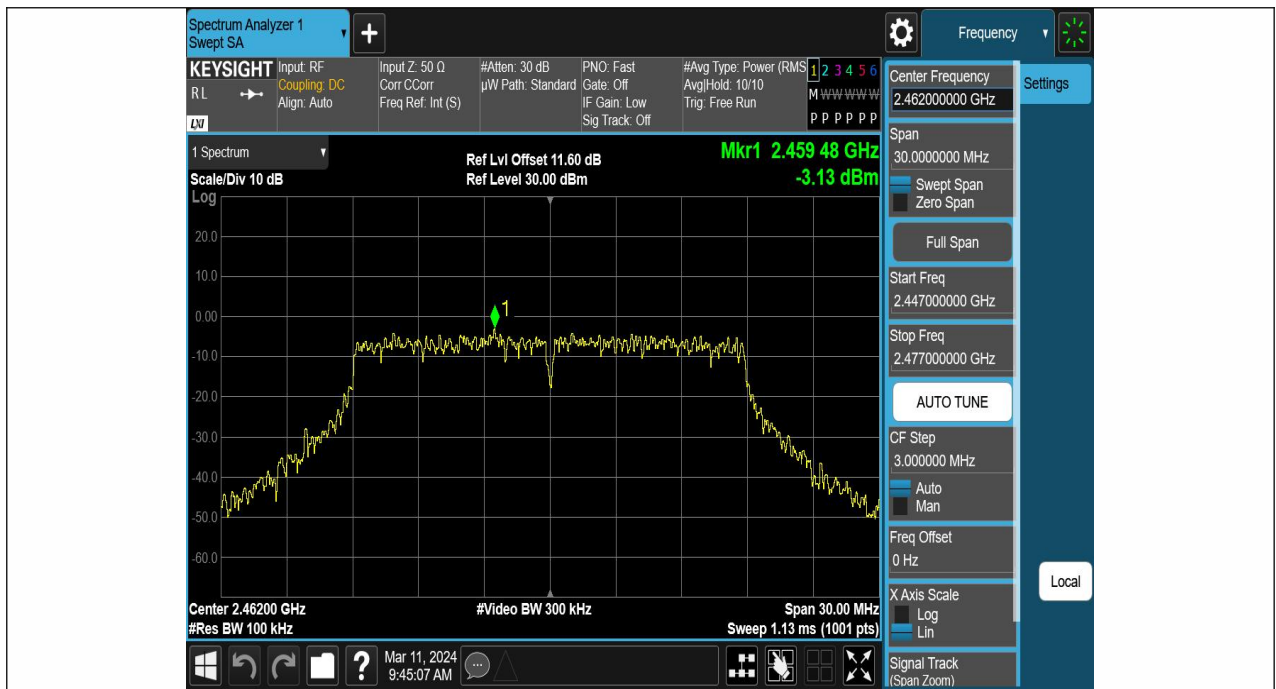
11N20SISO-Ant1-2462-0~Reference-PASS
