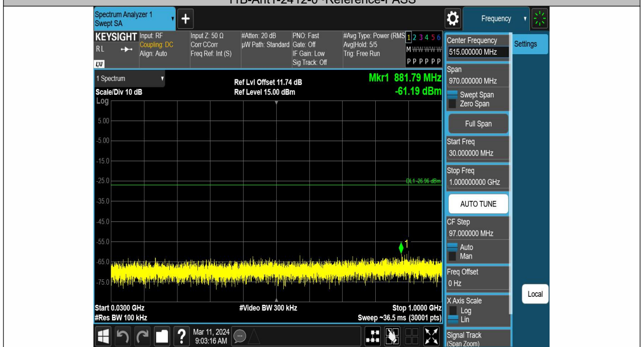
11B-Ant1-2412-30~1000-PASS
