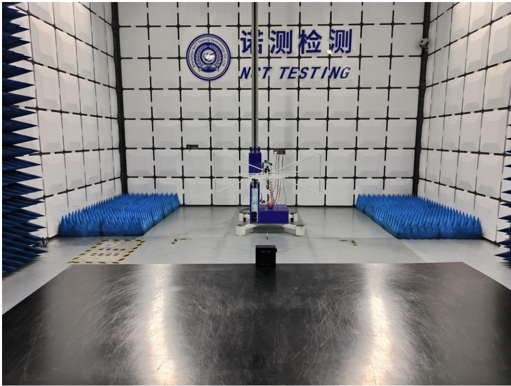
Setup Photo FCC ID: 2BFVI-BT2972
