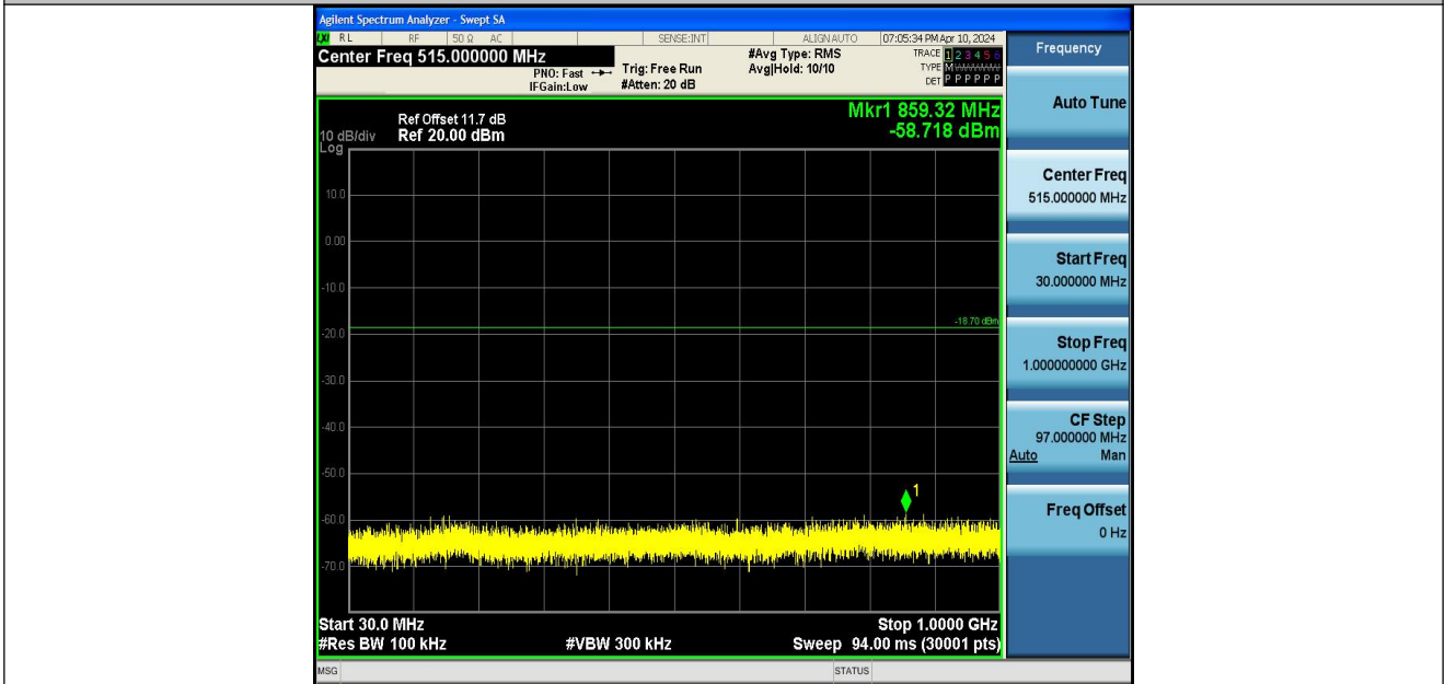
BLE_1M-Ant1-2480-30~1000-PASS
