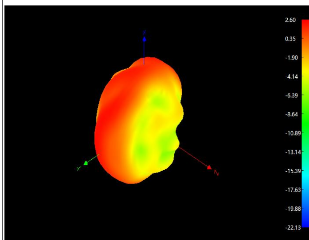
WIF/BT1: 2420Mhz
