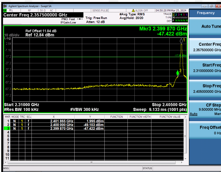
2_Bandedge_NVNT_ANT1_1-DH1_2402
