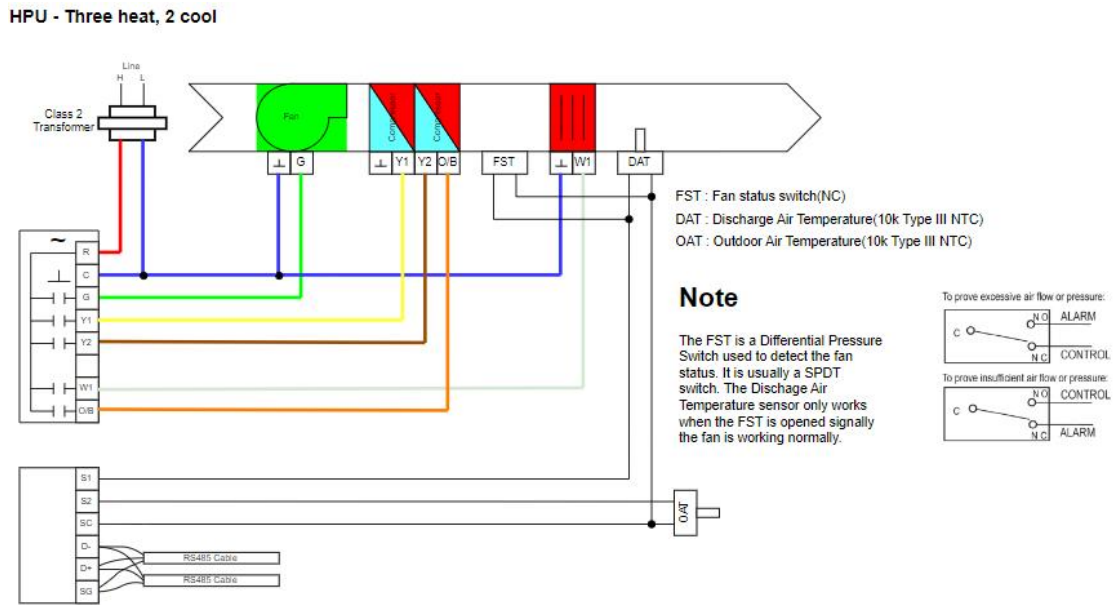
FIGURE 15: HEAT PUMP APPLICATION
