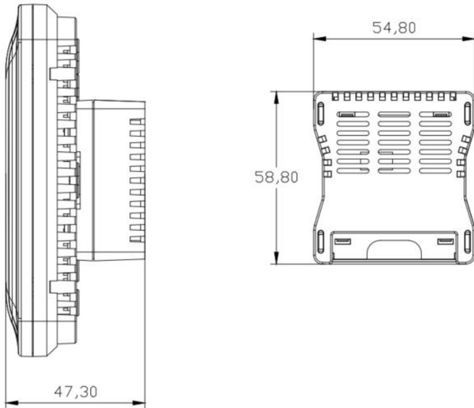
FIGURE 3: MT-5-X/L DIMENSION
