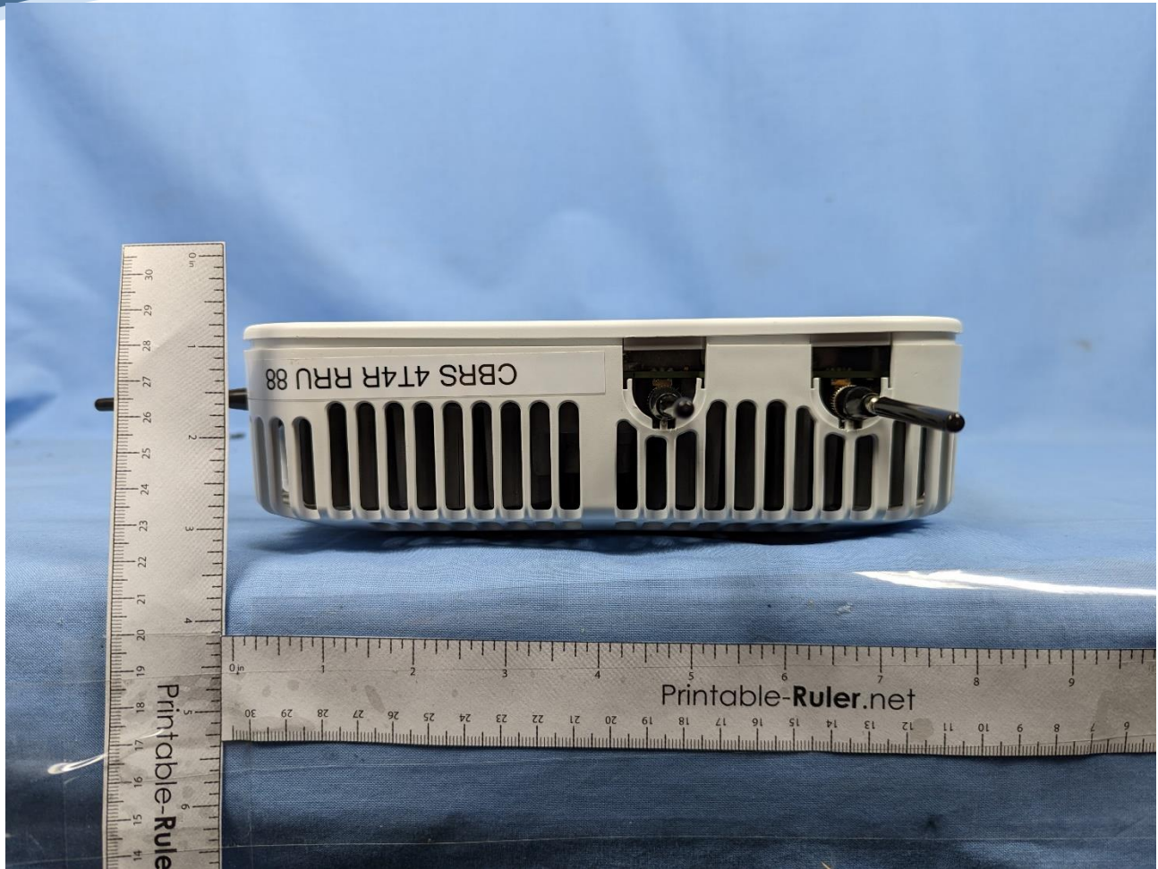
Left View
