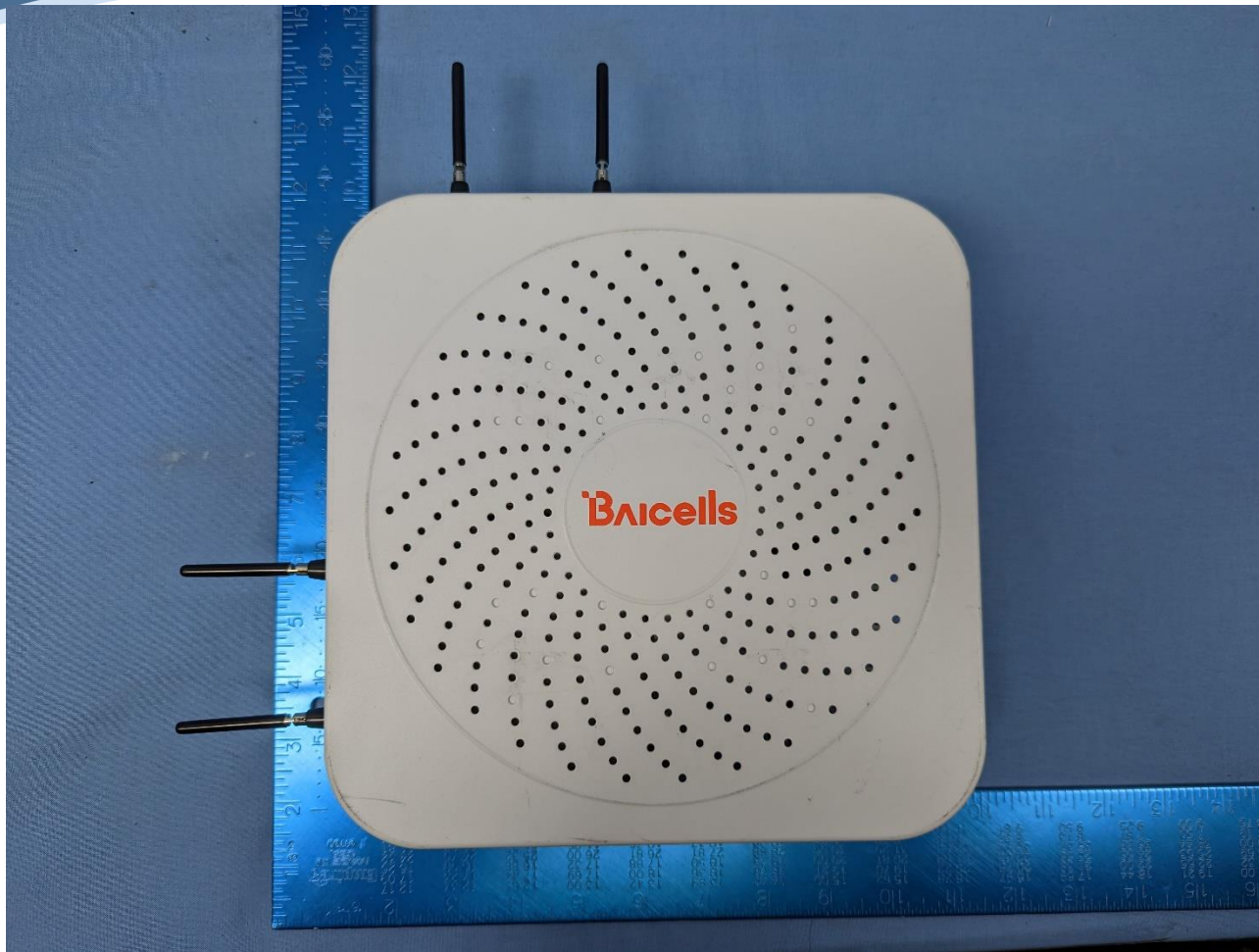
Front View
