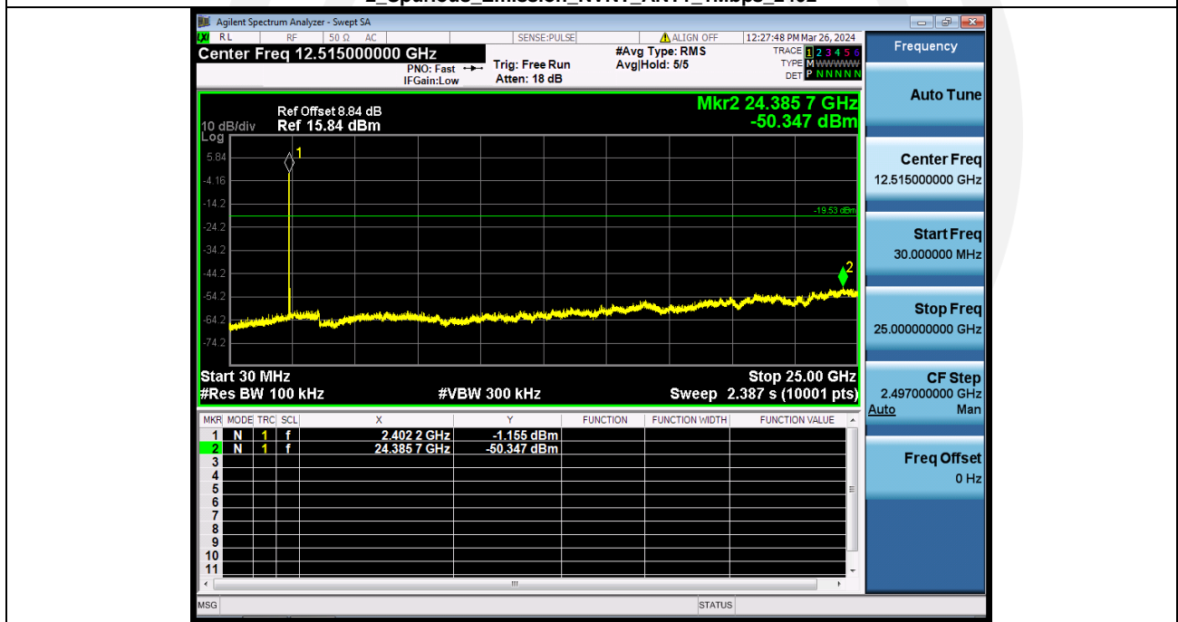
2_Spurious_Emission_NVNT_ANT1_1Mbps_2402
