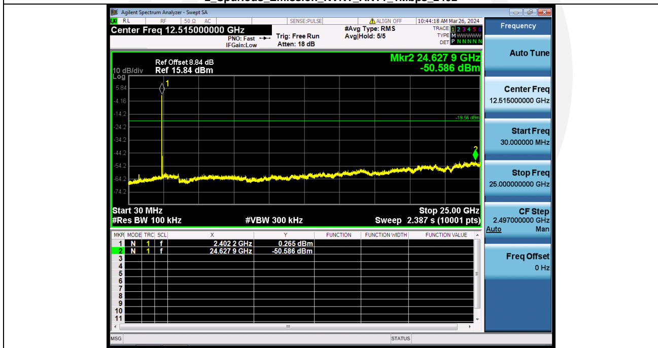
2_Spurious_Emission_NVNT_ANT1_1Mbps_2402
