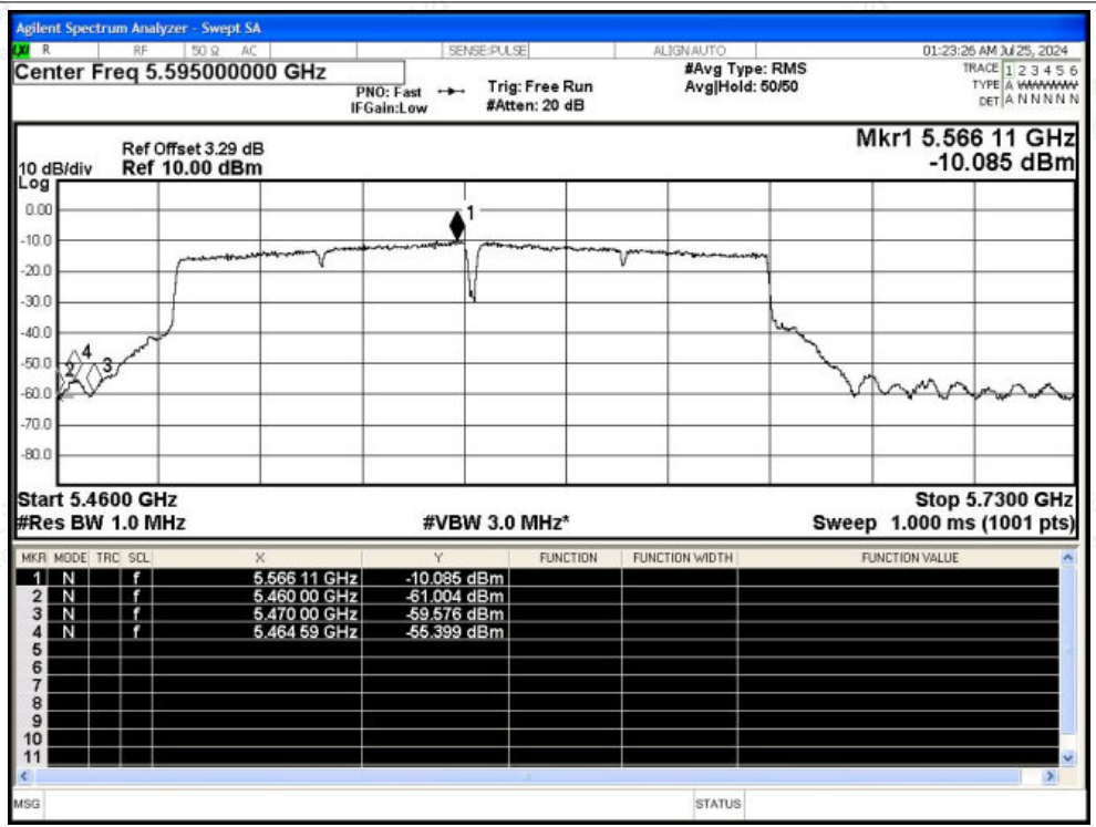
Restrict Band NVNT ax160 5570MHz Ant2 Peak
