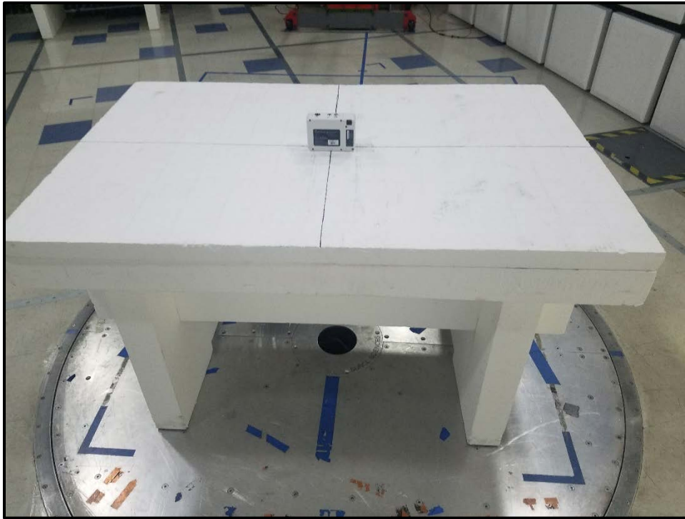
Radiated Emissions-1
