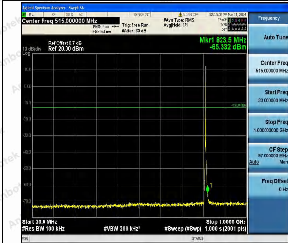
Band26_3MHz_QPSK_26705_1RB#0_30~1000_30~1000
