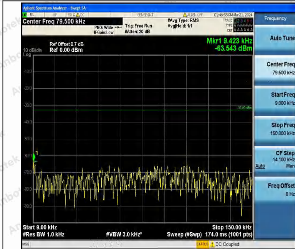
Band26_3MHz_QPSK_27025_1RB#0_0.009~0.15_0.009~0.15
