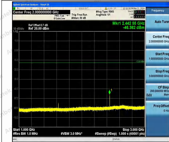
Band26_3MHz_16QAM_26705_1RB#0_1000~3000_1000~3000
