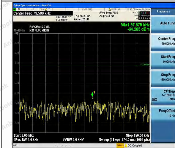
Band26_3MHz_QPSK_26740_1RB#0_0.009~0.15_0.09~0.15
