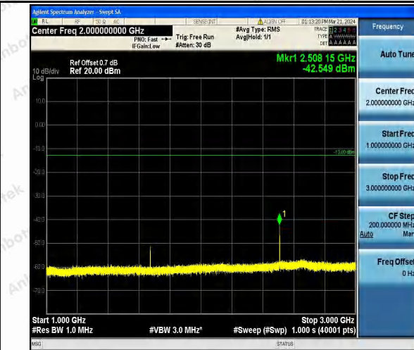
Band26_1.4MHz_QPSK_26915_1RB#0_1000~3000_1000~3000
