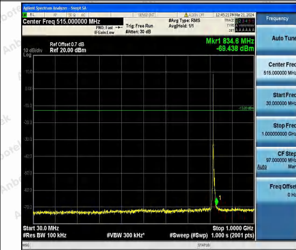
Band26_5MHz_16QAM_26765_1RB#0_30~1000_30~1000 000
