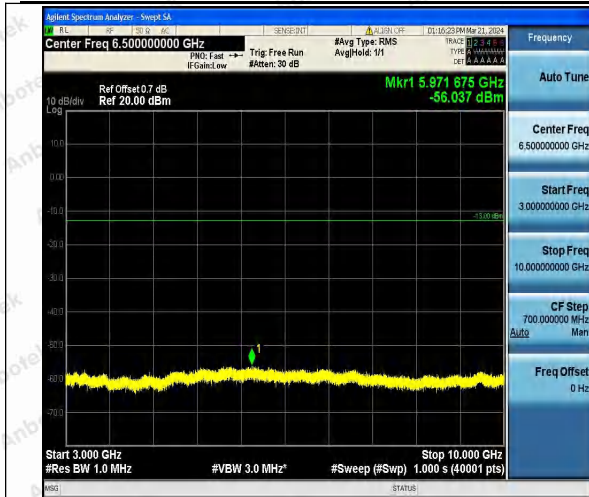
Band26_1.4MHz_QPSK_27033_1RB#0_3000~10000_3000~10000
