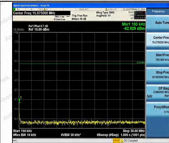
Band26_1.4MHz_QPSK_26797_1RB#0_0.15~30_0.15~30
