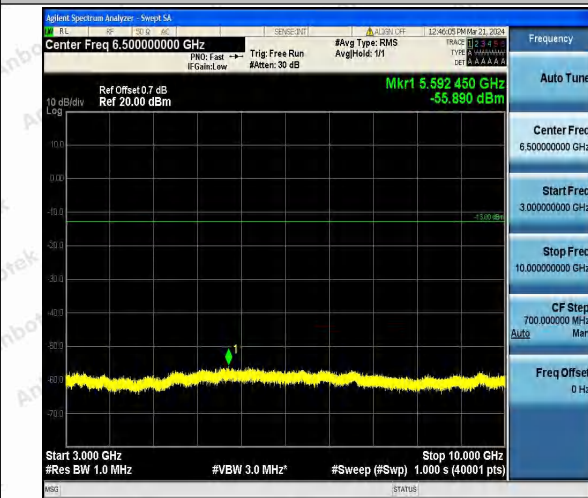
Band26_5MHz_16QAM_26765_1RB#0_3000~10000_3000~10000 000~10000
