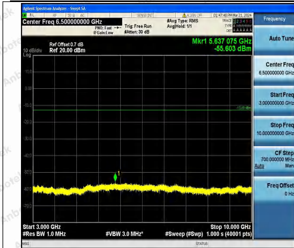
Band26_3MHz_QPSK_27025_1RB#0_3000~10000_3000~10000
