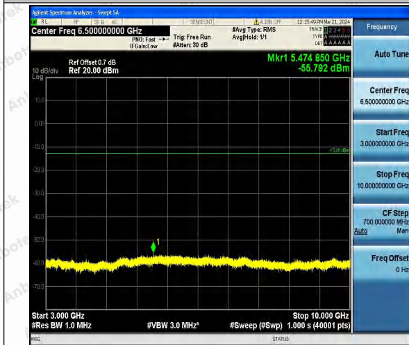
Band26_3MHz_QPSK_26705_1RB#0_3000~10000_3000~10000
