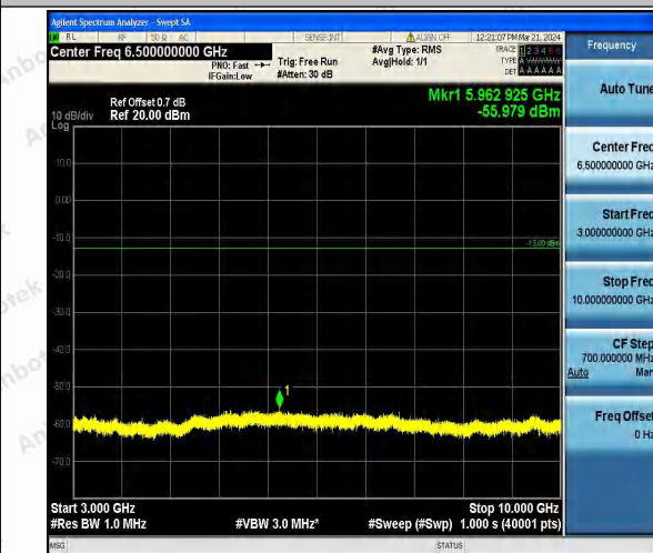
Band26_3MHz_16QAM_26775_1RB#0_3000~10000_3 000~10000
