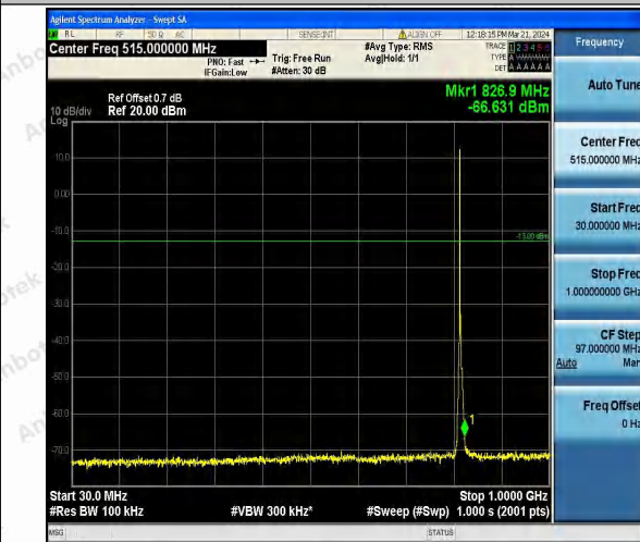
Band26_3MHz_16QAM_26740_1RB#0_30~1000_30~1000
