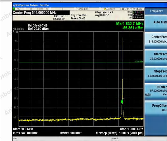
Band26_1.4MHz_16QAM_26915_1RB#0_30~1000_30~1000
