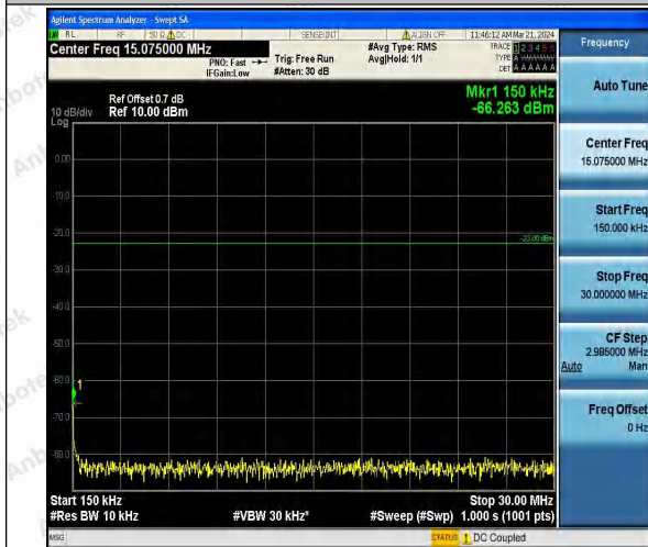
Band26_1.4MHz_16QAM_26740_1RB#0_0.15~30_0.15~30
