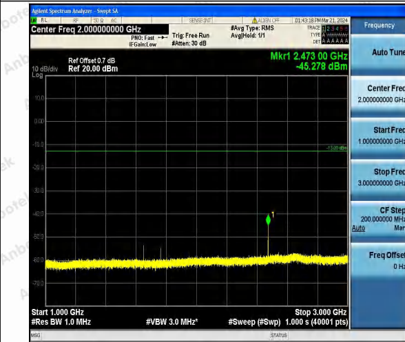
Band26_3MHz_QPSK_26805_1RB#0_1000~3000_1000~3000
