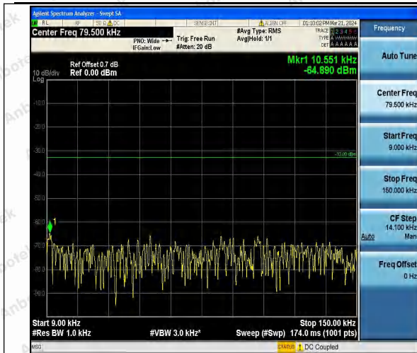
Band26_1.4MHz_QPSK_26797_1RB#0_0.009~0.15_0.009~0.15
