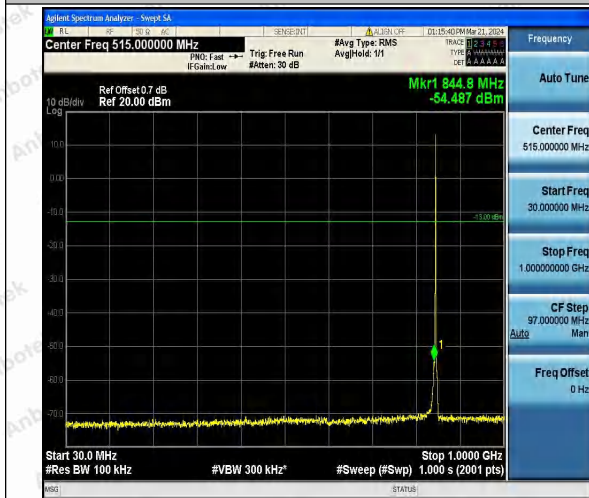
Band26_1.4MHz_QPSK_27033_1RB#0_30~1000_30~1000
