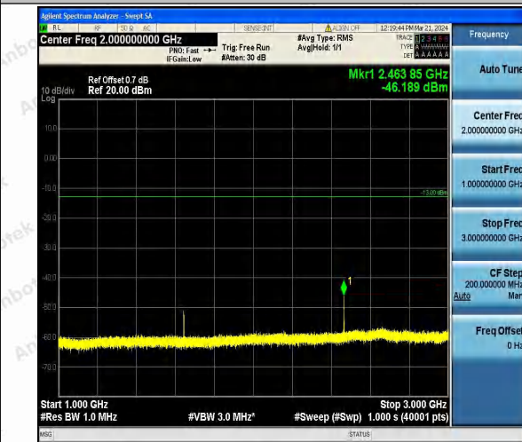
Band26_3MHz_QPSK_26775_1RB#0_1000~3000_1000~3000
