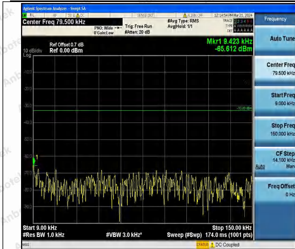
Band26_3MHz_QPSK_26705_1RB#0_0.009~0.15_0.0 09~0.15
