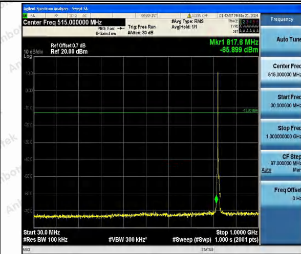
Band26_3MHz_16QAM_26805_1RB#0_30~1000_30~1000
