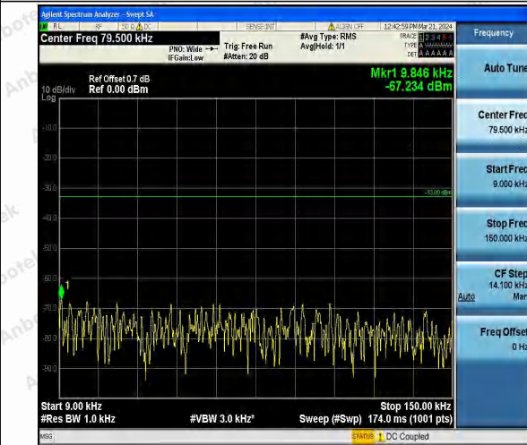
Band26_5MHz_16QAM_26740_1RB#0_0.009~0.15_0.09~0.15
