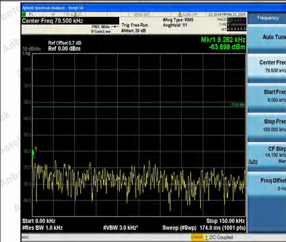
Band26_3MHz_16QAM_26740_1RB#0_0.009~0.15_0.09~0.15
