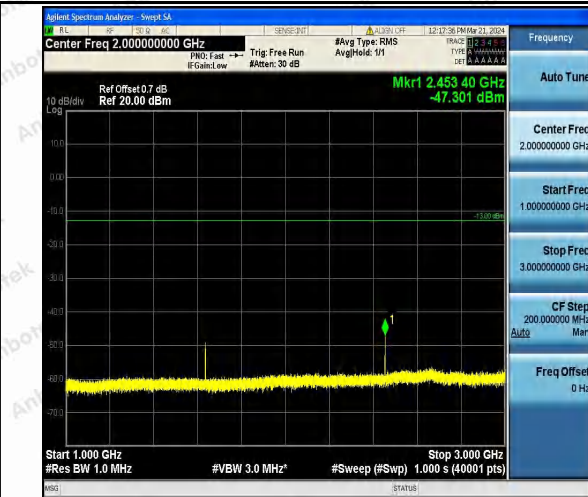
Band26_3MHz_QPSK_26740_1RB#0_1000~3000_1000~3000
