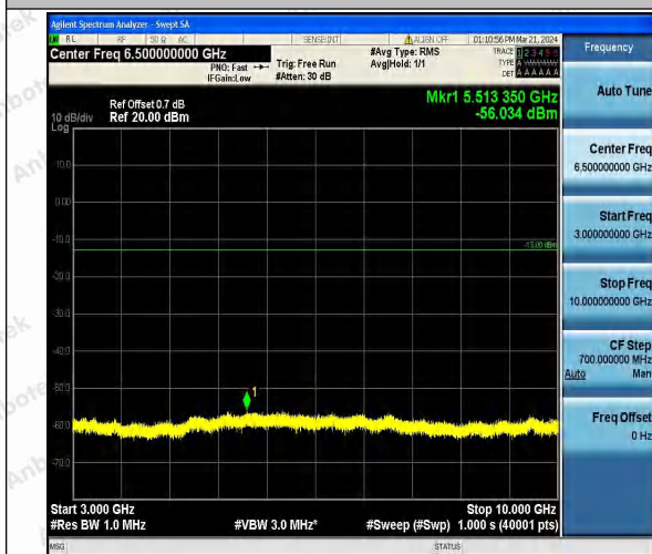
Band26_1.4MHz_QPSK_26797_1RB#0_3000~10000_3000~10000
