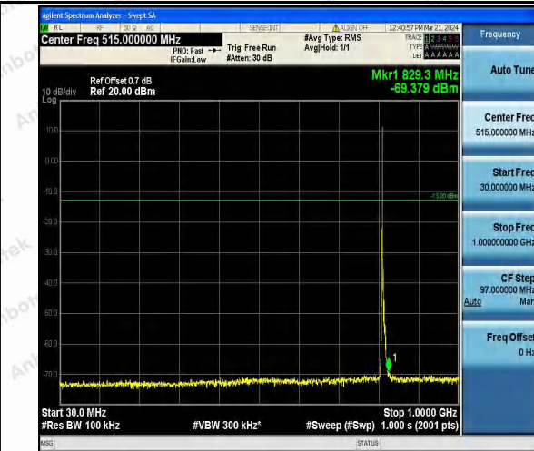
Band26_5MHz_16QAM_26715_1RB#0_30~1000_30~1000
