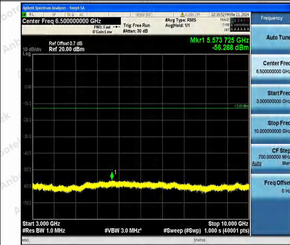
Band26_3MHz_16QAM_26705_1RB#0_3000~10000_3000~10000
