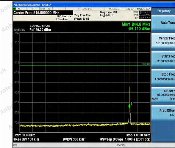
Band26_1.4MHz_16QAM_27033_1RB#0_30~1000_30~1000
