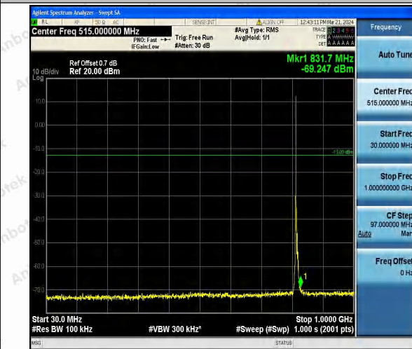
Band26_5MHz_16QAM_26740_1RB#0_30~1000_30~1000
