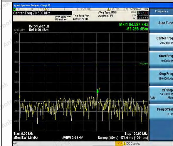
Band26_1.4MHz_QPSK_26915_1RB#0_0.009~0.15_0.09~0.15 009~0.15
