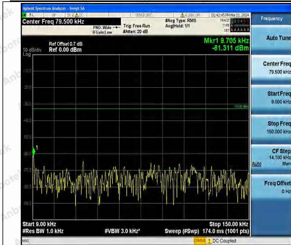
Band26_3MHz_QPSK_26805_1RB#0_0.009~0.15_0.0 09~0.15
