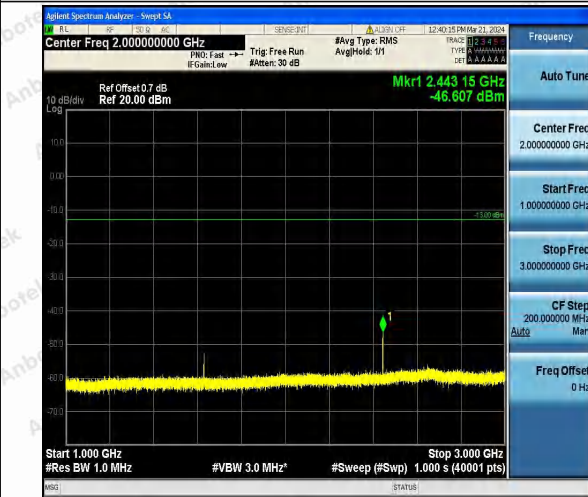
Band26_5MHz_QPSK_26715_1RB#0_1000~3000_1000~3000
