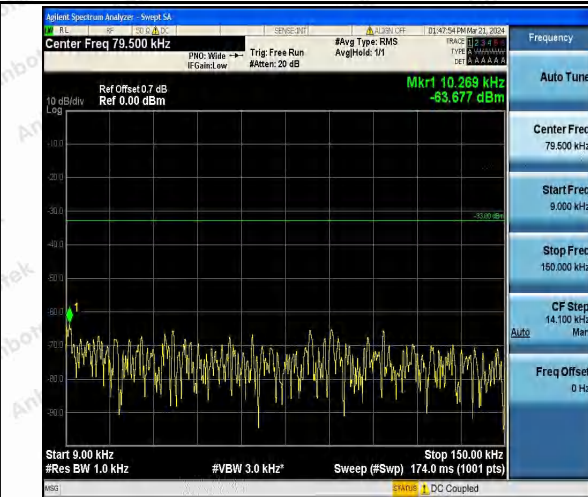
Band26_3MHz_16QAM_27025_1RB#0_0.009~0.15_0.09~0.15
