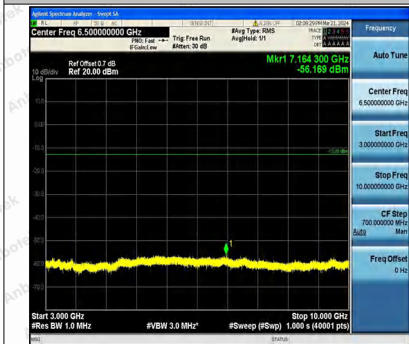
Band26_5MHz_QPSK_26815_1RB#0_3000~10000_3000~10000
