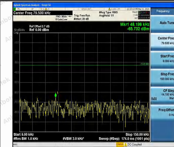
Band26_3MHz_16QAM_26775_1RB#0_0.009~0.15_0.0 09~0.15
