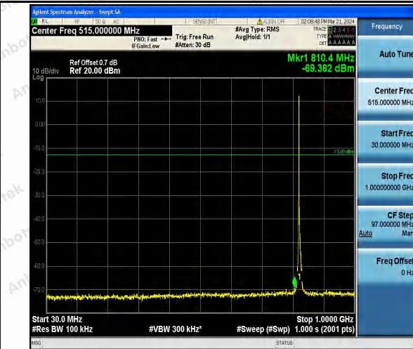
Band26_5MHz_16QAM_26815_1RB#0_30~1000_30~1000
