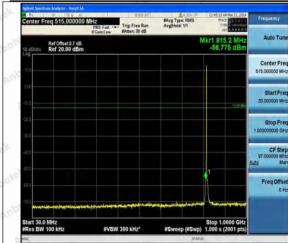
Band26_1.4MHz_QPSK_26740_1RB#0_30~1000_30~1000
