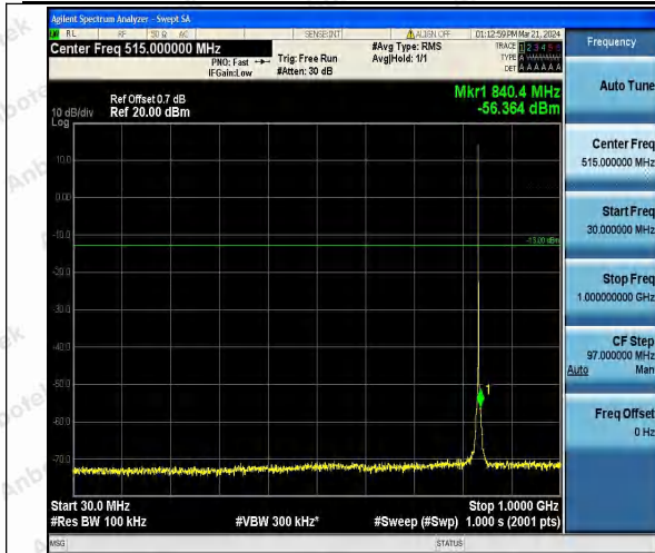
Band26_1.4MHz_QPSK_26915_1RB#0_30~1000_30~1000
