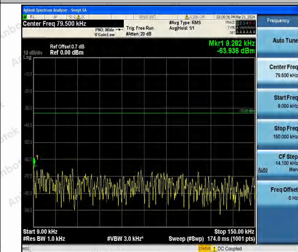
Band26_5MHz_16QAM_26815_1RB#0_0.009~0.15_0.0
