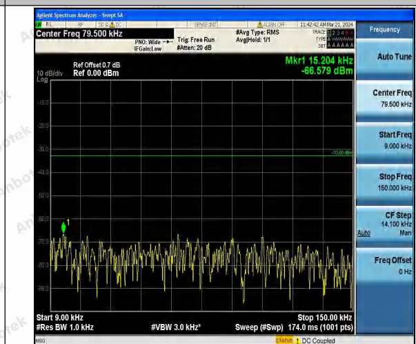
Band26_1.4MHz_16QAM_26697_1RB#0_0.009~0.15_0.009~0.15
