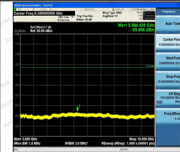
Band26_1.4MHz_16QAM_26740_1RB#0_3000~10000_3000~10000
