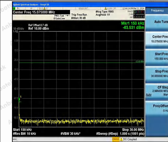
Band26_5MHz_QPSK_26765_1RB#0_0.15~30_0.15~30
