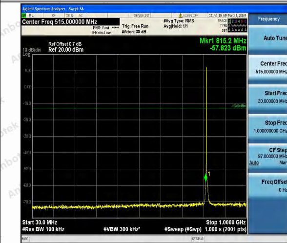
Band26_1.4MHz_16QAM_26740_1RB#0_30~1000_30~1000
