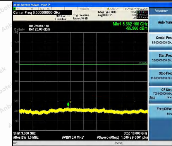
Band26_3MHz_16QAM_26805_1RB#0_3000~10000_3000~10000
