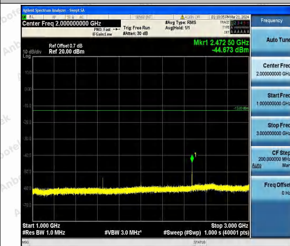
Band26_1.4MHz_QPSK_26797_1RB#0_1000~3000_1000~3000
