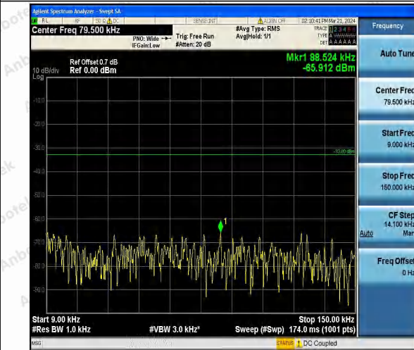
Band26_5MHz_16QAM_26915_1RB#0_0.009~0.15_0.09~0.15
