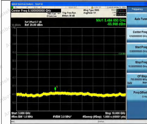
Band26_1.4MHz_QPSK_26740_1RB#0_3000~10000_3000~10000
