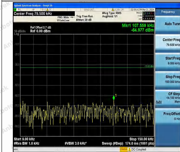
Band26_5MHz_QPSK_26915_1RB#0_0.009~0.15_0.09~0.15
