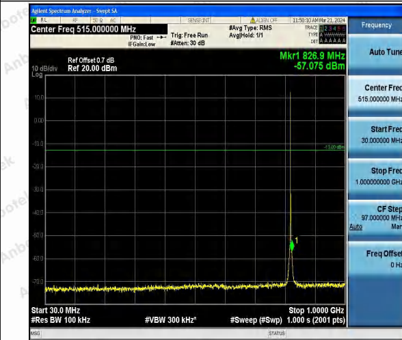
Band26_1.4MHz_16QAM_26783_1RB#0_30~1000_30~1000
