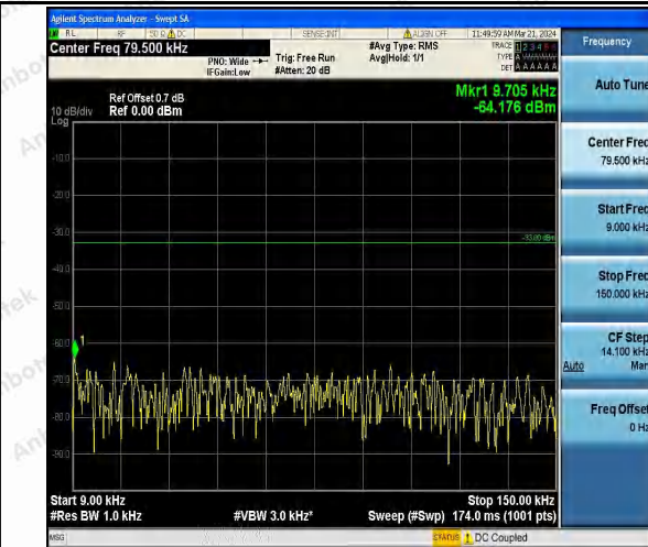
Band26_1.4MHz_16QAM_26783_1RB#0_0.009~0.15_0.009~0.15
