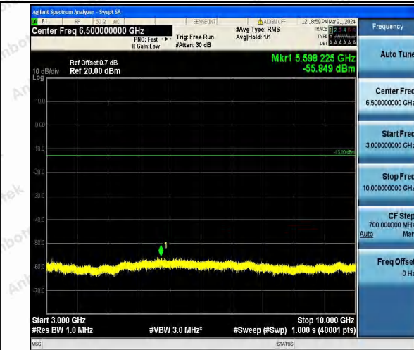
Band26_3MHz_16QAM_26740_1RB#0_3000~10000_3000~10000
