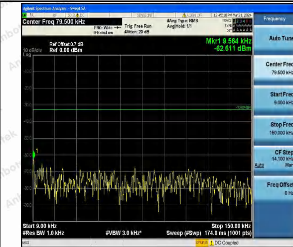
Band26_5MHz_16QAM_26765_1RB#0_0.009~0.15_0.0 09~0.15
