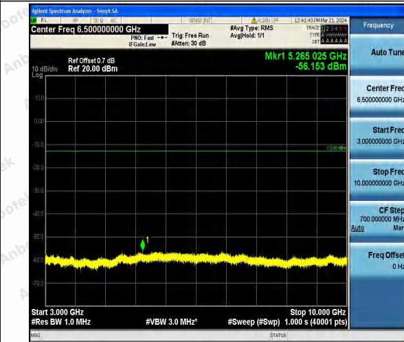
Band26_5MHz_16QAM_26715_1RB#0_3000~10000_3000~10000
