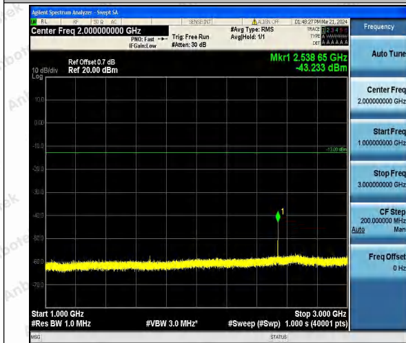
Band26_3MHz_16QAM_27025_1RB#0_1000~3000_1000~3000
