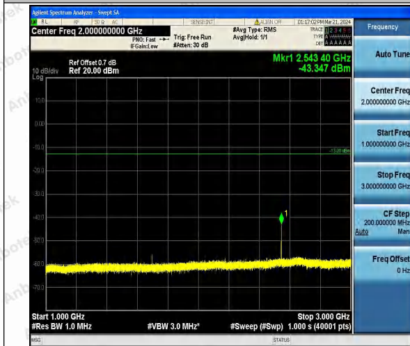
Band26_1.4MHz_16QAM_27033_1RB#0_1000~3000_1000~3000
