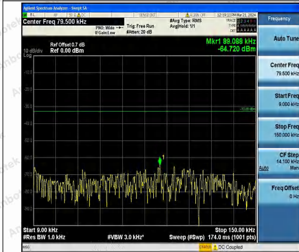
Band26_3MHz_QPSK_26775_1RB#0_0.009~0.15_0.09~0.15
