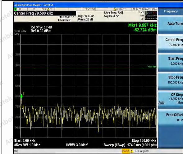
Band26_5MHz_QPSK_26765_1RB#0_0.009~0.15_0.09~0.15
