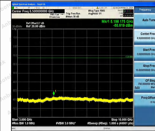
Band26_5MHz_16QAM_26815_1RB#0_3000~10000_3000~10000
