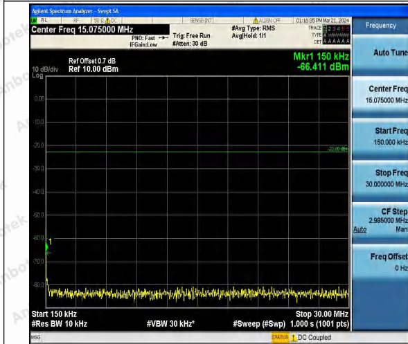
Band26_1.4MHz_16QAM_27033_1RB#0_0.15~30_0.15~30
