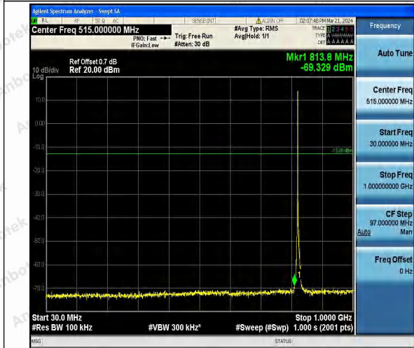
Band26_5MHz_QPSK_26815_1RB#0_30~1000_30~1000
