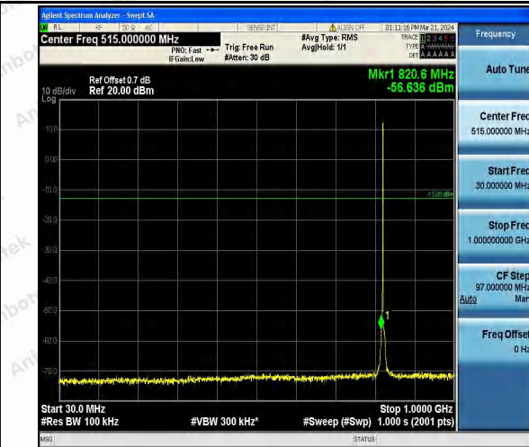
Band26_1.4MHz_16QAM_26797_1RB#0_30~1000_30~1000 1000
