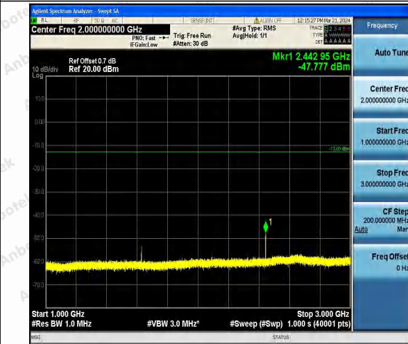
Band26_3MHz_QPSK_26705_1RB#0_1000~3000_1000~3000
