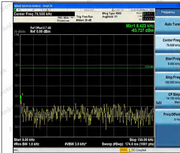
Band26_1.4MHz_QPSK_26697_1RB#0_0.009~0.15_0.009~0.15
