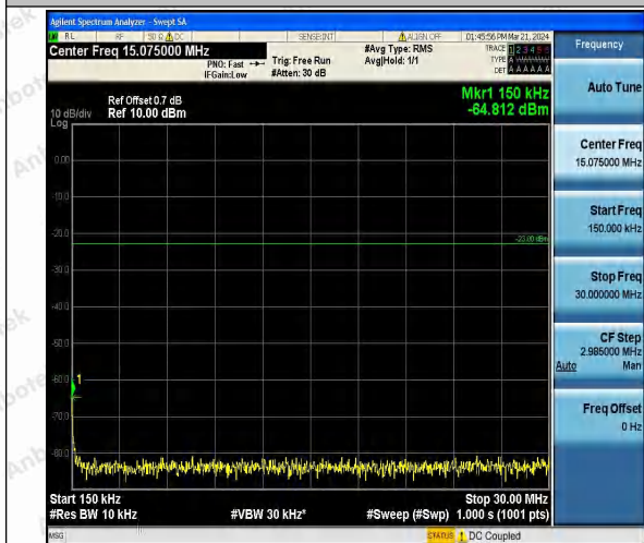
Band26_3MHz_16QAM_26915_1RB#0_0.15~30_0.15~30 30
