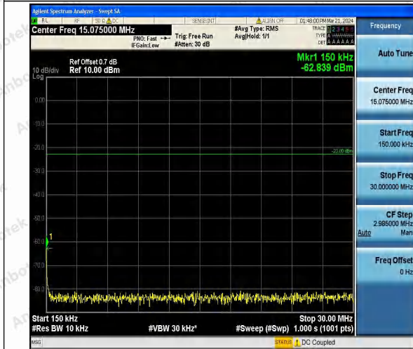
Band26_3MHz_16QAM_27025_1RB#0_0.15~30_0.15~30
