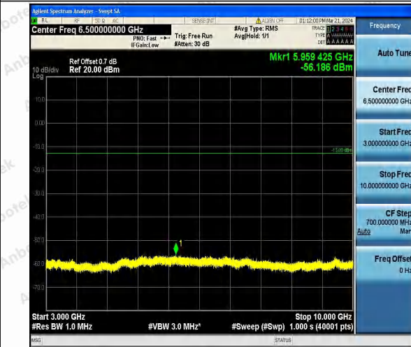
Band26_1.4MHz_16QAM_26797_1RB#0_3000~10000 3000~10000
