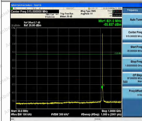
Band26_1.4MHz_QPSK_26797_1RB#0_30~1000_30~1000
