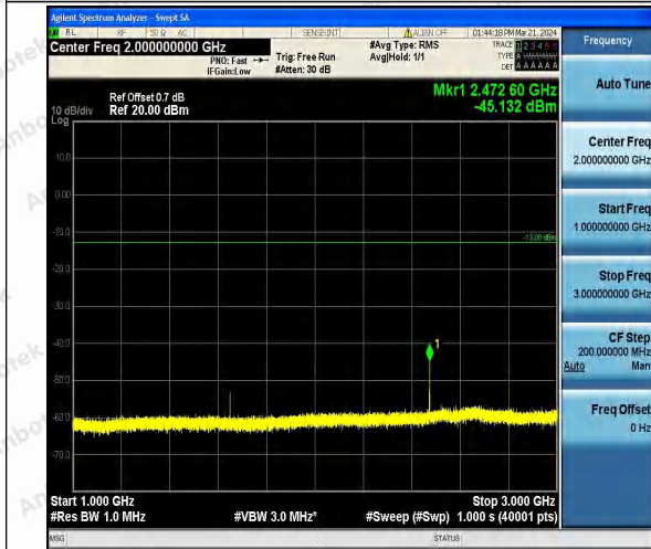
Band26_3MHz_16QAM_26805_1RB#0_1000~3000_1000~3000
