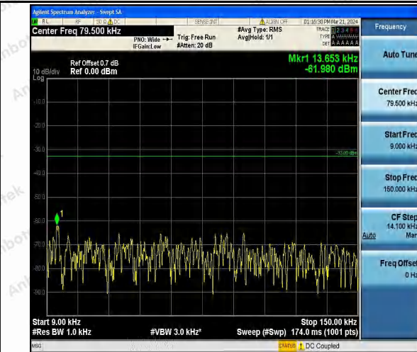
Band26_1.4MHz_16QAM_27033_1RB#0_0.009~0.15_0.009~0.15
