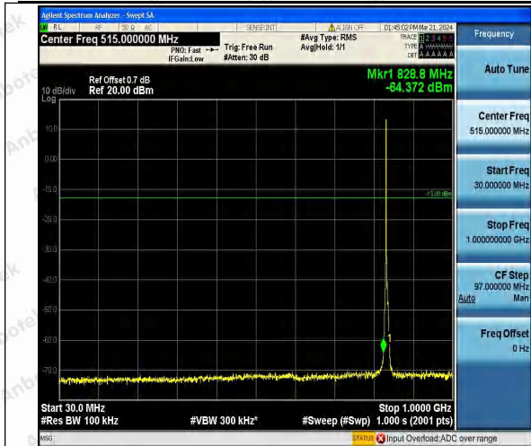
Band26_3MHz_QPSK_26915_1RB#0_30~1000_30~10 00
