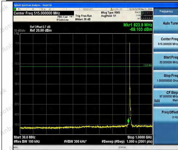
Band26_5MHz_QPSK_26915_1RB#0_30~1000_30~10 00
