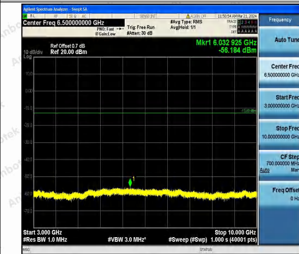
Band26_1.4MHz_16QAM_26783_1RB#0_3000~10000_3000~10000
