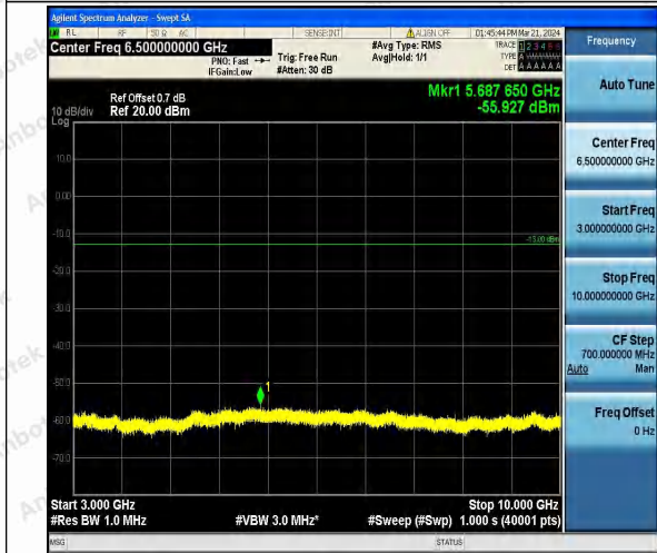
Band26_3MHz_QPSK_26915_1RB#0_3000~10000_3000~10000 00~10000
