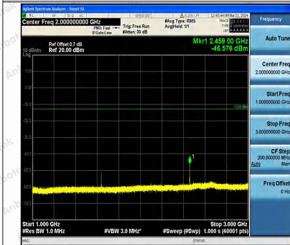
Band26_5MHz_16QAM_26765_1RB#0_1000~3000_1000~3000 00~3000
