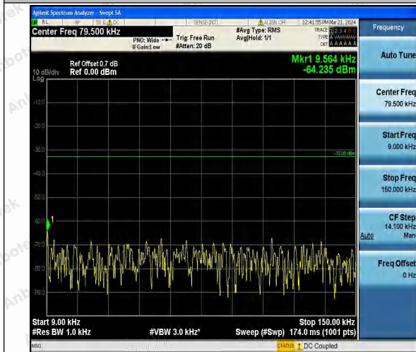
Band26_5MHz_QPSK_26740_1RB#0_0.009~0.15_0.09~0.15
