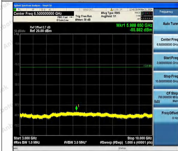
Band26_5MHz_QPSK_26715_1RB#0_3000~10000_3000~10000
