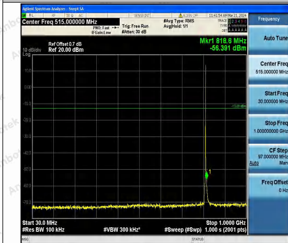
Band26_1.4MHz_QPSK_26697_1RB#0_30~1000_30~1000
