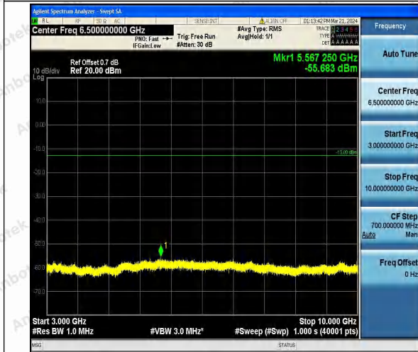
Band26_1.4MHz_QPSK_26915_1RB#0_3000~10000_3000~10000
