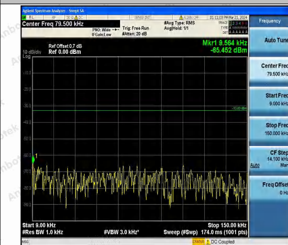
Band26_1.4MHz_16QAM_26797_1RB#0_0.009~0.15_0.009~0.15
