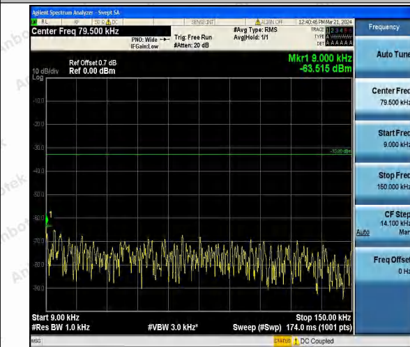
Band26_5MHz_16QAM_26715_1RB#0_0.009~0.15_0.09~0.15
