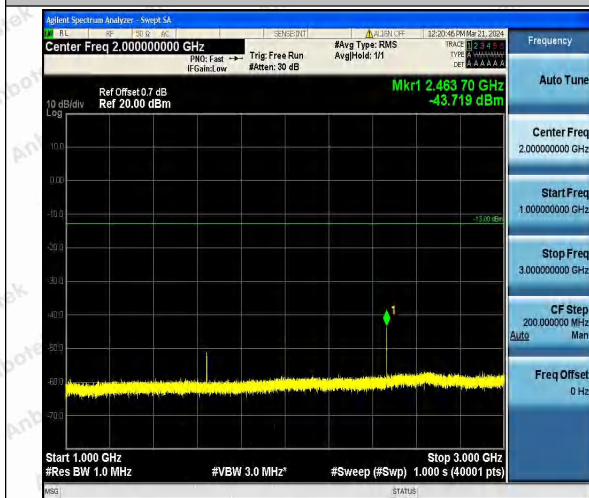
Band26_3MHz_16QAM_26775_1RB#0_1000~3000_10 00~3000
