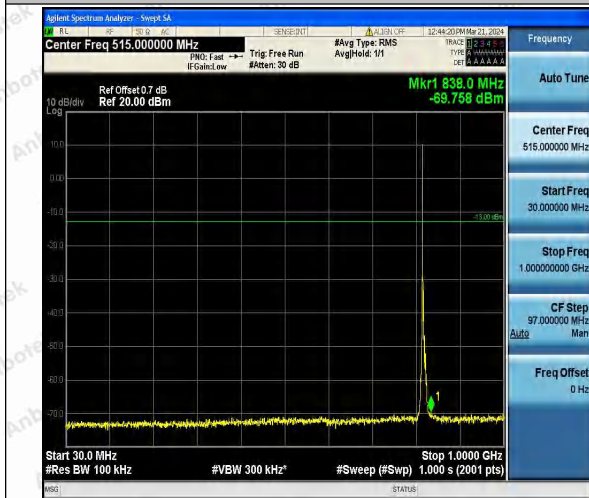
Band26_5MHz_QPSK_26765_1RB#0_30~1000_30~1000
