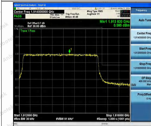
Band25_3MHz_QPSK_26675_15RB#0
