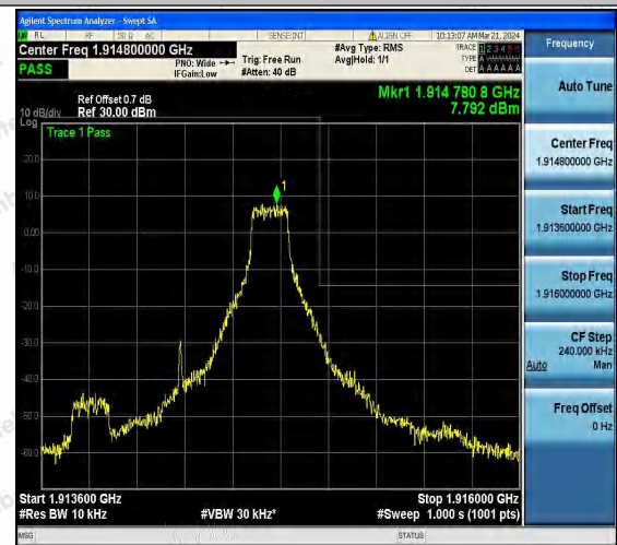
Band25_1.4MHz_16QAM_26683_1RB#5
