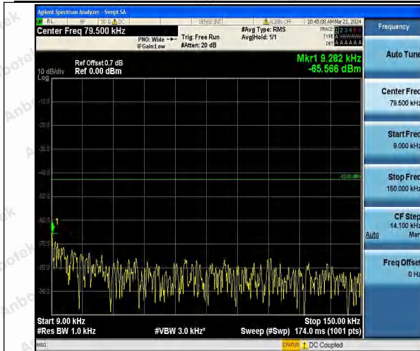
Band25_3MHz_QPSK_26055_1RB#0_0.009~0.15_0.00 9~0.15
