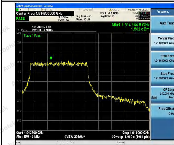
Band25_1.4MHz_QPSK_26683_6RB#0
