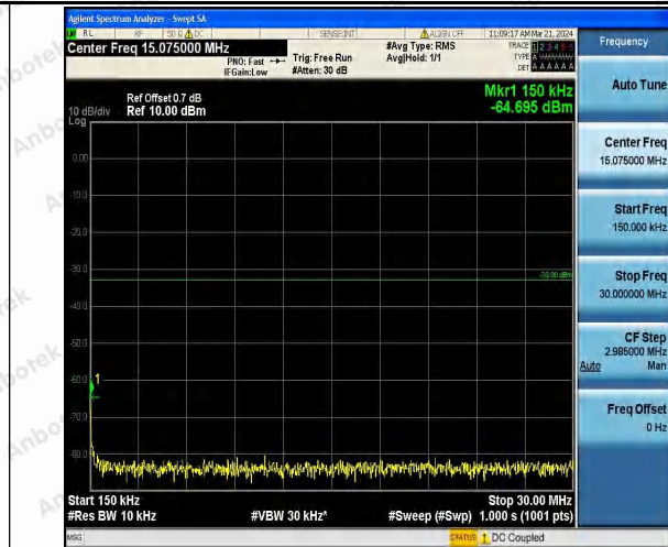
Band25_5MHz_QPSK_26065_1RB#0_0.15~30_0.15~30
