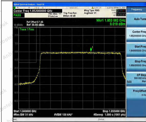
Band25_5MHz_QPSK_26065_25RB#0
