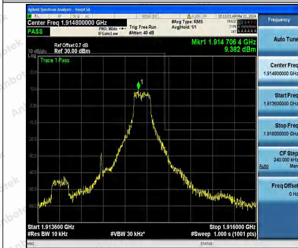
Band25_1.4MHz_QPSK_26683_1RB#5
