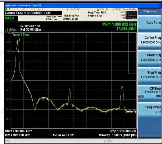
Band25_15MHz_16QAM_26615_1RB#0
