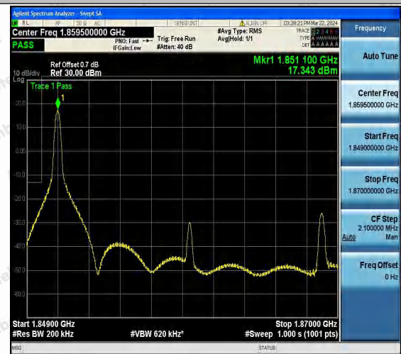
Band25_20MHz_16QAM_26140_1RB#0
