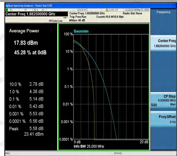
Band25-5MHz-16QAM-26365-1RB#0-PASS
