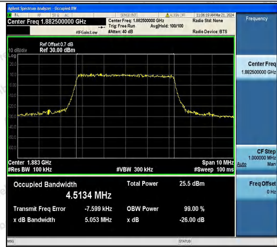
Band25-5MHz-16QAM-26365-25RB#0-PASS
