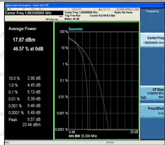
Band25-3MHz-16QAM-26365-1RB#0-PASS
