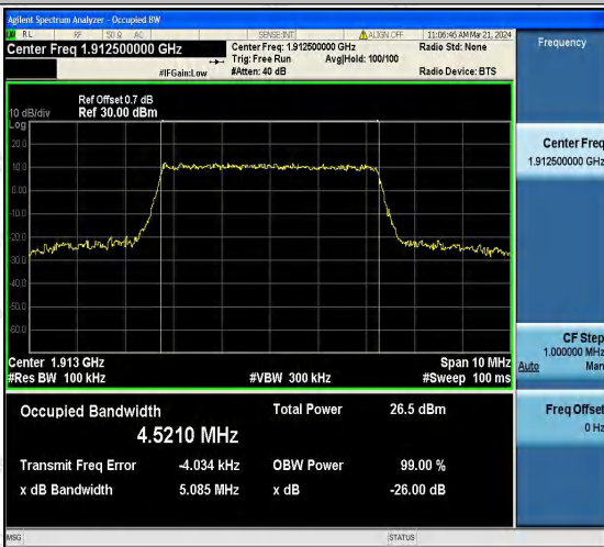
Band25-5MHz-QPSK-26665-25RB#0-PASS
