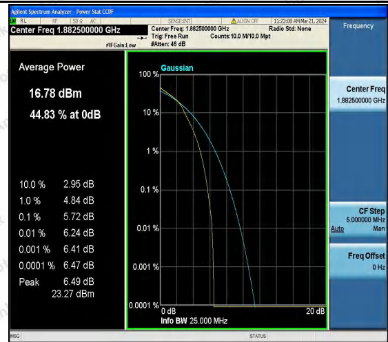
Band25-5MHz-16QAM-26365-25RB#0-PASS
