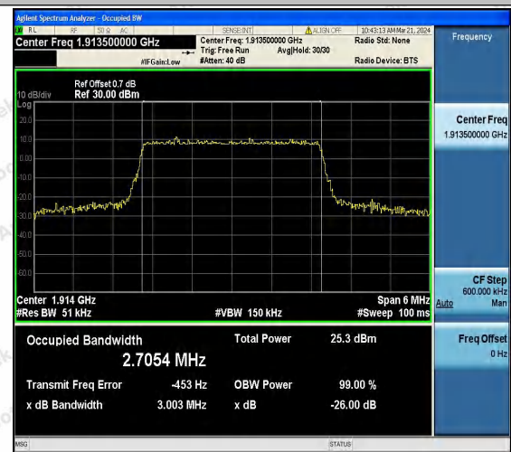
Band25-3MHz-16QAM-26675-15RB#0-PASS
