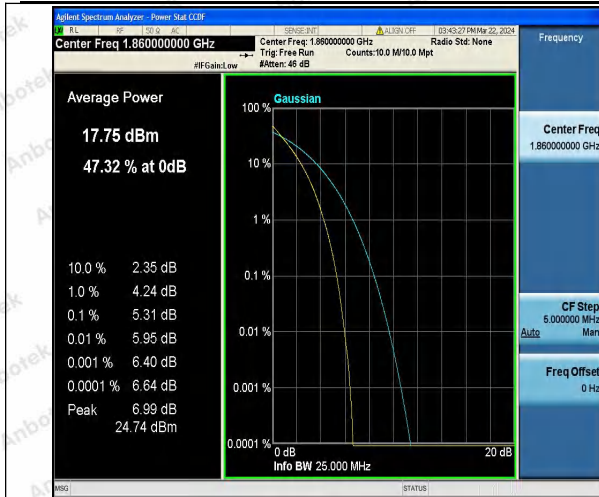
Band25-20MHz-QPSK-26140-100RB#0-PASS
