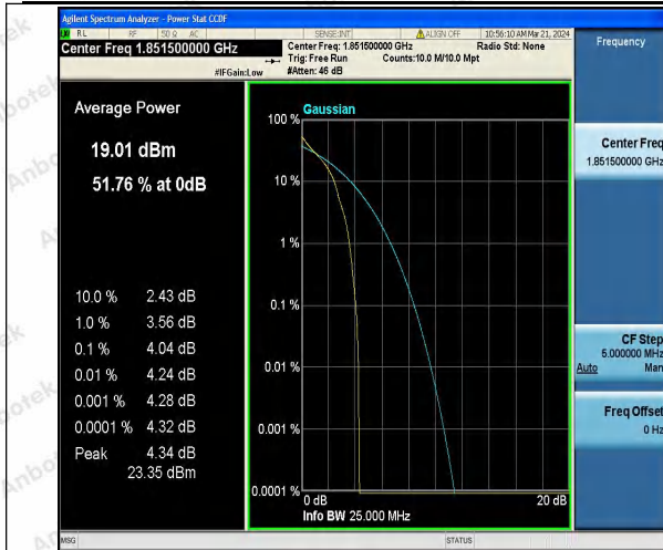
Band25-3MHz-QPSK-26055-1RB#0-PASS
