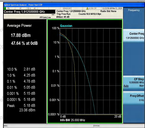
Band25-5MHz-16QAM-26665-1RB#0-PASS
