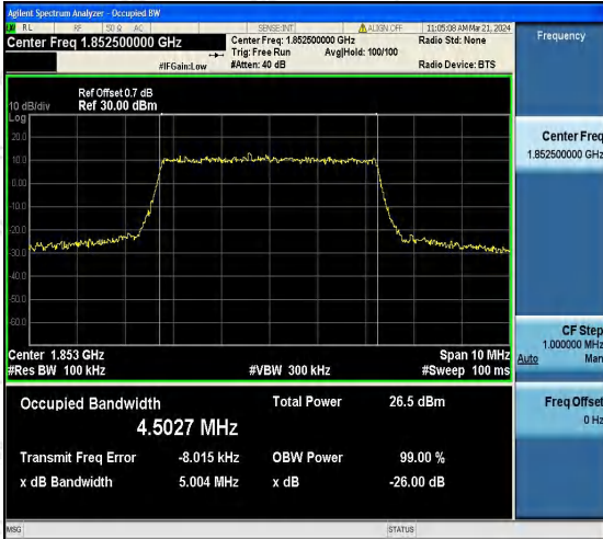
Band25-5MHz-QPSK-26065-25RB#0-PASS
