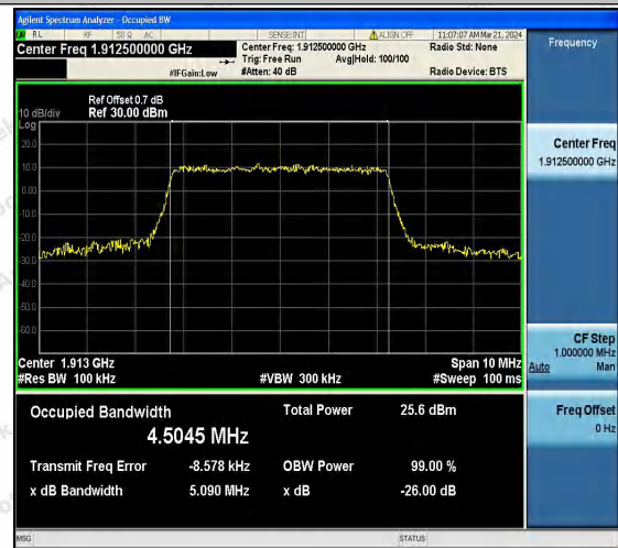
Band25-5MHz-16QAM-26665-25RB#0-PASS
