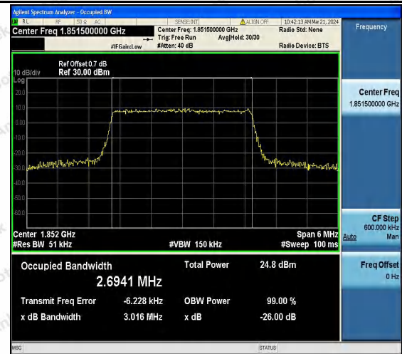
Band25-3MHz-16QAM-26055-15RB#0-PASS
