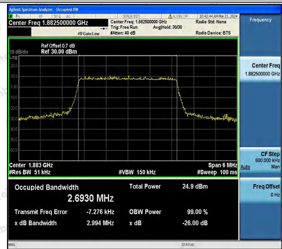
Band25-3MHz-16QAM-26365-15RB#0-PASS
