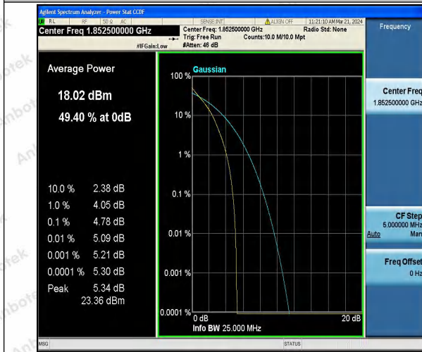
Band25-5MHz-QPSK-26065-25RB#0-PASS
