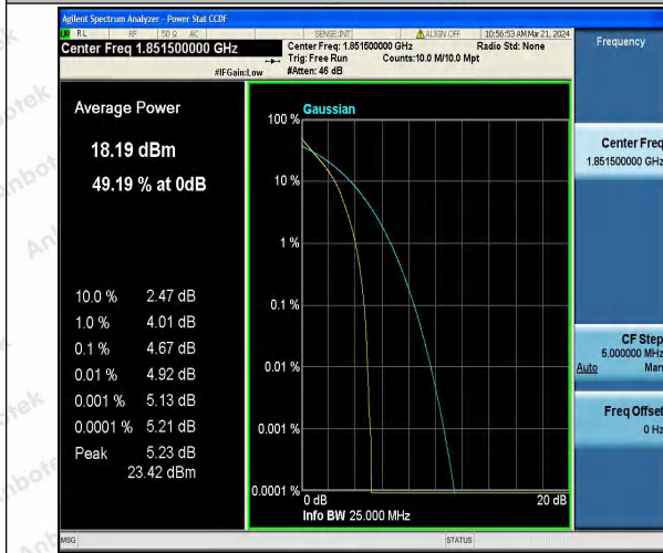
Band25-3MHz-QPSK-26055-15RB#0-PASS
