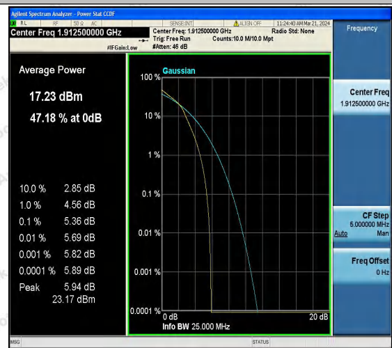
Band25-5MHz-16QAM-26665-25RB#0-PASS
