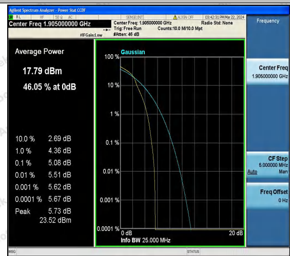
Band25-20MHz-16QAM-26590-1RB#0-PASS
