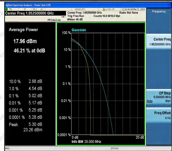
Band25-5MHz-16QAM-26065-1RB#0-PASS
