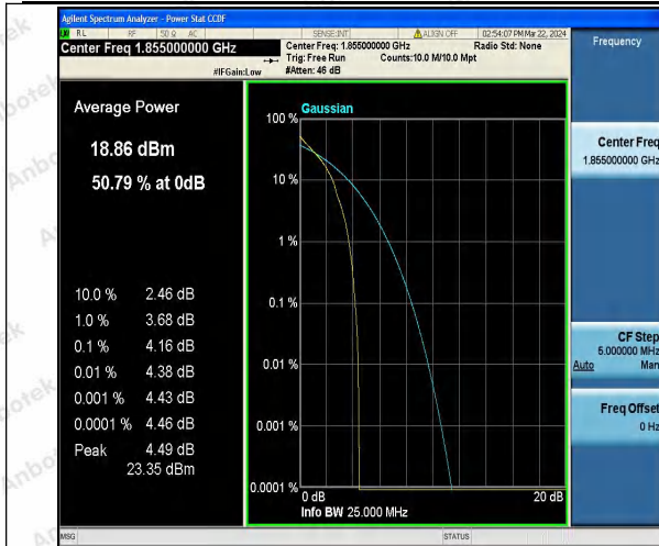
Band25-10MHz-QPSK-26090-1RB#0-PASS
