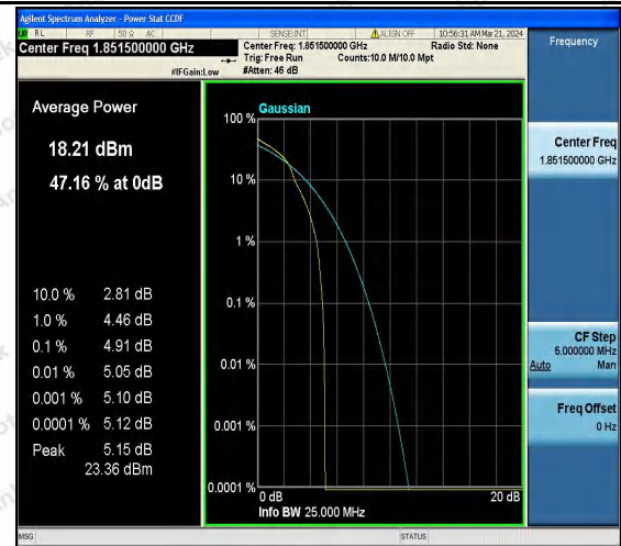
Band25-3MHz-16QAM-26055-1RB#0-PASS
