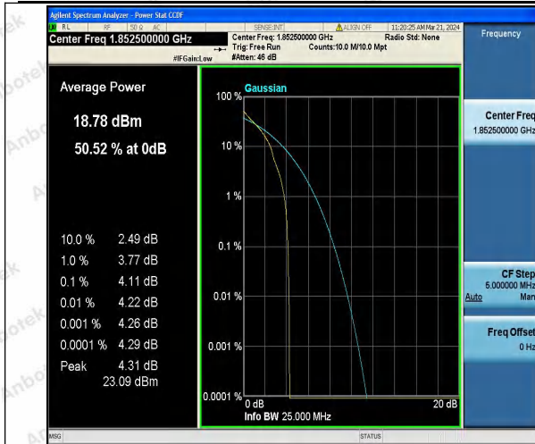
Band25-5MHz-QPSK-26065-1RB#0-PASS
