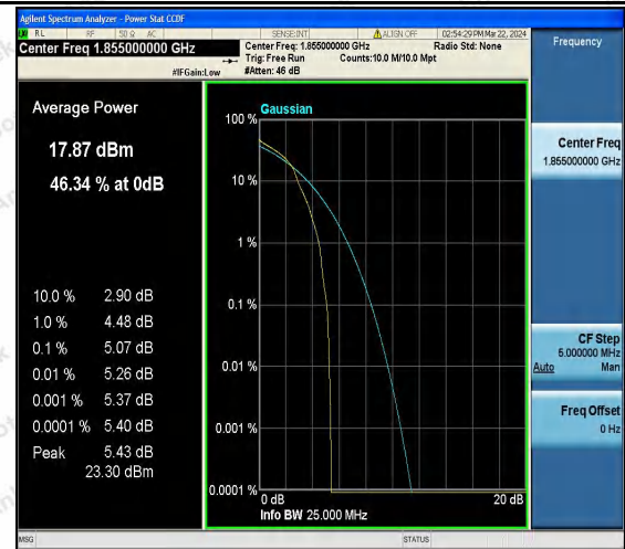
Band25-10MHz-16QAM-26090-1RB#0-PASS
