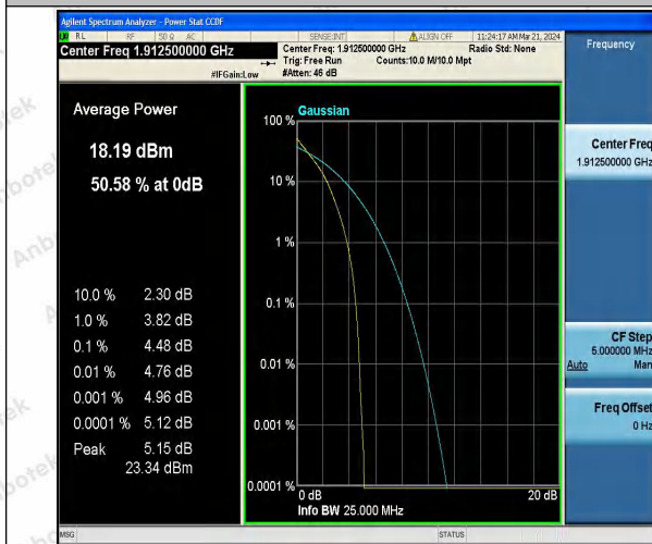
Band25-5MHz-QPSK-26665-25RB#0-PASS
