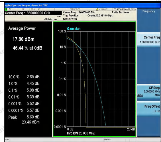
Band25-20MHz-16QAM-26140-1RB#0-PASS
