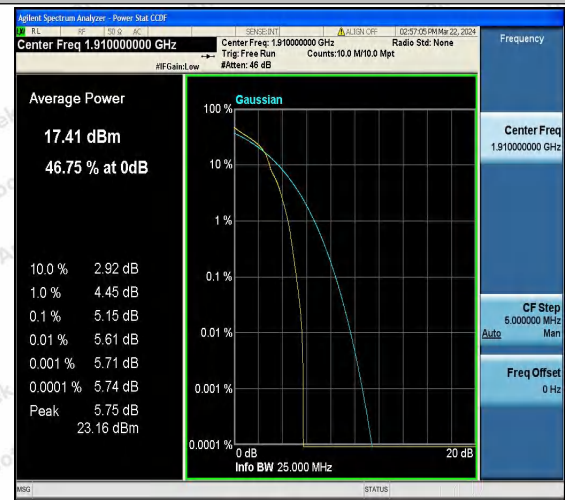
Band25-10MHz-16QAM-26640-1RB#0-PASS
