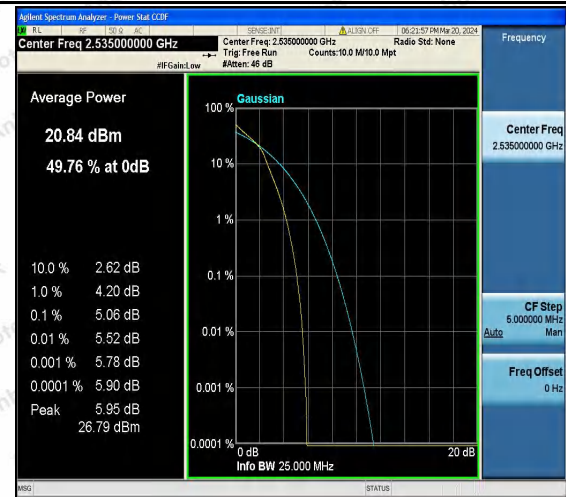
Band7-5MHz-16QAM-21100-25RB#0-PASS
