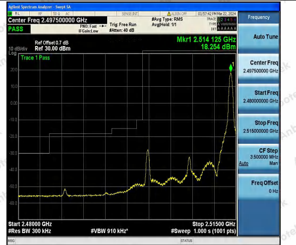
Band7_15MHz_16QAM_20825_1RB#74
