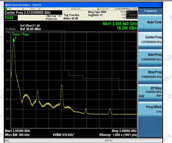
Band7_15MHz_16QAM_21375_1RB#0
