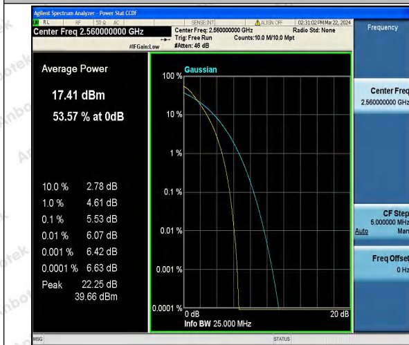
Band7-20MHz-QPSK-21350-100RB#0-PASS
