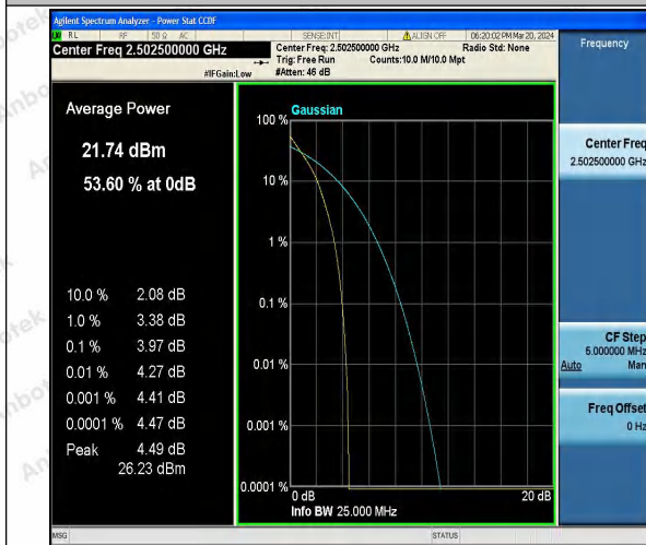
Band7-5MHz-QPSK-20775-25RB#0-PASS
