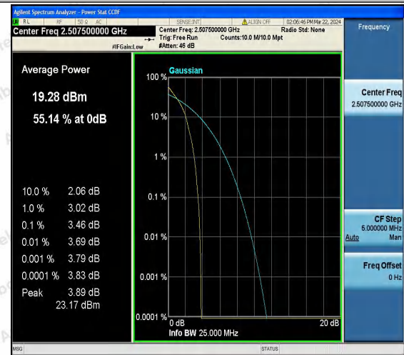
Band7-15MHz-QPSK-20825-1RB#0-PASS
