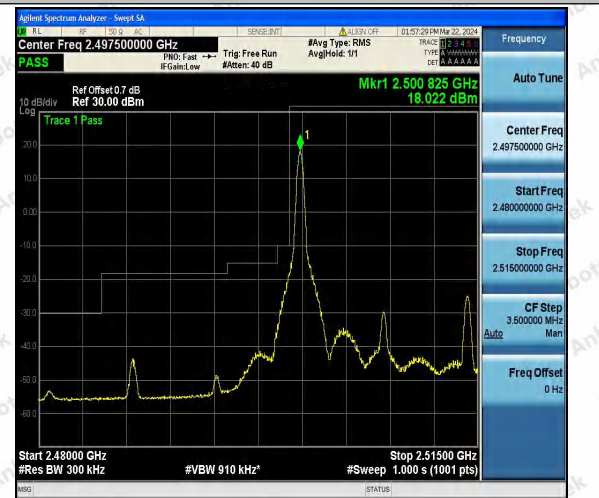
Band7_15MHz_16QAM_20825_1RB#0
