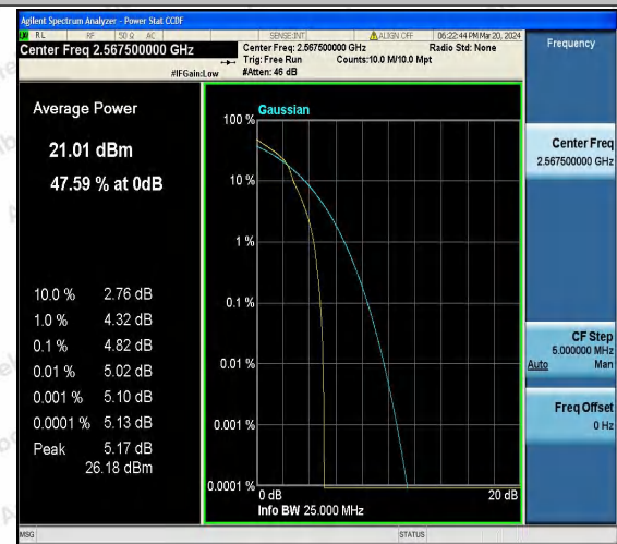
Band7-5MHz-16QAM-21425-1RB#0-PASS
