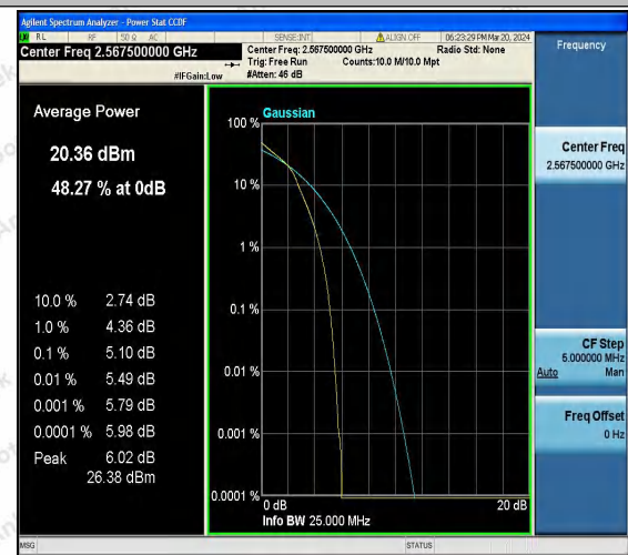
Band7-5MHz-16QAM-21425-25RB#0-PASS
