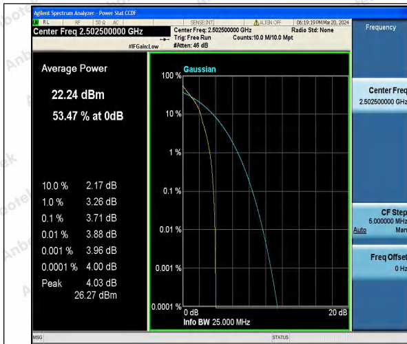
Band7-5MHz-QPSK-20775-1RB#0-PASS
