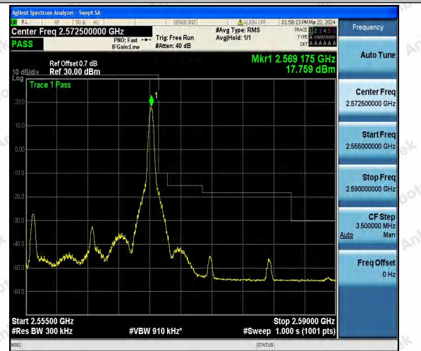
Band7_15MHz_16QAM_21375_1RB#74
