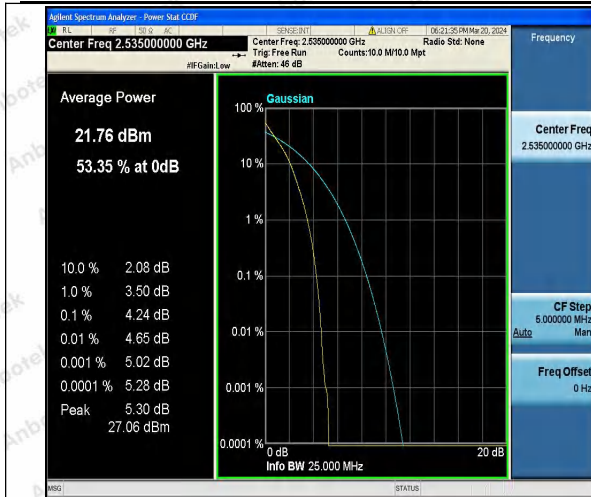
Band7-5MHz-QPSK-21100-25RB#0-PASS
