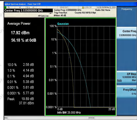
Band7-10MHz-QPSK-21100-50RB#0-PASS
