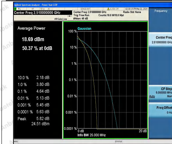
Band7-20MHz-QPSK-20850-100RB#0-PASS
