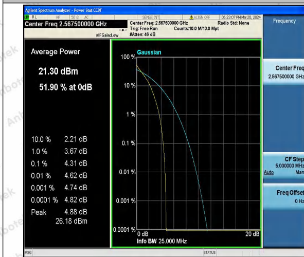
Band7-5MHz-QPSK-21425-25RB#0-PASS
