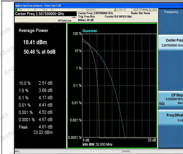
Band7-15MHz-16QAM-20825-1RB#0-PASS
