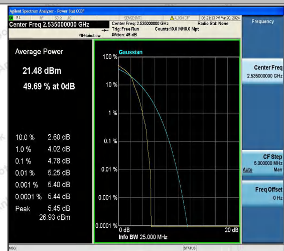
Band7-5MHz-16QAM-21100-1RB#0-PASS
