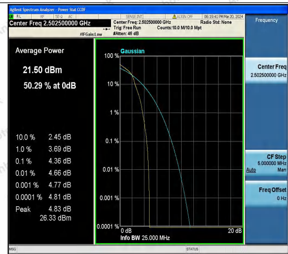
Band7-5MHz-16QAM-20775-1RB#0-PASS
