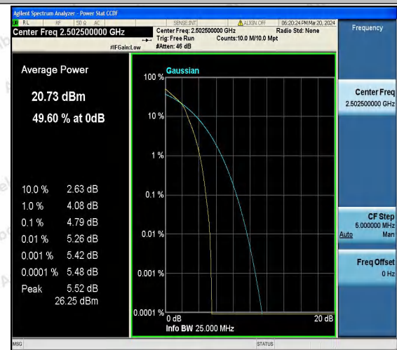
Band7-5MHz-16QAM-20775-25RB#0-PASS
