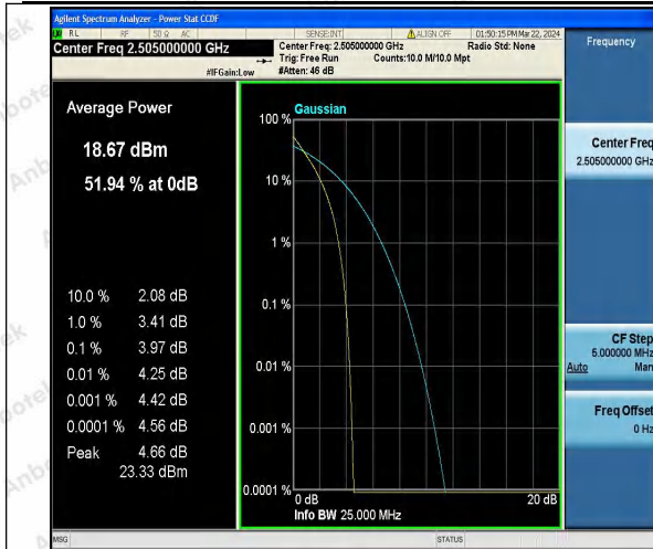
Band7-10MHz-QPSK-20800-50RB#0-PASS
