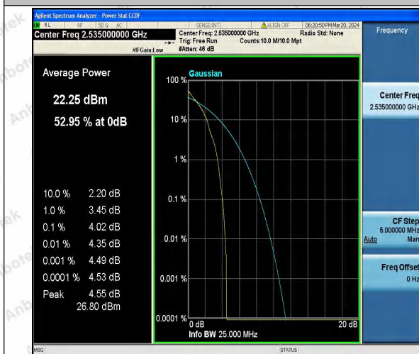
Band7-5MHz-QPSK-21100-1RB#0-PASS
