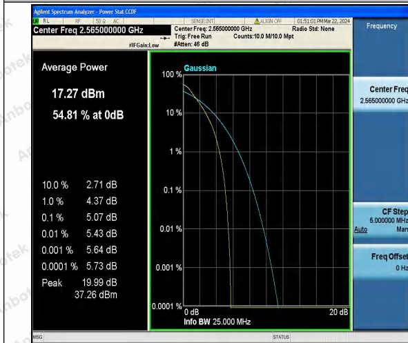
Band7-10MHz-QPSK-21400-50RB#0-PASS
