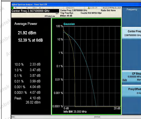
Band7-5MHz-QPSK-21425-1RB#0-PASS
