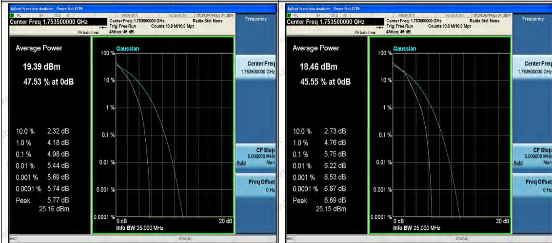
Band4-3MHz-QPSK-20385-15RB#0-PASS
