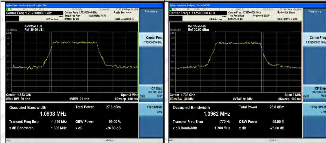
Band4-1.4MHz-QPSK-20175-6RB#0-PASS
