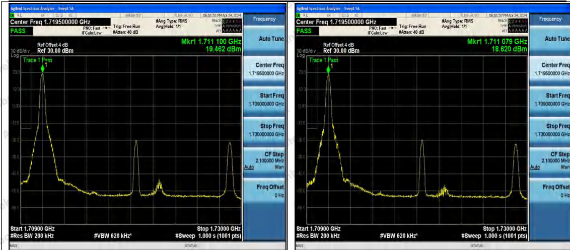
Band4_20MHz_QPSK_20050_1RB#0
