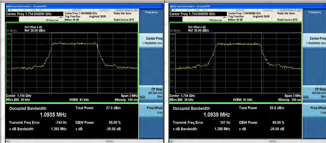
Band4-1.4MHz-QPSK-20393-6RB#0-PASS
