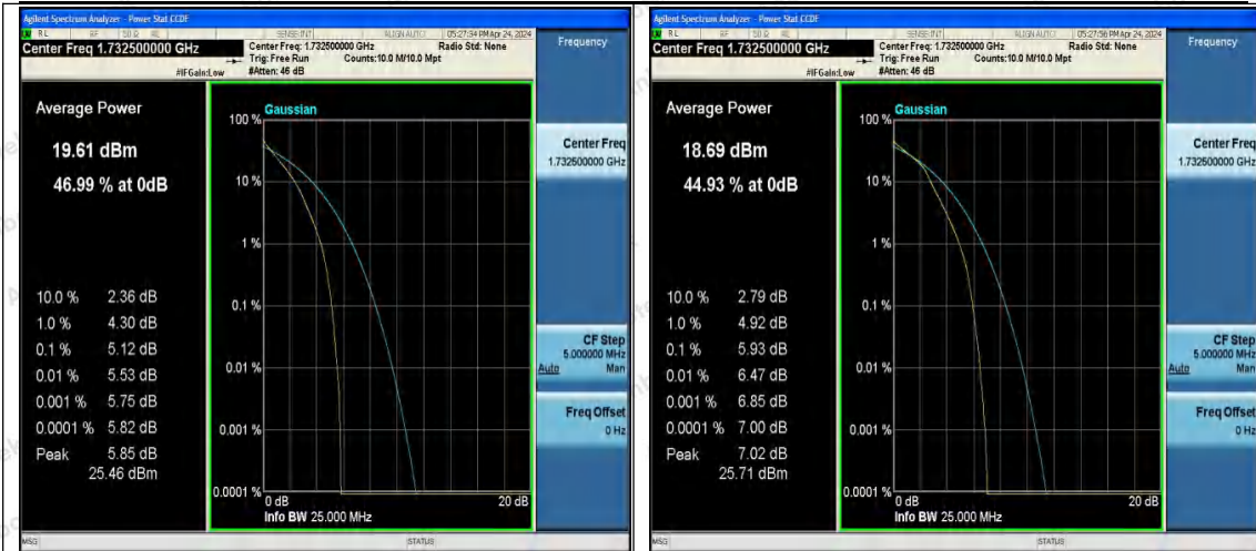
Band4-3MHz-QPSK-20175-15RB#0-PASS
