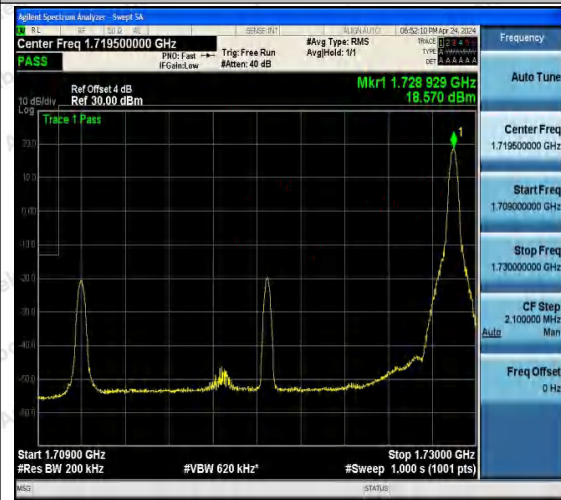
Band4_20MHz_16QAM_20050_1RB#99
