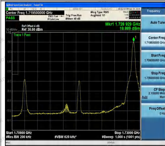
Band4_20MHz_QPSK_20050_1RB#99
