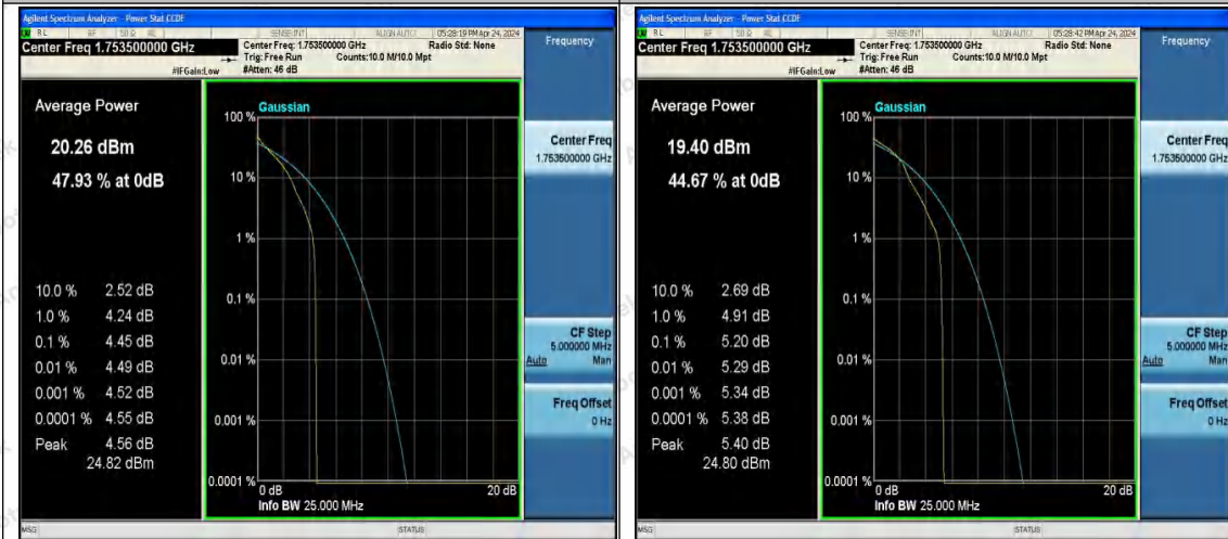
Band4-3MHz-QPSK-20385-1RB#0-PASS
