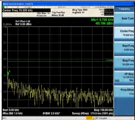
Band66_1.4MHz_16QAM_131979_1RB#0_0.009~ 0.15_0.009~0.15
