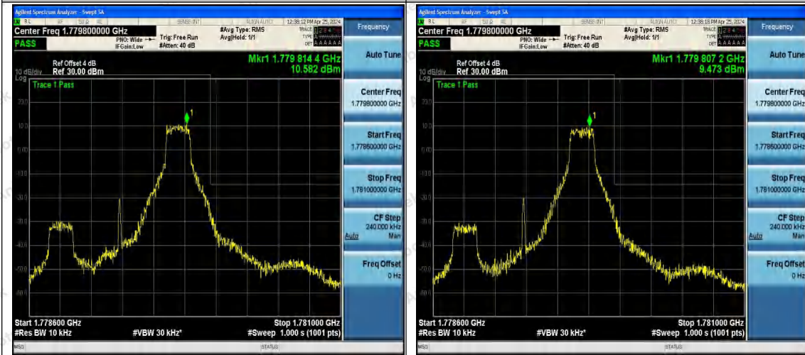
Band66_1.4MHz_QPSK_132665_1RB#5
