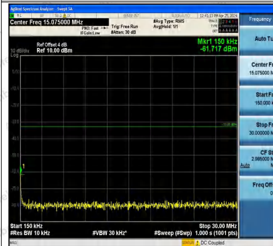
Band66_1.4MHz_16QAM_131979_1RB#0_0.15~ 30_0.15~30
