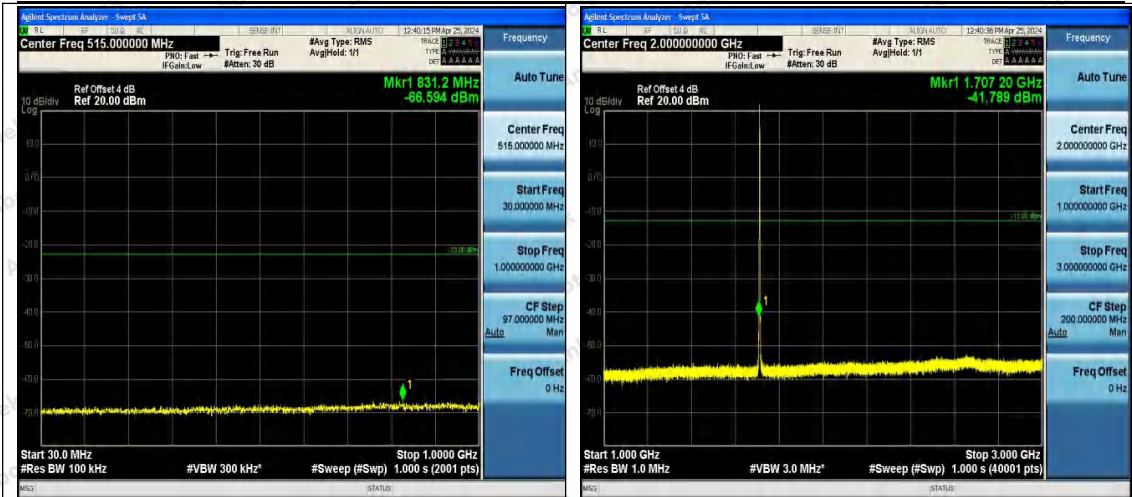
Band66_1.4MHz_QPSK_131979_1RB#0_30~100 0_30~1000
