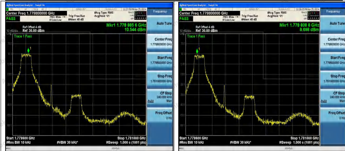
Band66_1.4MHz_QPSK_132665_1RB#0
