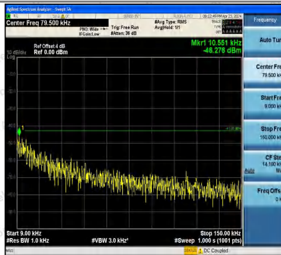
Band4-1513-4-0.009~0.15MHz-PASS
