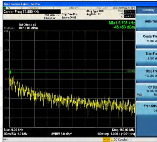
Band4-1312-5-0.009~0.15MHz-PASS
