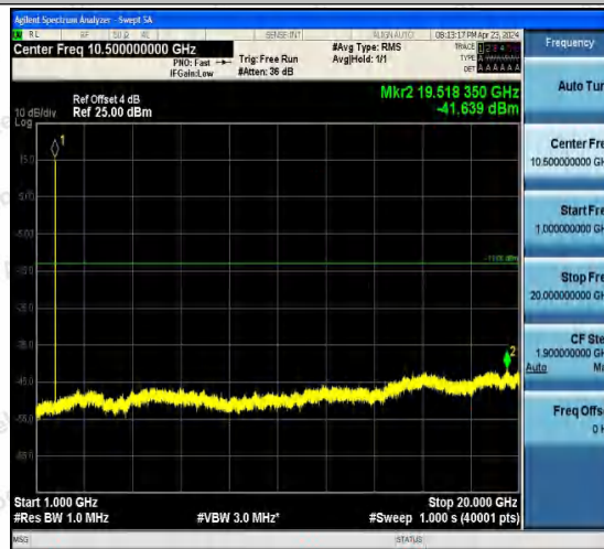
Band4-1513-4-1000~20000MHz-PASS
