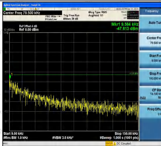
Band4-1413-1-0.009~0.15MHz-PASS
