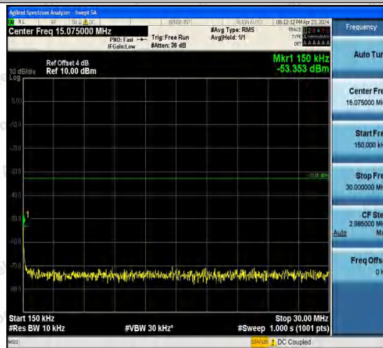
Band4-1413-4-0.15~30MHz-PASS
