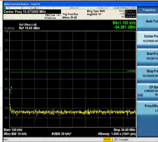
Band4-1513-2-0.15~30MHz-PASS
