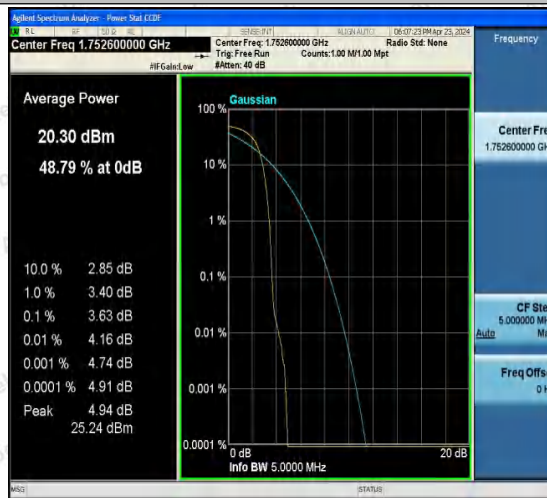
Band4-1513-4-PASS
