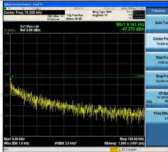
Band4-1312-2-0.009~0.15MHz-PASS
