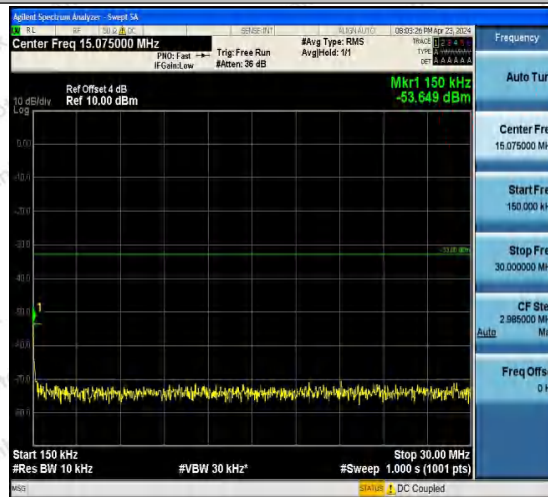
Band4-1312-1-0.15~30MHz-PASS
