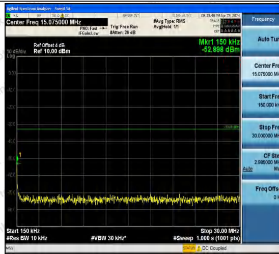
Band4-1312-5-0.15~30MHz-PASS
