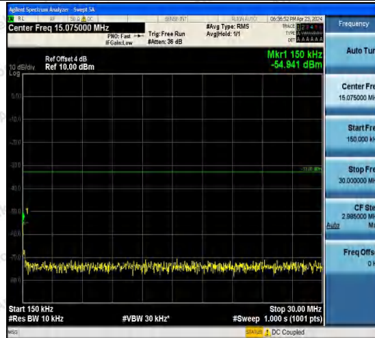
Band4-1513-1-0.15~30MHz-PASS
