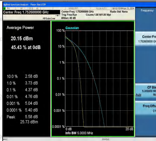
Band4-1513-1-PASS
