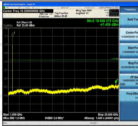
Band4-1413-2-1000~20000MHz-PASS
