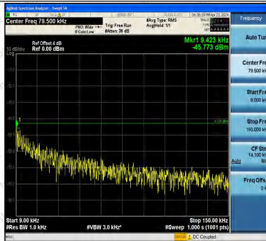
Band4-1413-2-0.009~0.15MHz-PASS
