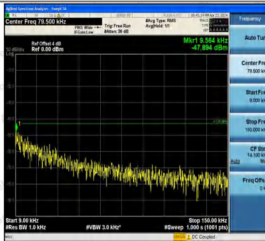
Band4-1513-3-0.009~0.15MHz-PASS
