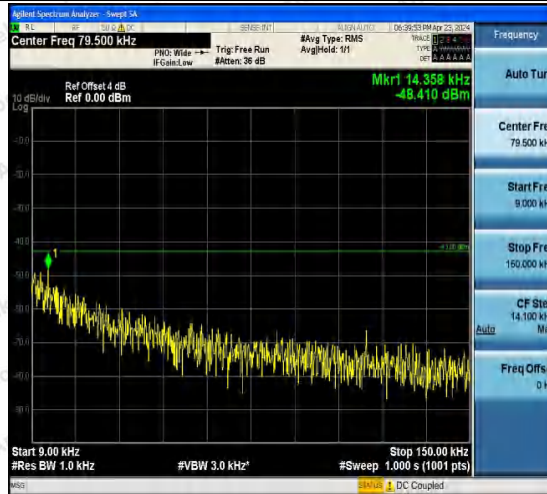
Band4-1312-3-0.009~0.15MHz-PASS
