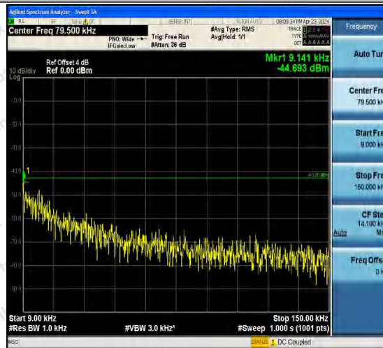
Band4-1413-3-0.009~0.15MHz-PASS
