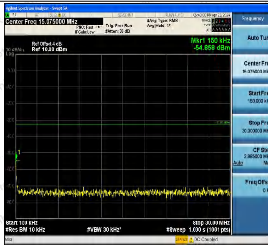
Band4-1312-3-0.15~30MHz-PASS
