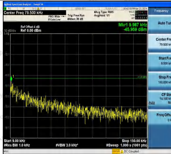
Band4-1312-4-0.009~0.15MHz-PASS
