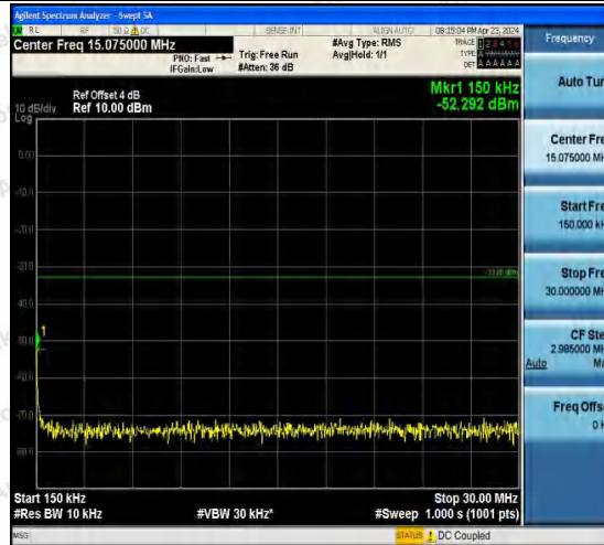
Band4-1513-5-0.15~30MHz-PASS
