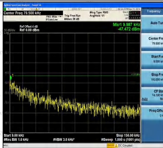
Band4-1413-5-0.009~0.15MHz-PASS
