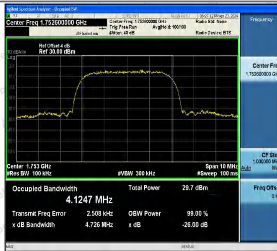
Band4-1513-1-PASS
