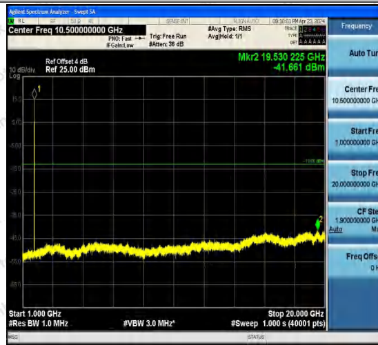
Band4-1413-3-1000~20000MHz-PASS
