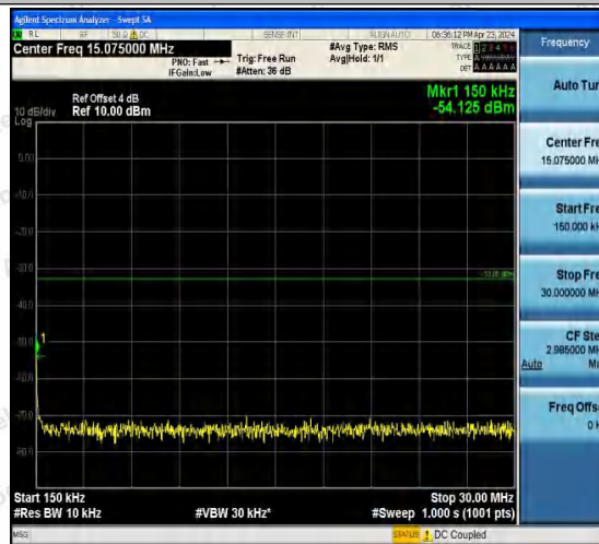
Band4-1413-1-0.15~30MHz-PASS
