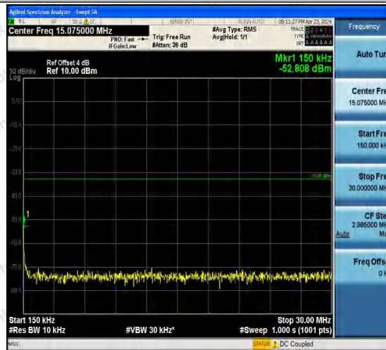
Band4-1312-4-0.15~30MHz-PASS
