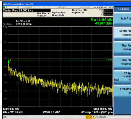
Band4-1413-4-0.009~0.15MHz-PASS
