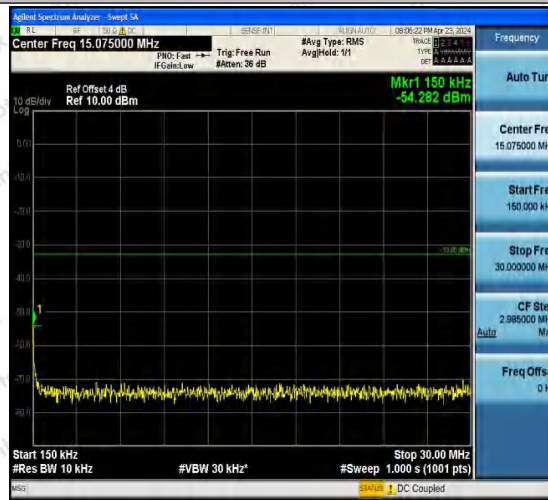
Band4-1312-2-0.15~30MHz-PASS
