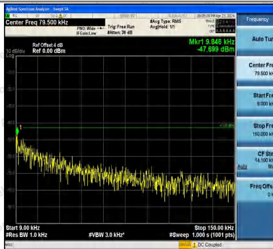
Band4-1513-1-0.009~0.15MHz-PASS
