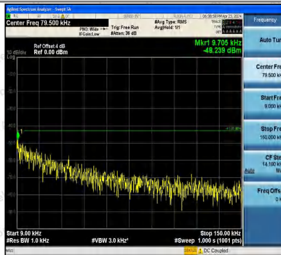
Band4-1513-2-0.009~0.15MHz-PASS
