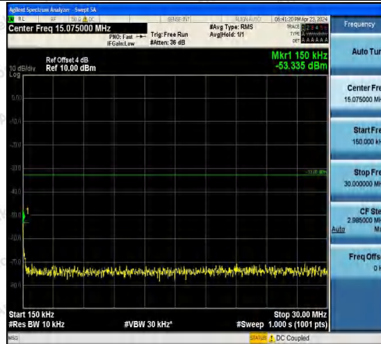
Band4-1513-3-0.15~30MHz-PASS
