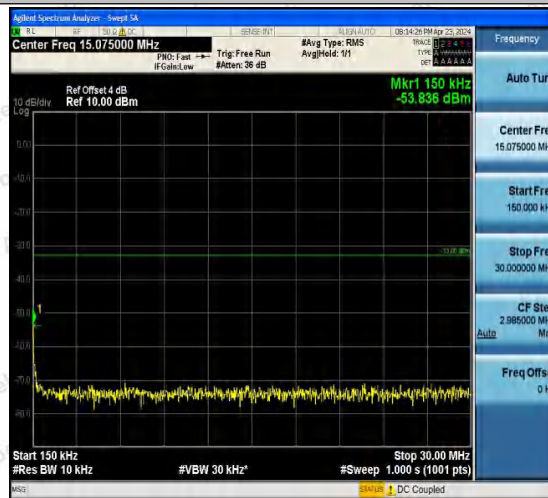
Band4-1413-5-0.15~30MHz-PASS
