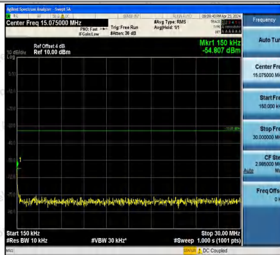
Band4-1413-3-0.15~30MHz-PASS
