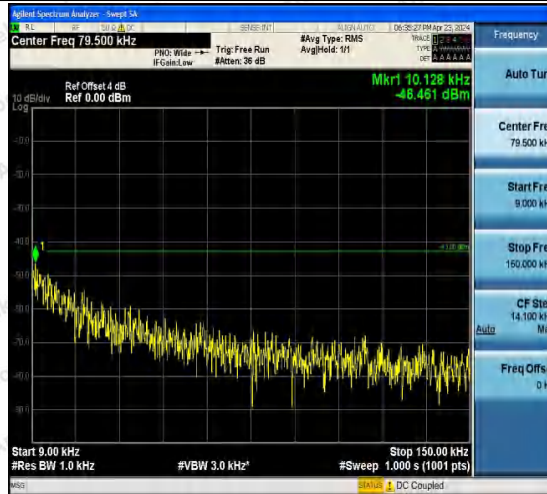
Band4-1312-1-0.009~0.15MHz-PASS
