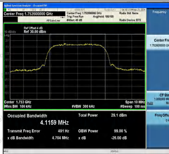
Band4-1513-3-PASS
