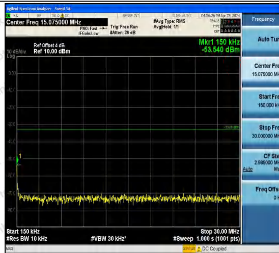
Band2-9262-2-0.15~30MHz-PASS
