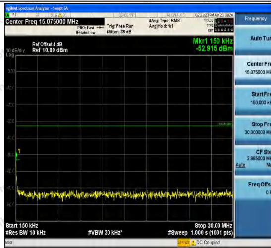
Band2-9262-2-0.15~30MHz-PASS
