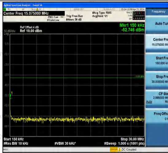
Band2-9262-5-0.15~30MHz-PASS
