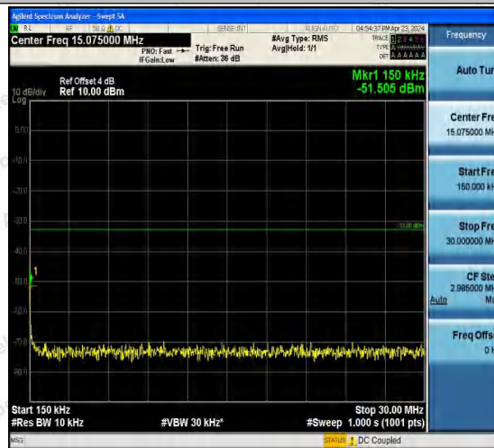
Band2-9400-1-0.15~30MHz-PASS
