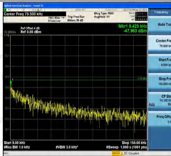
Band2-9538-4-0.009~0.15MHz-PASS
