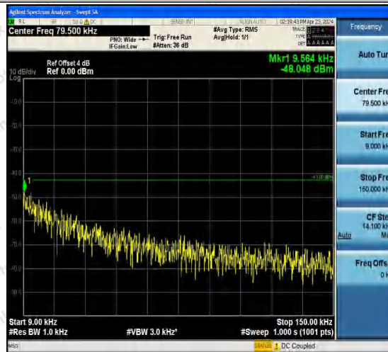
Band2-9400-1-0.009~0.15MHz-PASS
