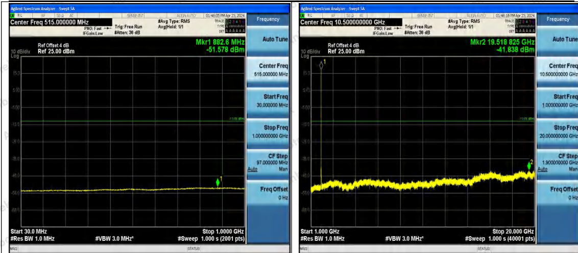
Band2-9400-30~1000MHz-PASS
