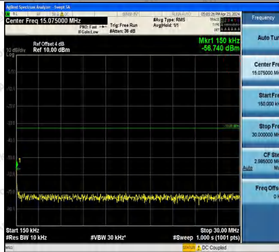
Band2-9538-4-0.15~30MHz-PASS
