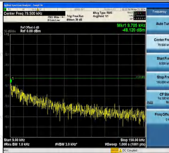
Band2-9400-2-0.009~0.15MHz-PASS
