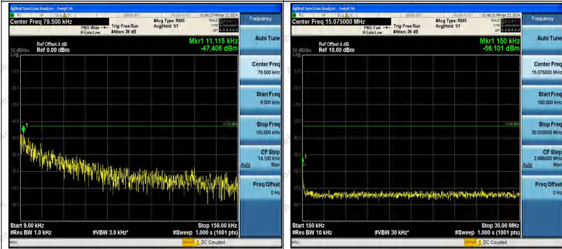
Band2-9538-0.009~0.15MHz-PASS
