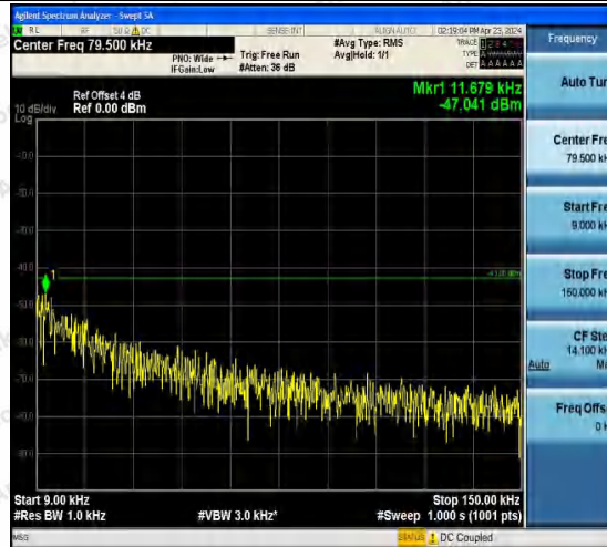
Band2-9262-1-0.009~0.15MHz-PASS
