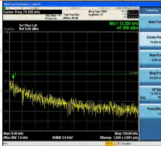
Band2-9262-5-0.009~0.15MHz-PASS
