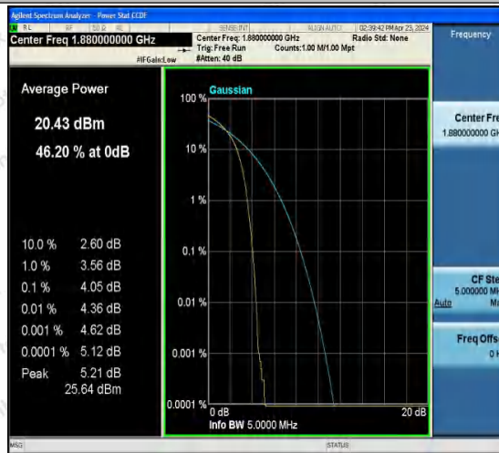
Band2-9400-5-PASS
