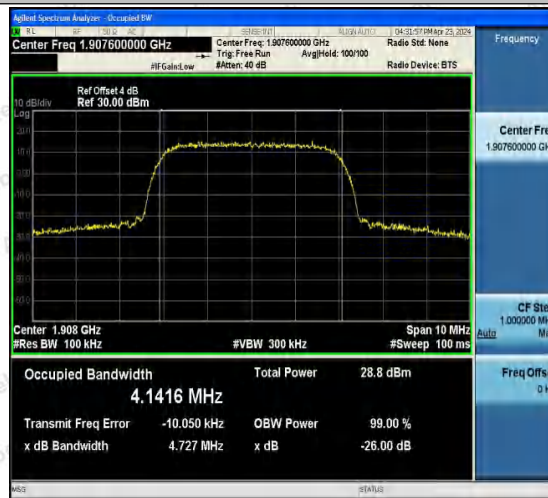
Band2-9538-1-PASS
