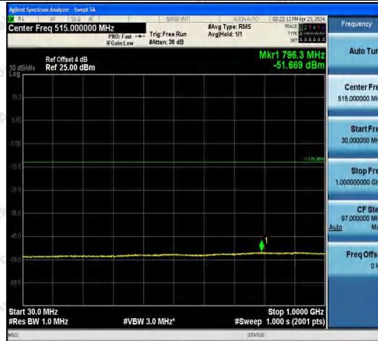
Band2-9400-2-30~1000MHz-PASS
