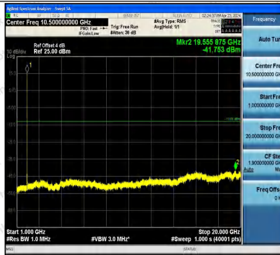
Band2-9400-3-1000~20000MHz-PASS
