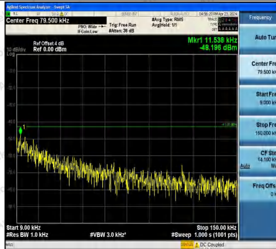
Band2-9262-2-0.009~0.15MHz-PASS
