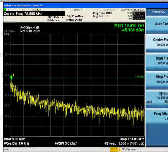
Band2-9538-3-0.009~0.15MHz-PASS
