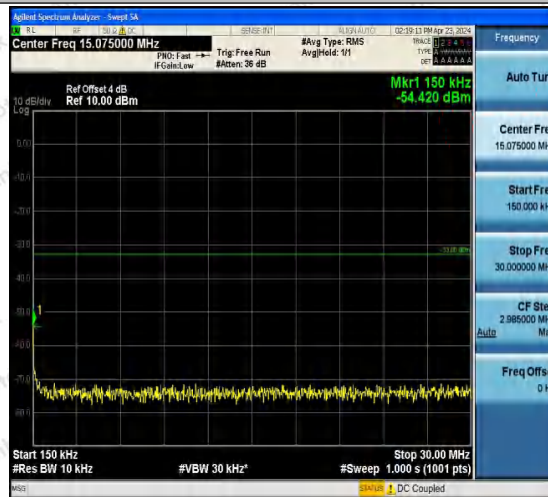
Band2-9262-1-0.15~30MHz-PASS
