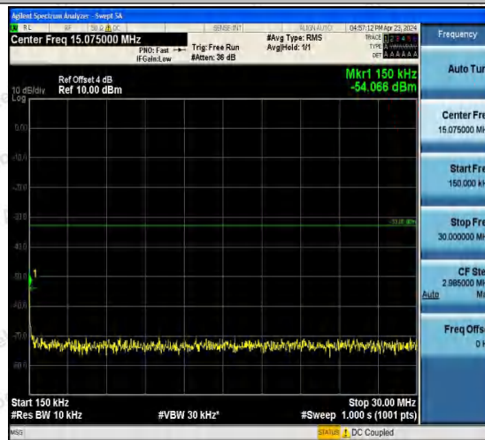
Band2-9400-2-0.15~30MHz-PASS
