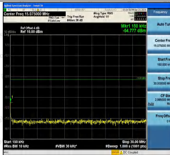
Band2-9400-5-0.15~30MHz-PASS
