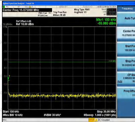
Band2-9538-1-0.15~30MHz-PASS
