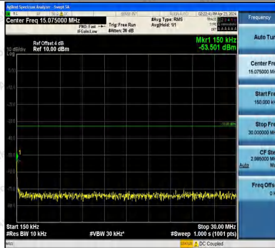
Band2-9538-2-0.15~30MHz-PASS
