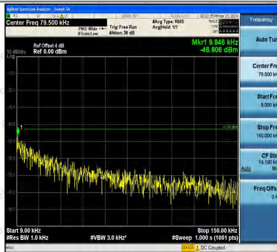
Band2-9538-2-0.009~0.15MHz-PASS
