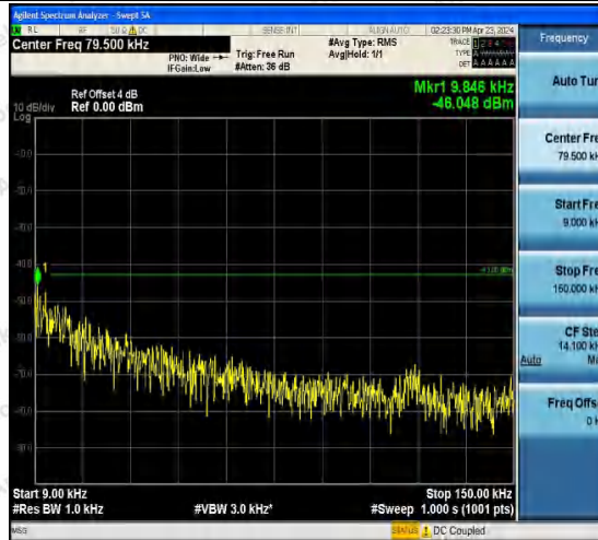
Band2-9262-3-0.009~0.15MHz-PASS
