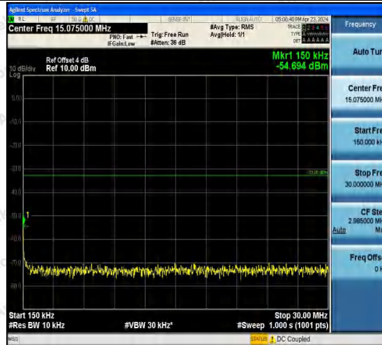
Band2-9538-3-0.15~30MHz-PASS
