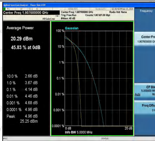
Band2-9538-5-PASS
