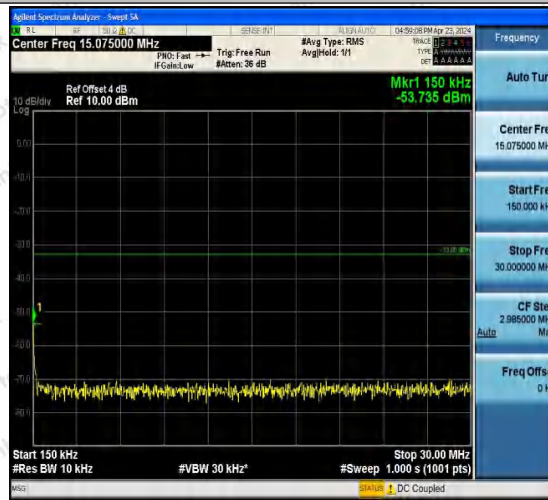
Band2-9262-3-0.15~30MHz-PASS
