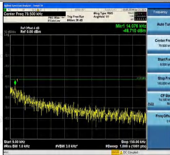
Band2-9538-5-0.009~0.15MHz-PASS
