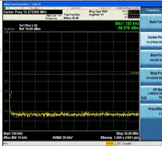
Band2-9538-5-0.15~30MHz-PASS
