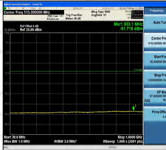
Band2-9400-4-30~1000MHz-PASS
