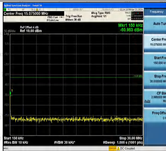
Band2-9400-3-0.15~30MHz-PASS
