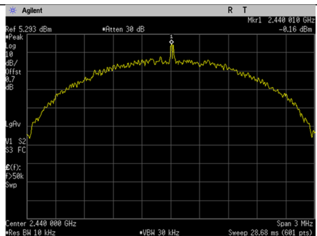
BLE_Mid Ch_2440MHz_2MBit_Spectral Density
