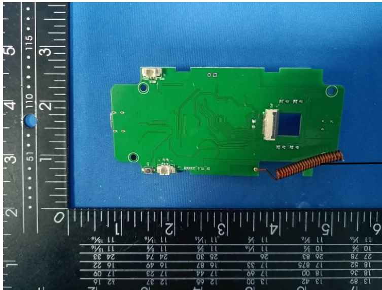
433MHz Spring Antenna
