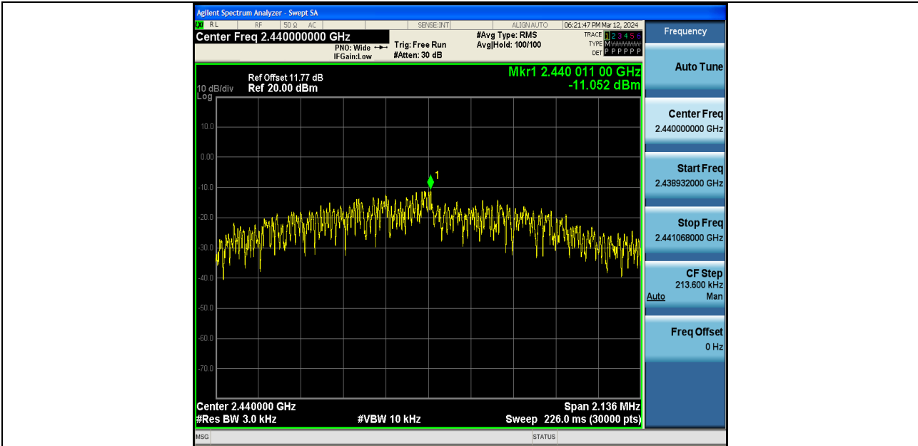
BLE_2M-Ant1-2440-PASS
