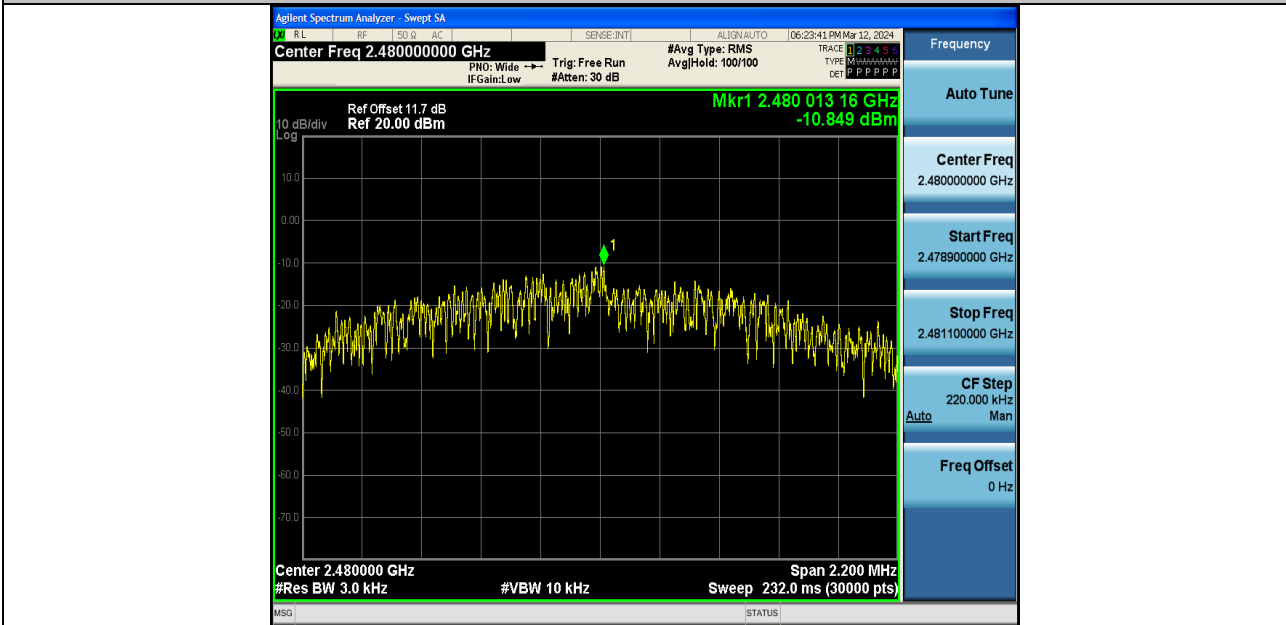
BLE_2M-Ant1-2480-PASS
