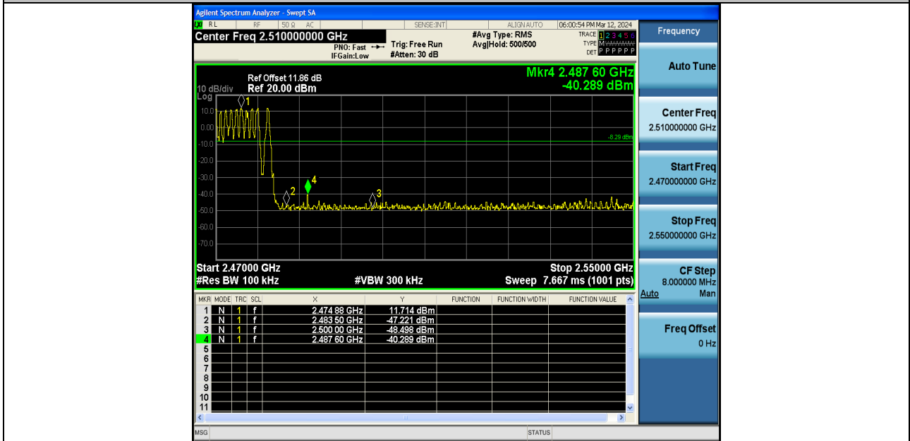
DH5-Ant1-Hop_2480-PASS
