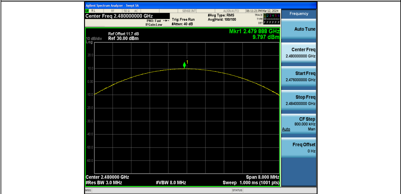
3DH5-Ant1-2480-PASS
