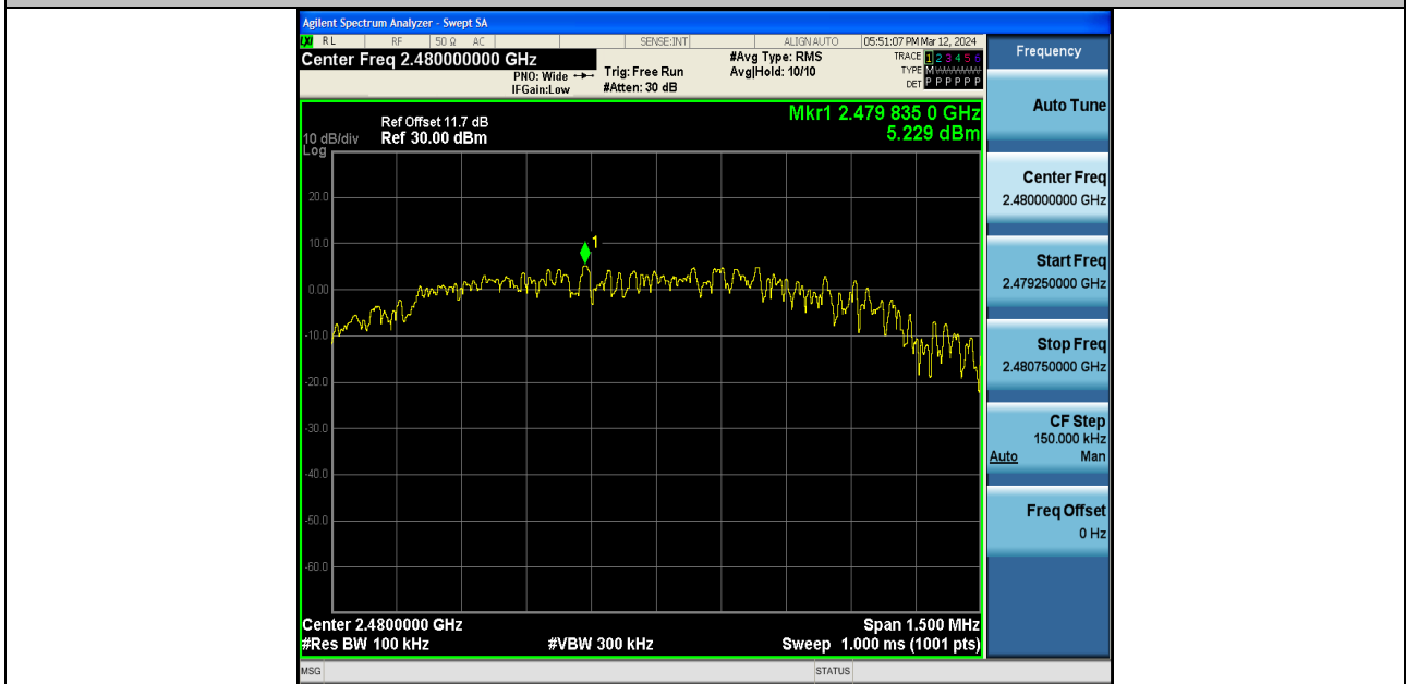
2DH5-Ant1-2480-0~Reference-PASS
