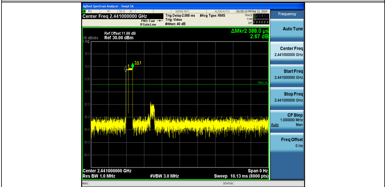
3DH1-Ant1-Hop-PASS
