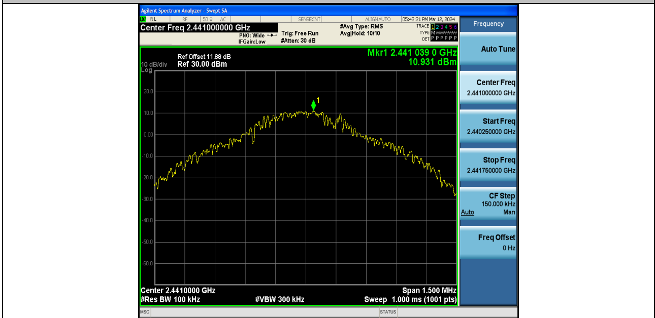
DH5-Ant1-2441-0~Reference-PASS
