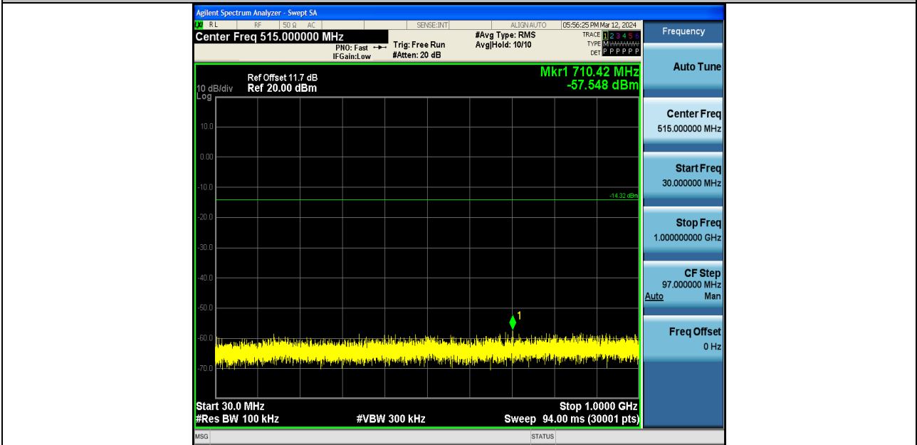
3DH5-Ant1-2480-30~1000-PASS
