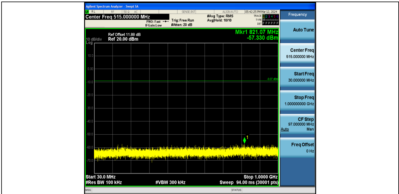
DH5-Ant1-2441-30~1000-PASS
