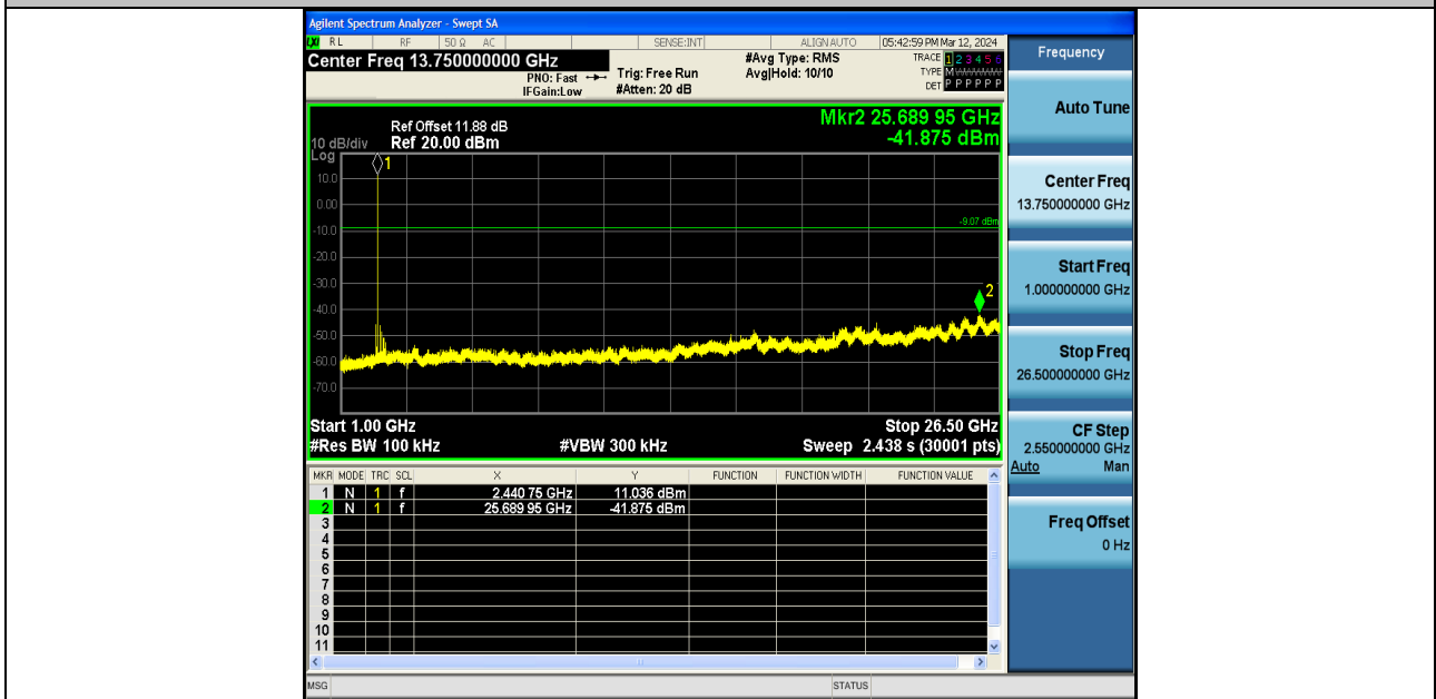
DH5-Ant1-2441-1000~26500-PASS
