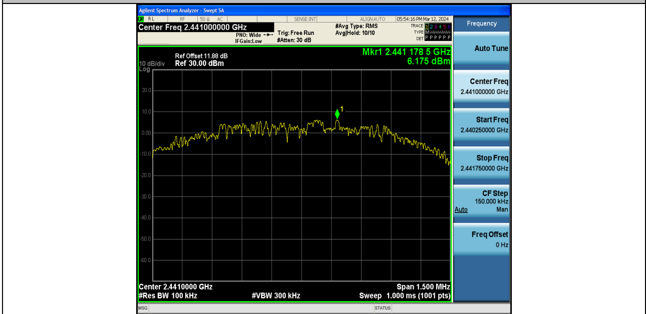
3DH5-Ant1-2441-0~Reference-PASS
