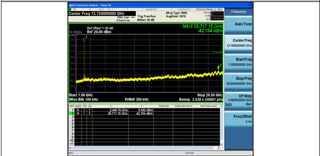
3DH5-Ant1-2441-1000~26500-PASS
