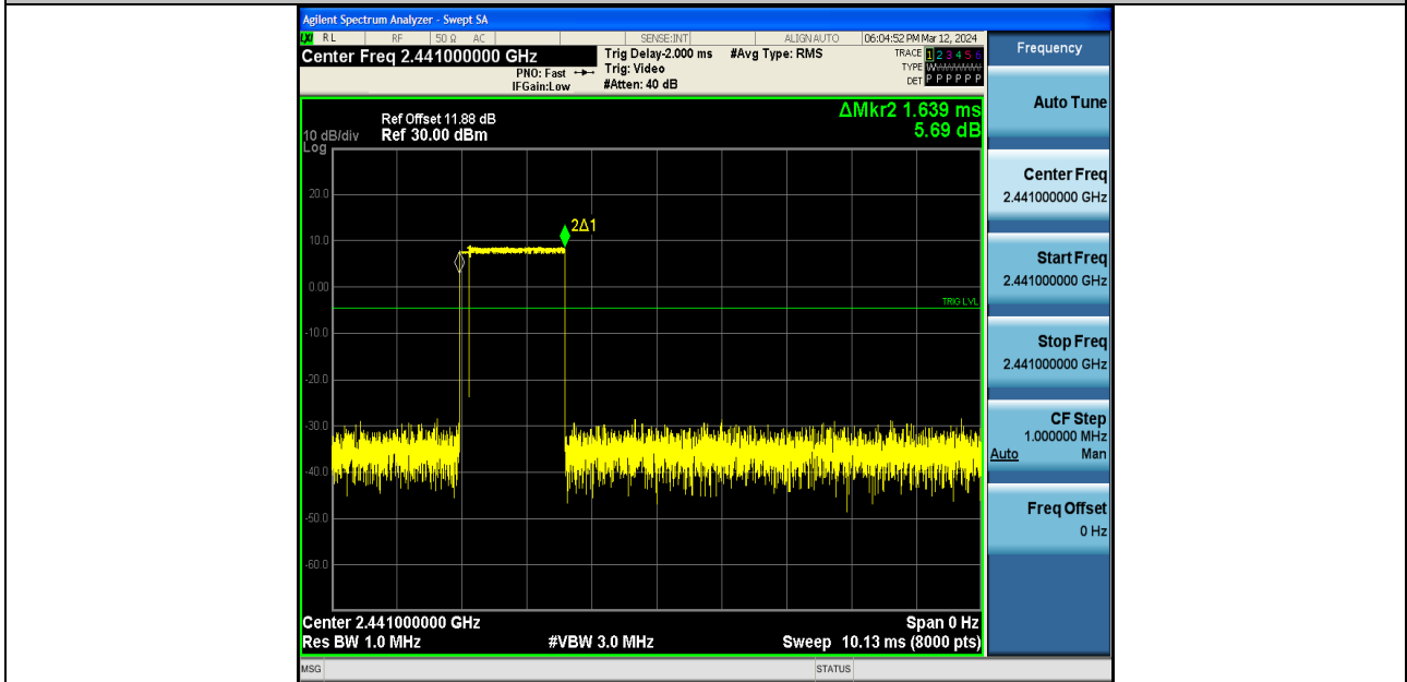
2DH3-Ant1-Hop-PASS
