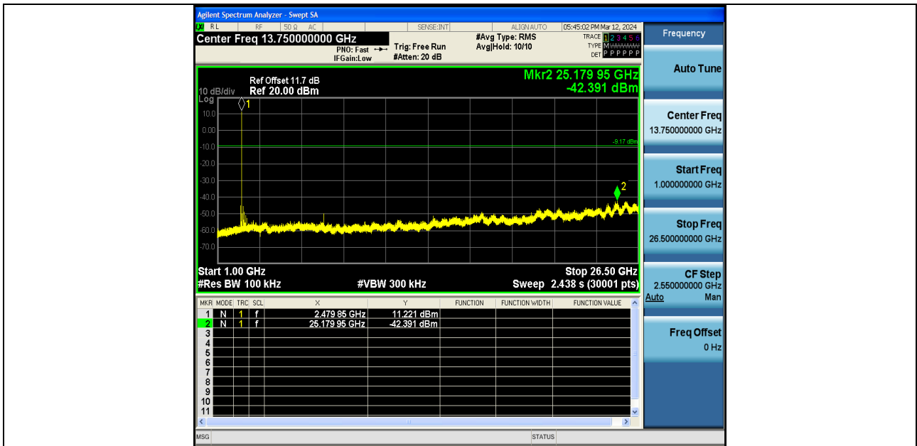
DH5-Ant1-2480-1000~26500-PASS
