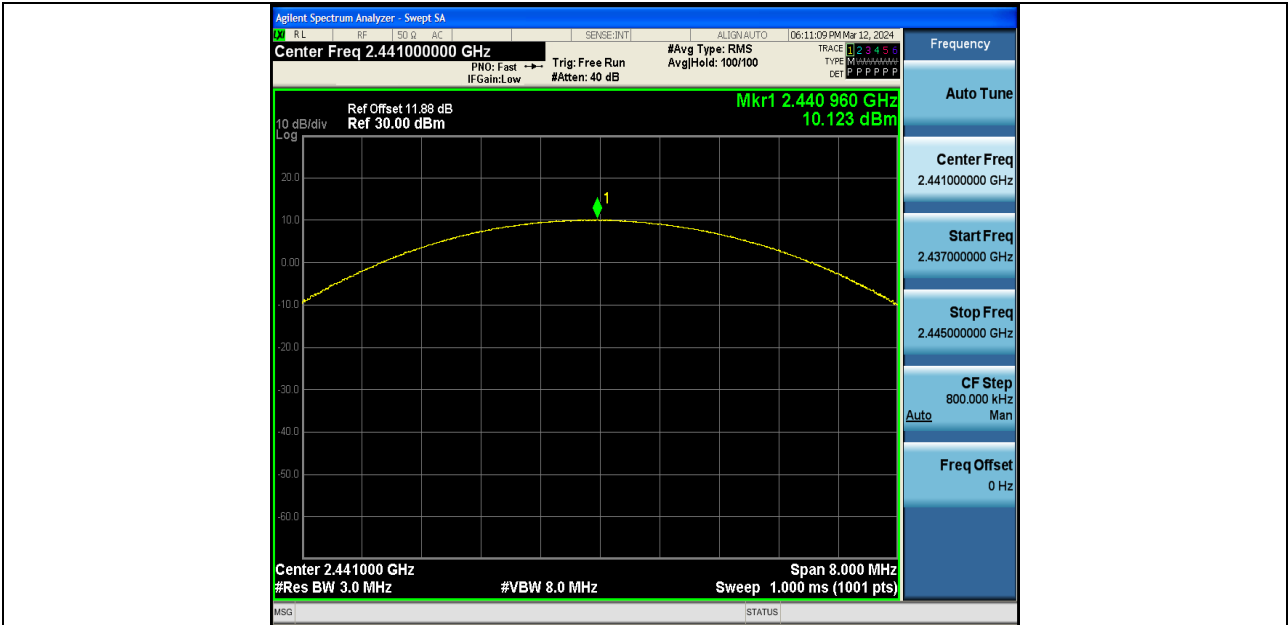
3DH5-Ant1-2441-PASS
