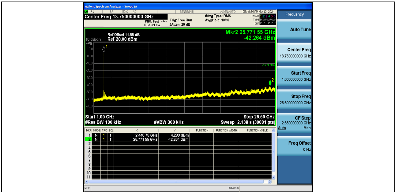
2DH5-Ant1-2441-1000~26500-PASS
