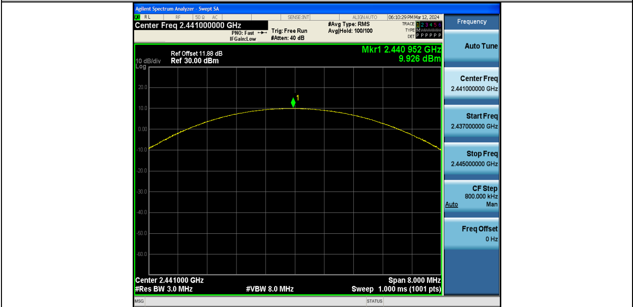
2DH5-Ant1-2441-PASS
