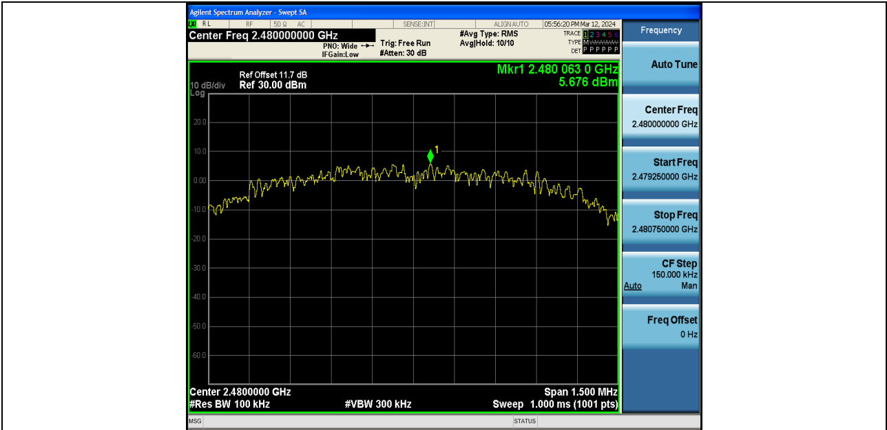
3DH5-Ant1-2480-0~Reference-PASS
