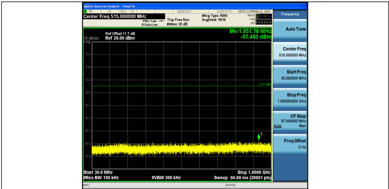
2DH5-Ant1-2480-30~1000-PASS
