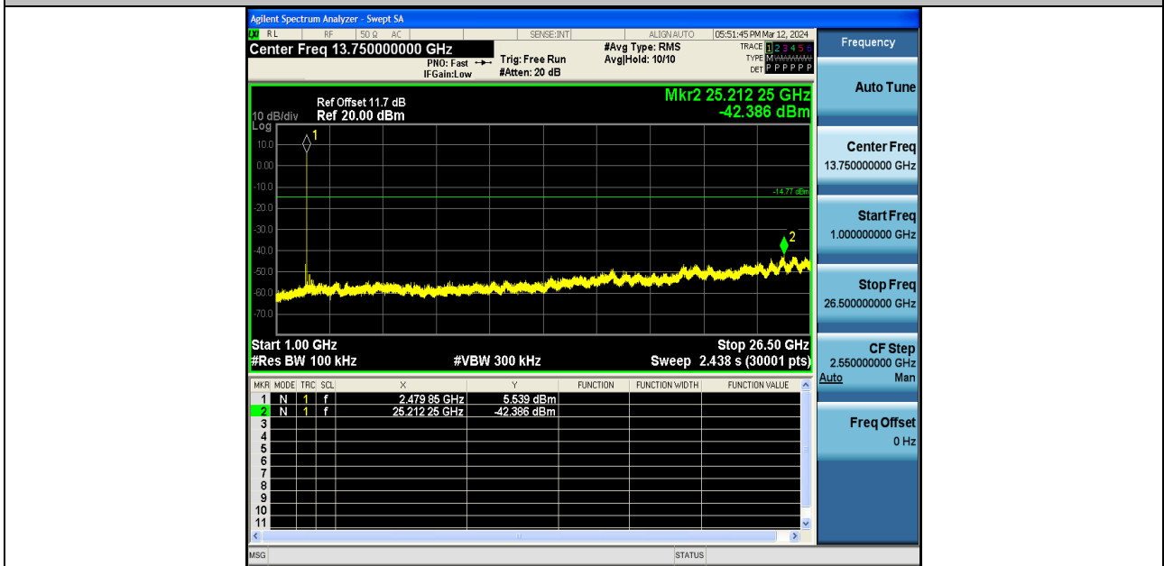
2DH5-Ant1-2480-1000~26500-PASS
