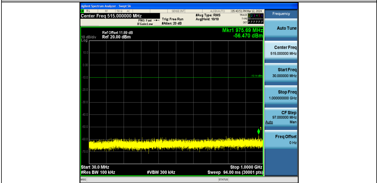
DH5-Ant1-2402-30~1000-PASS
