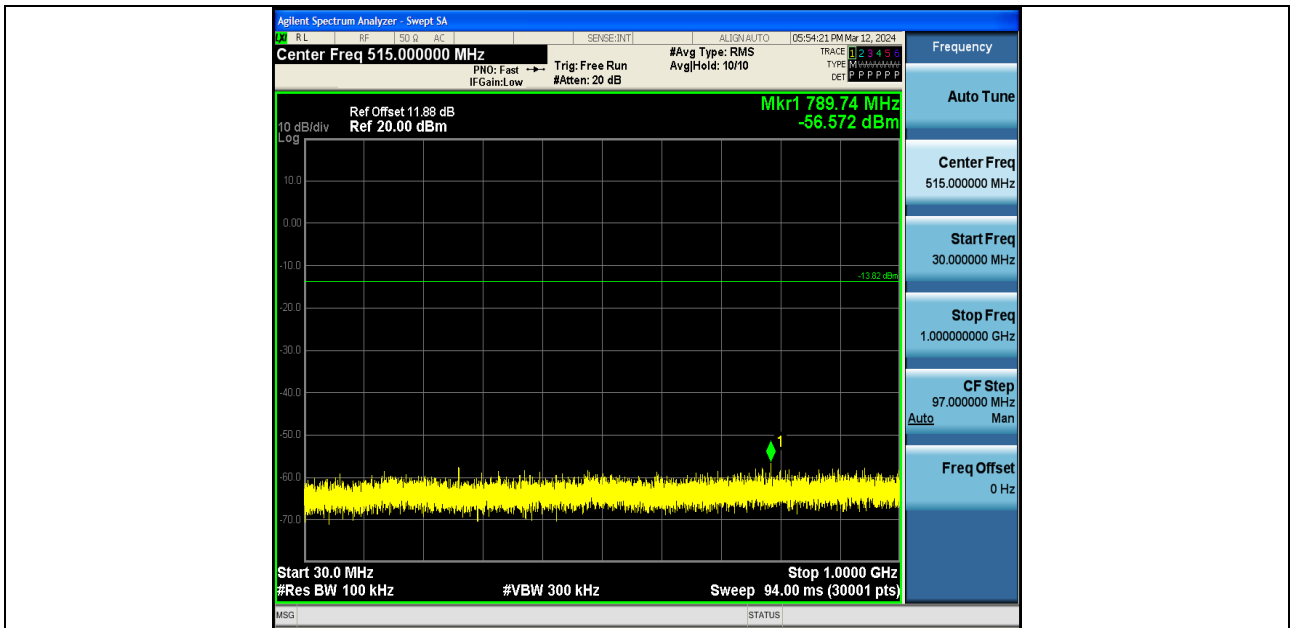
3DH5-Ant1-2441-30~1000-PASS
