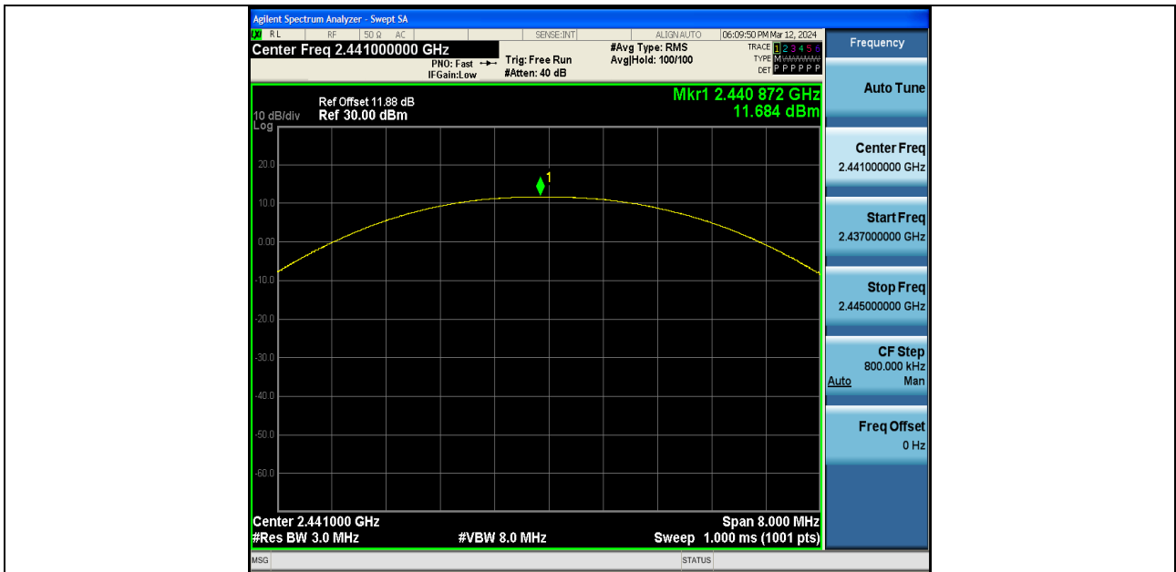
DH5-Ant1-2441-PASS
