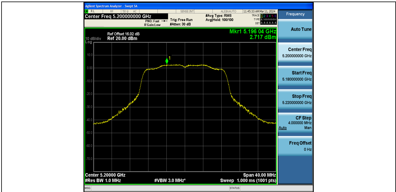
11N20SISO-Ant1-5200-PASS
