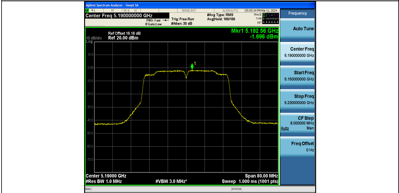
11AC40SISO-Ant2-5190-PASS
