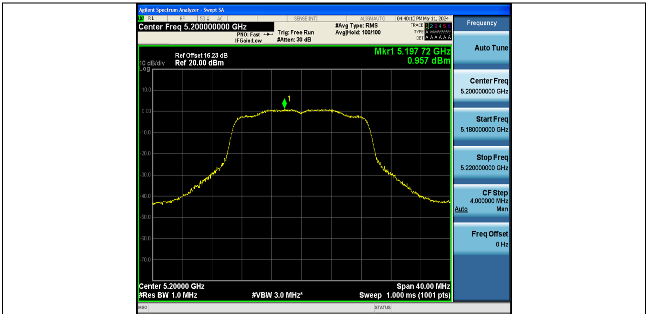
11AC20SISO-Ant1-5200-PASS
