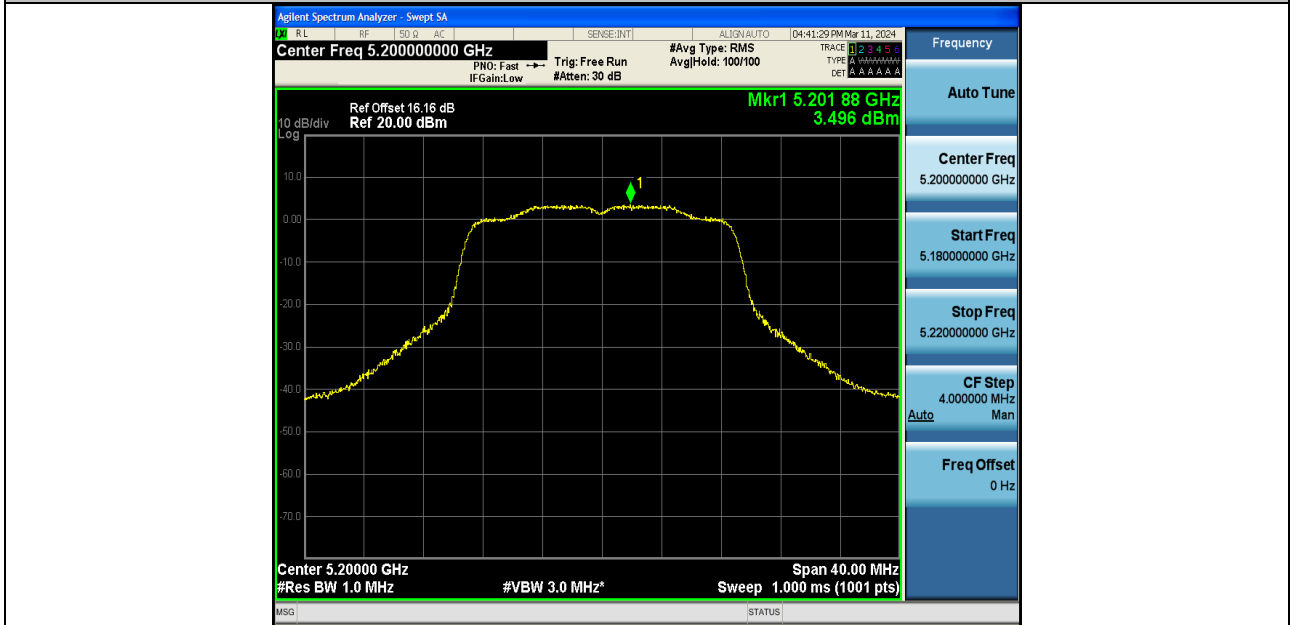
11AC20SISO-Ant2-5200-PASS
