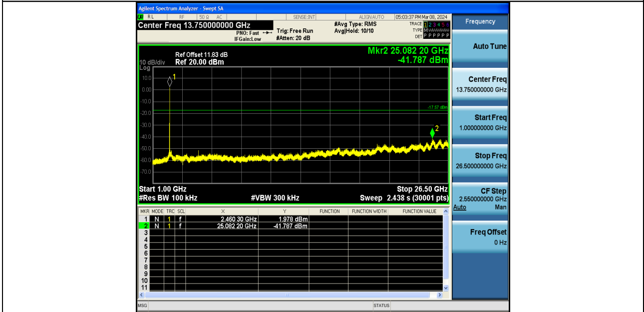
11B-Ant2-2462-1000~26500-PASS
