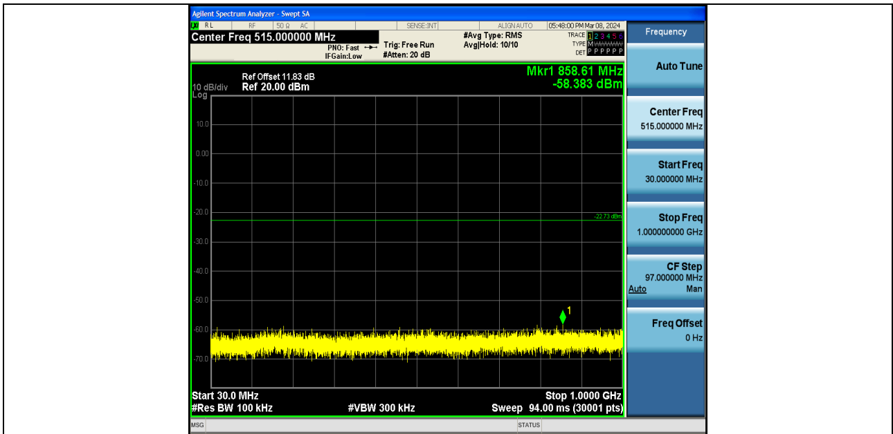
11N20SISO-Ant2-2462-30~1000-PASS
