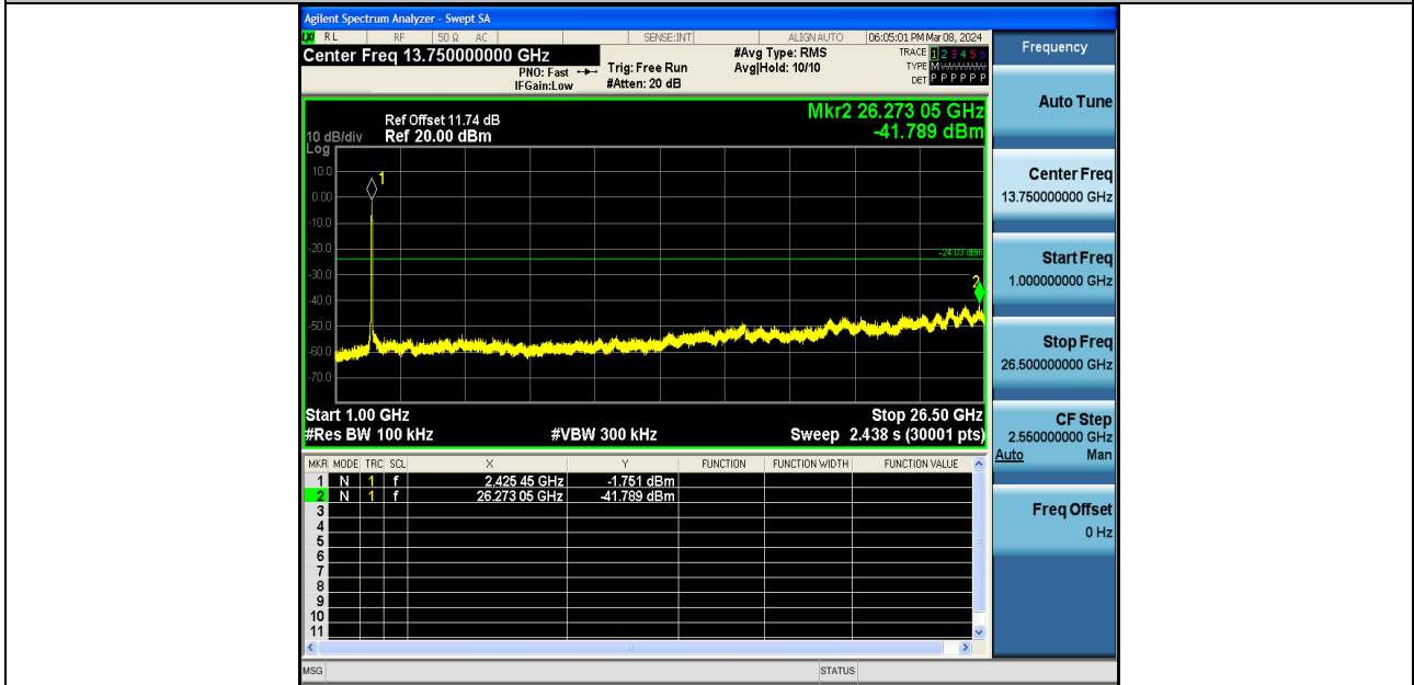
11N40SISO-Ant2-2437-1000~26500-PASS
