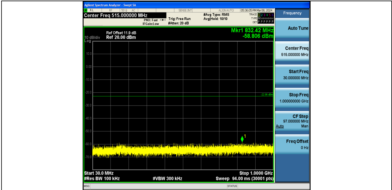
11N20SISO-Ant2-2412-30~1000-PASS
