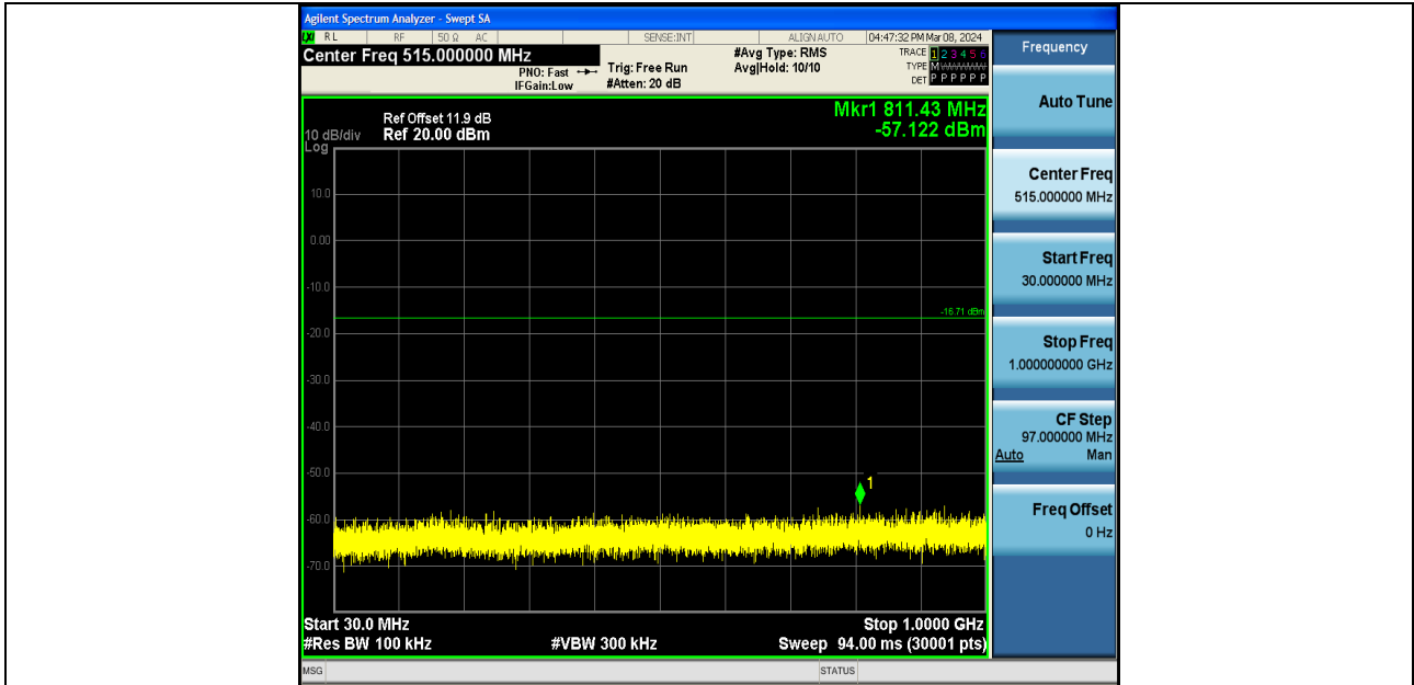
11B-Ant2-2412-30~1000-PASS
