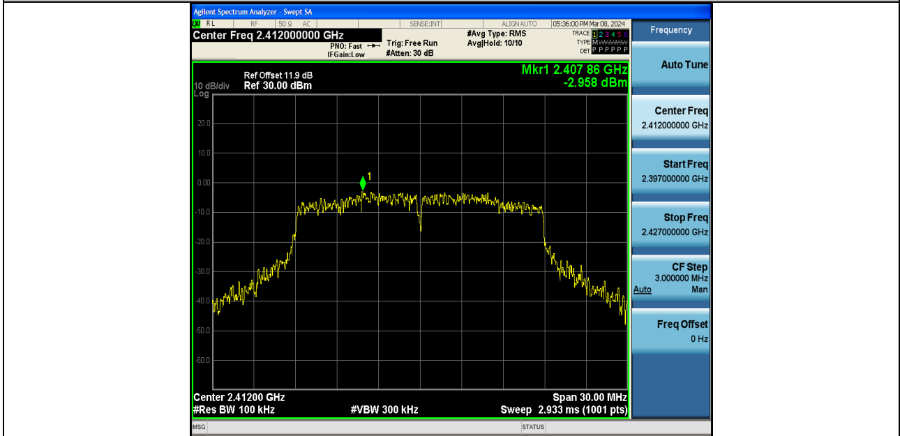
11N20SISO-Ant2-2412-0~Reference-PASS
