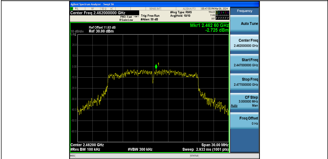
11N20SISO-Ant2-2462-0~Reference-PASS
