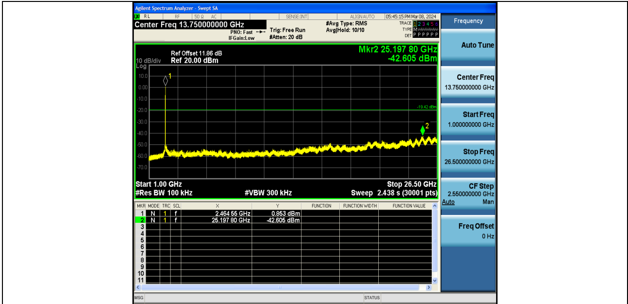
11N20SISO-Ant1-2462-1000~26500-PASS
