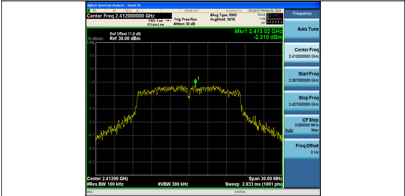
11G-Ant2-2412-0~Reference-PASS
