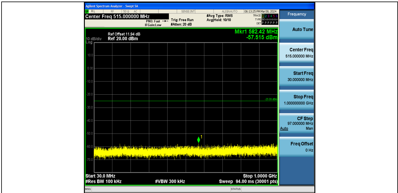
11N40SISO-Ant2-2452-30~1000-PASS
