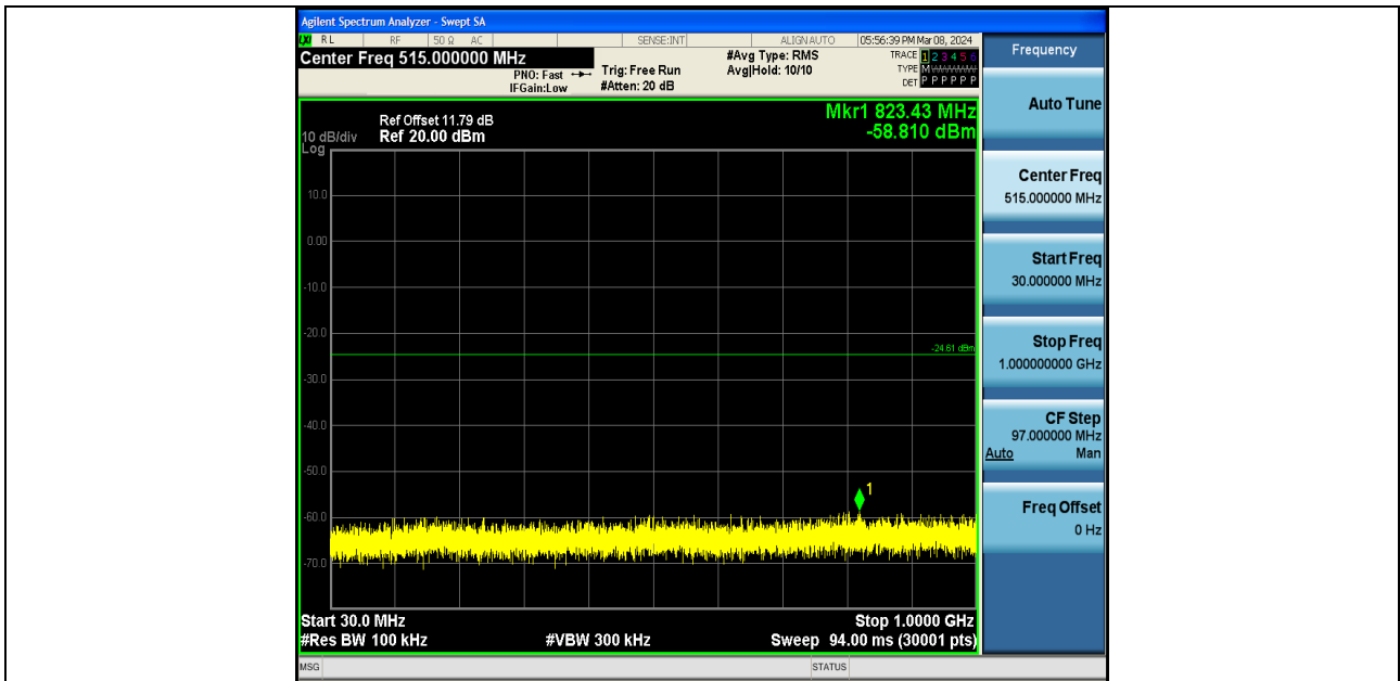
11N40SISO-Ant2-2422-30~1000-PASS
