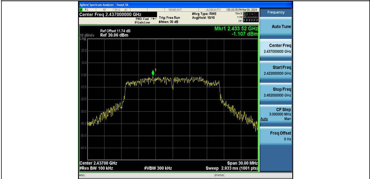
11G-Ant2-2437-0~Reference-PASS
