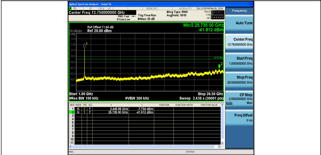
11N40SISO-Ant2-2452-1000~26500-PASS
