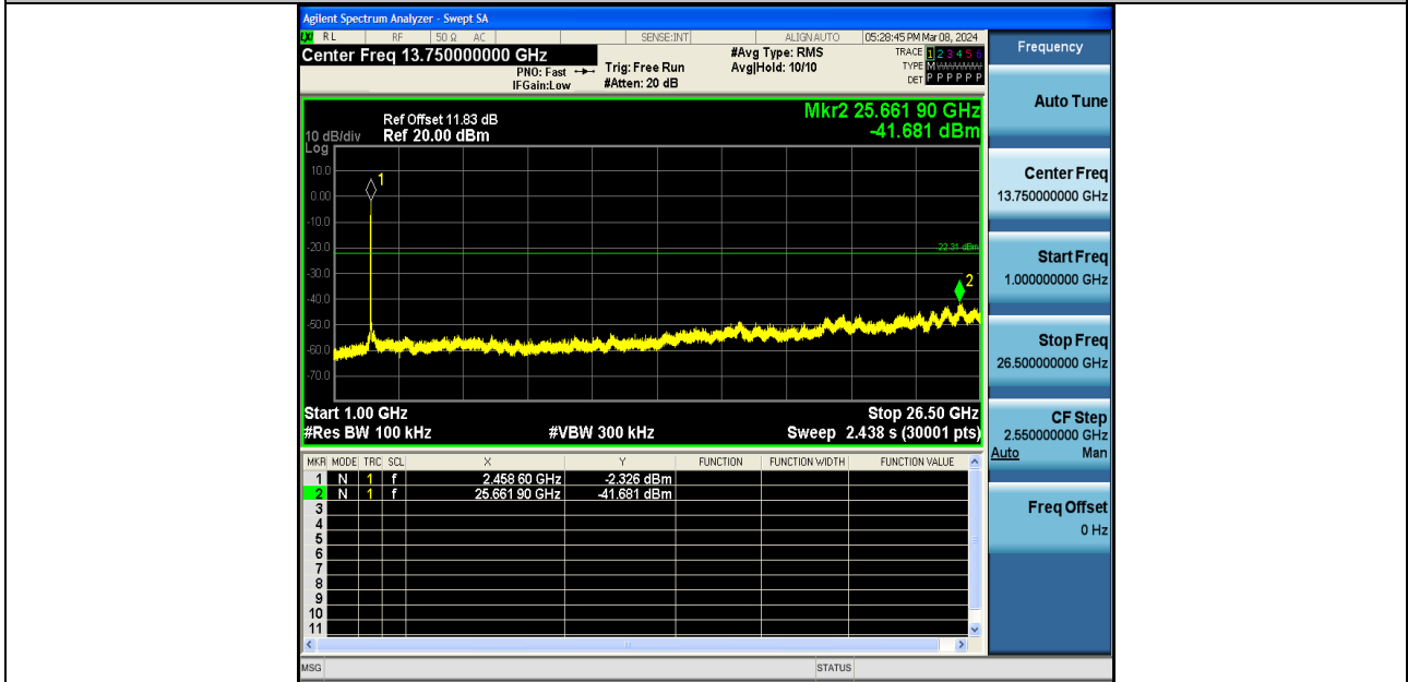
11G-Ant2-2462-1000~26500-PASS
