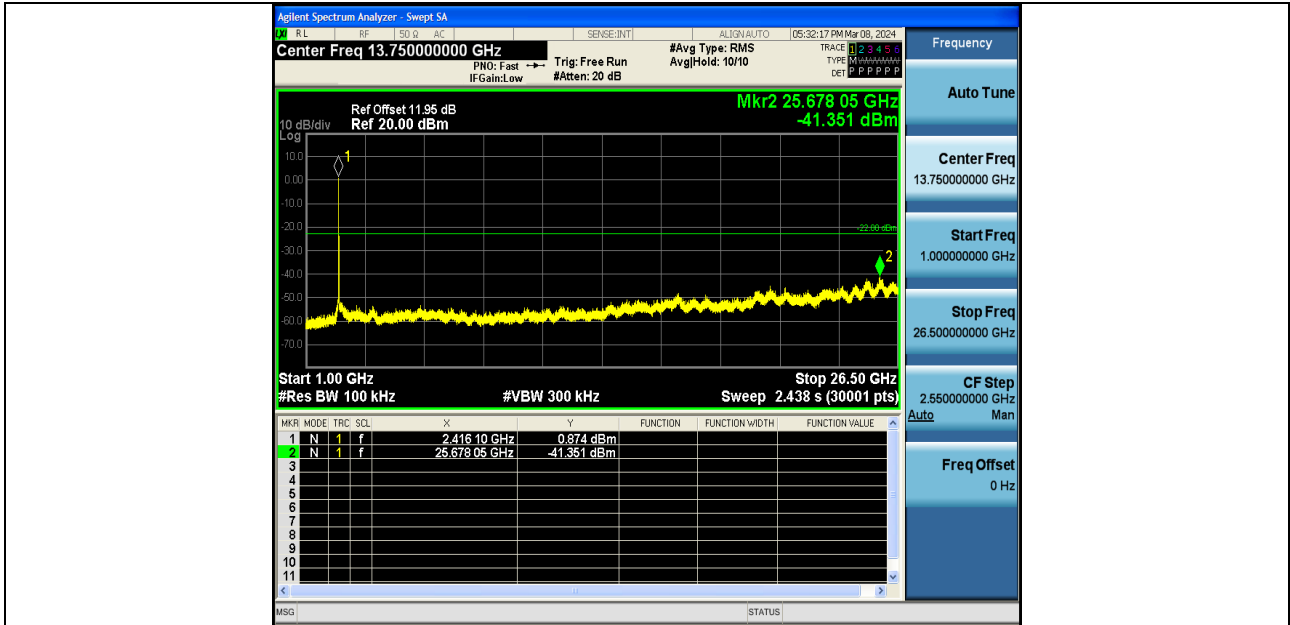
11N20SISO-Ant1-2412-1000~26500-PASS
