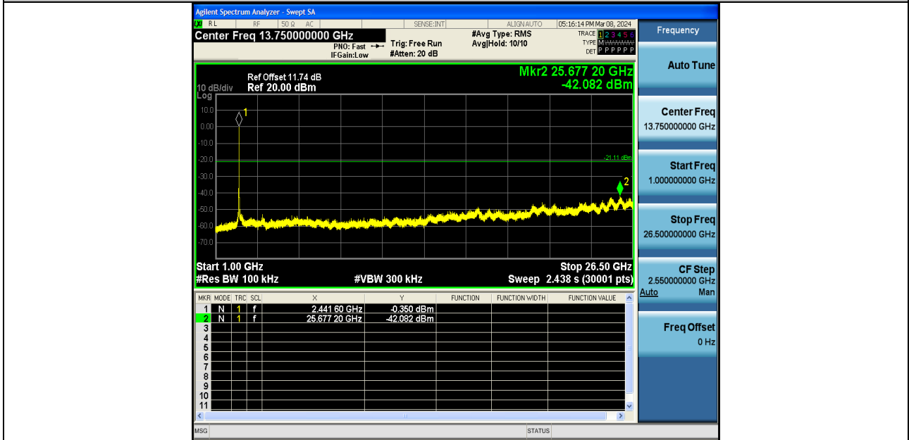
11G-Ant2-2437-1000~26500-PASS
