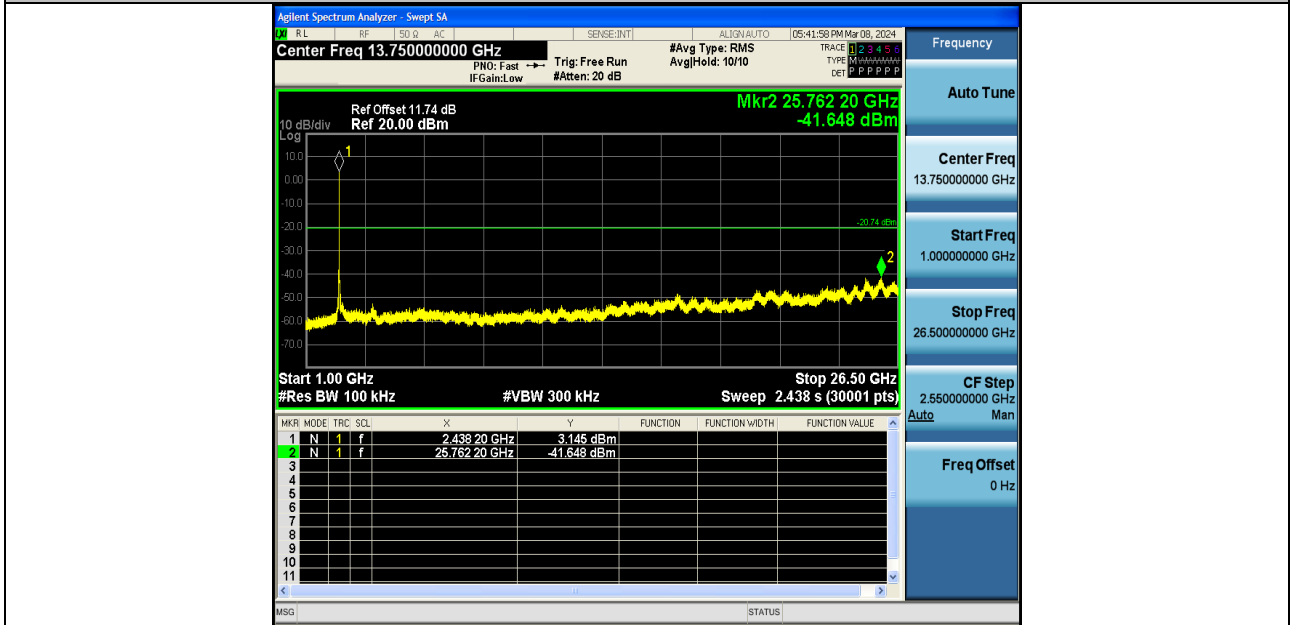
11N20SISO-Ant2-2437-1000~26500-PASS
