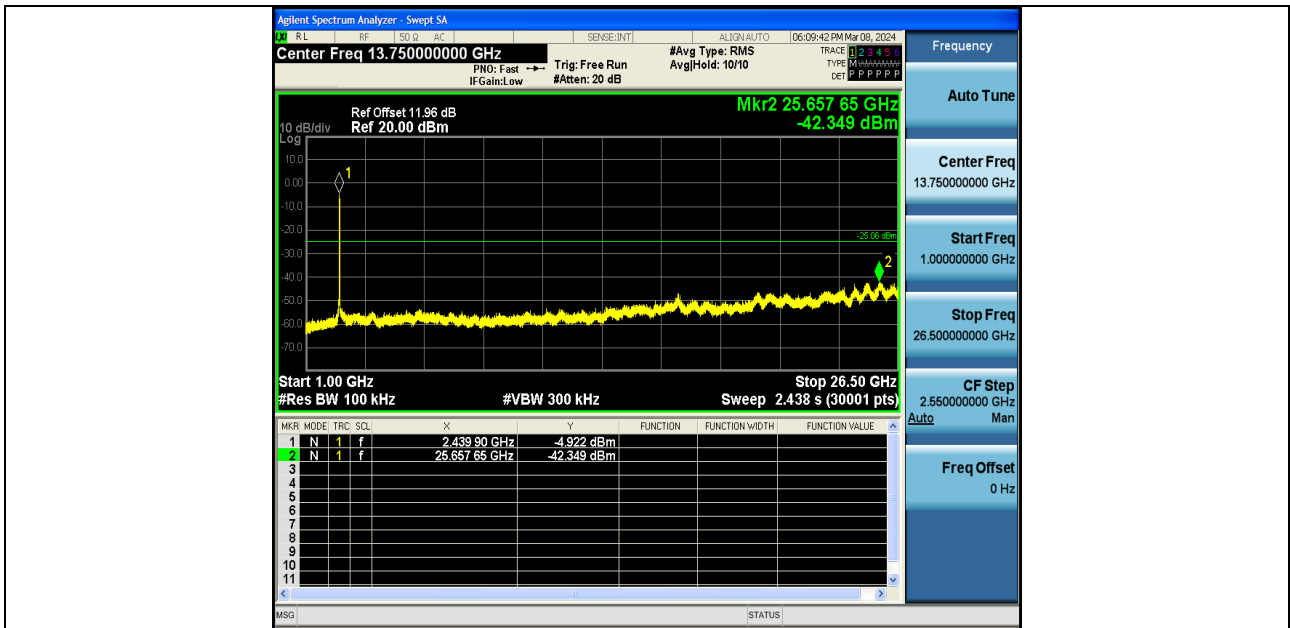
11N40SISO-Ant1-2452-1000~26500-PASS
