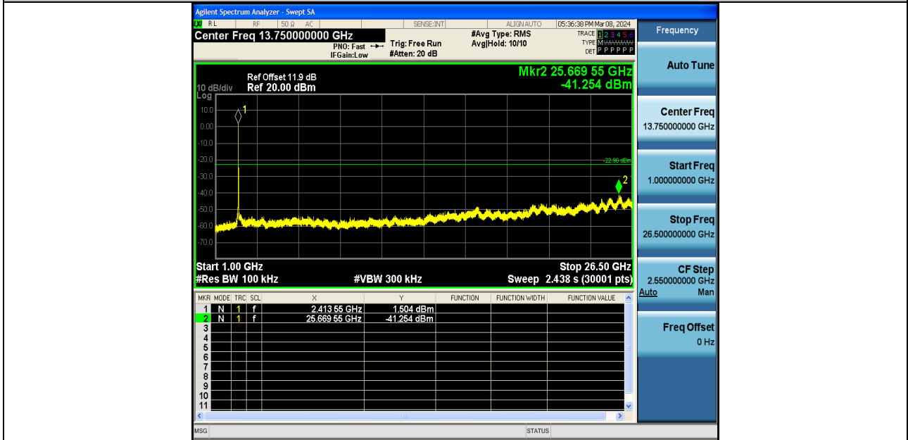
11N20SISO-Ant2-2412-1000~26500-PASS
