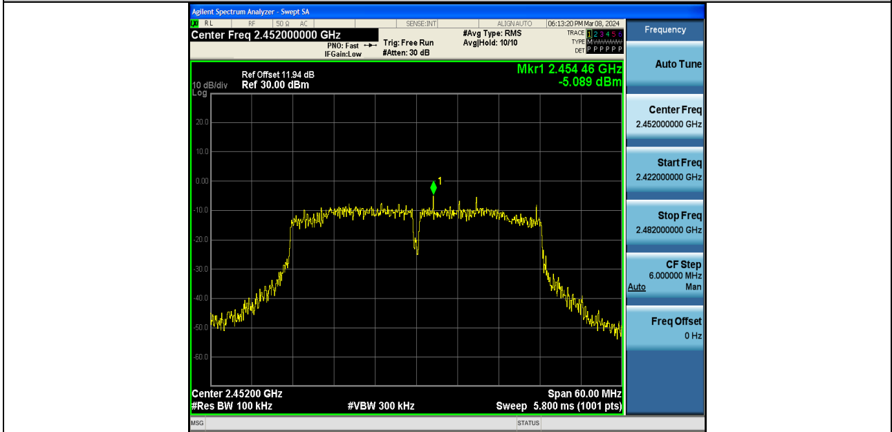
11N40SISO-Ant2-2452-0~Reference-PASS
