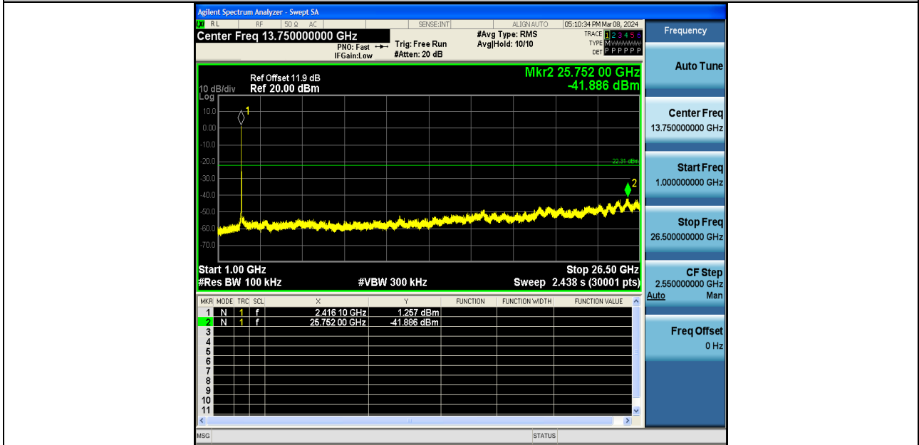
11G-Ant2-2412-1000~26500-PASS
