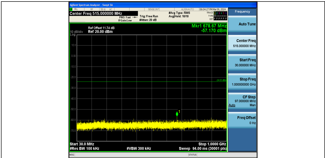
11N40SISO-Ant2-2437-30~1000-PASS
