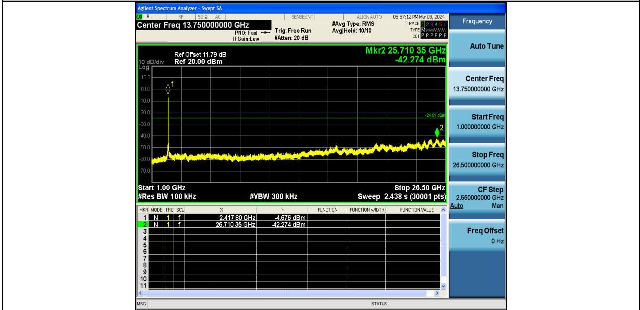
11N40SISO-Ant2-2422-1000~26500-PASS
