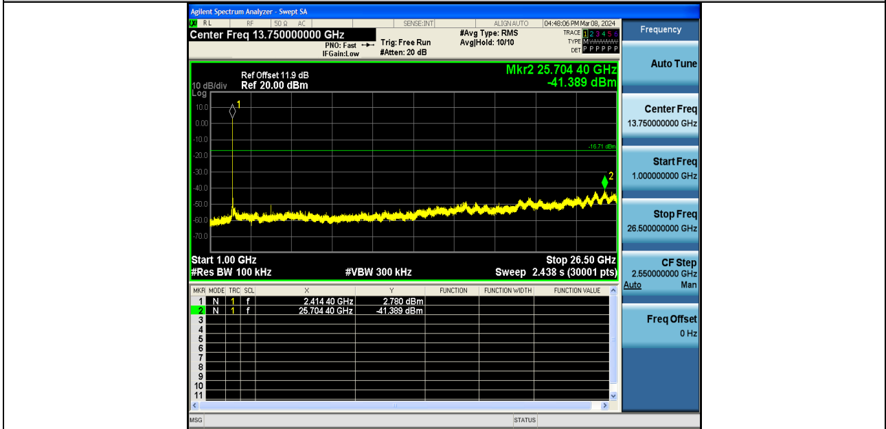
11B-Ant2-2412-1000~26500-PASS
