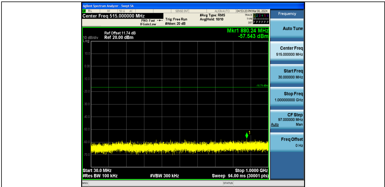
11B-Ant2-2437-30~1000-PASS
