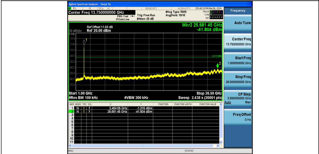
11N20SISO-Ant2-2462-1000~26500-PASS
