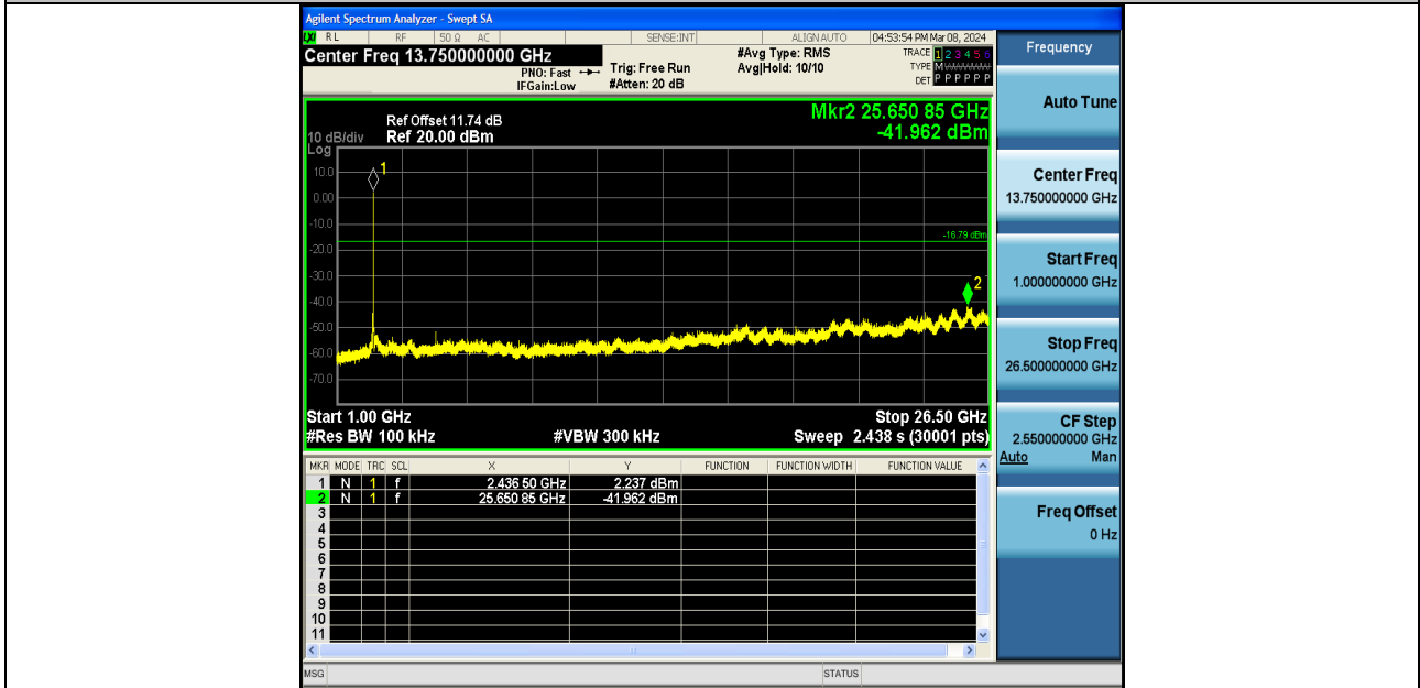
11B-Ant2-2437-1000~26500-PASS
