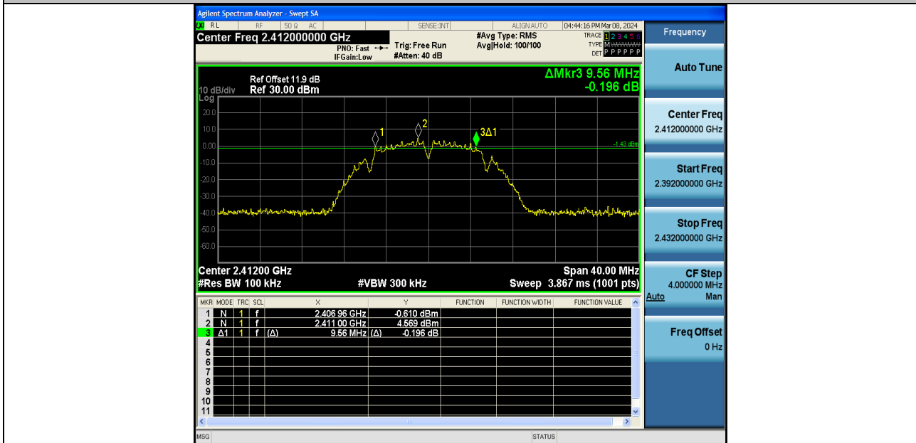
11B-Ant2-2412-PASS
