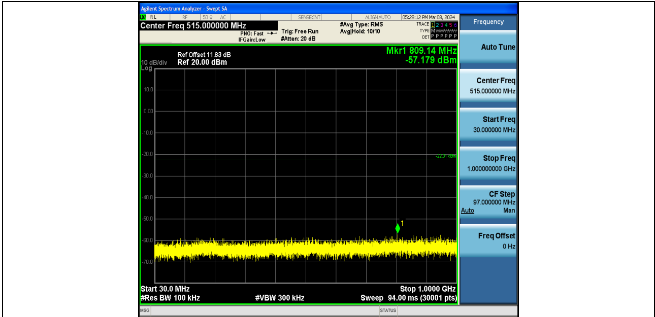
11G-Ant2-2462-30~1000-PASS
