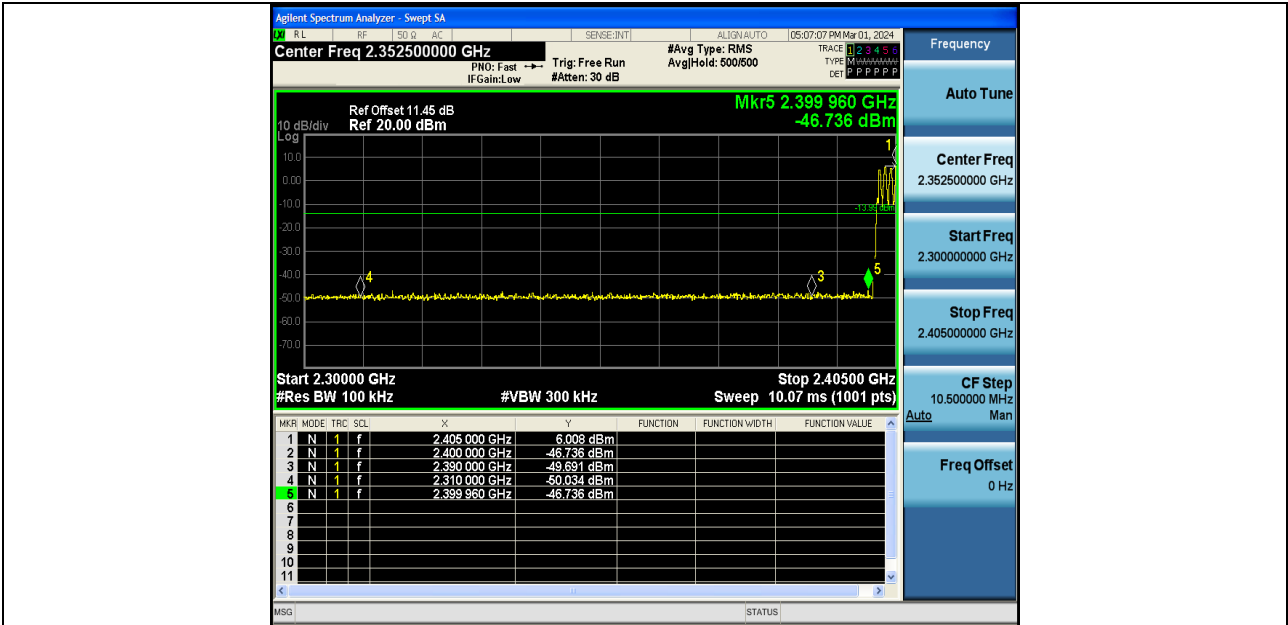
DH5-Ant1-Hop_2402-PASS
