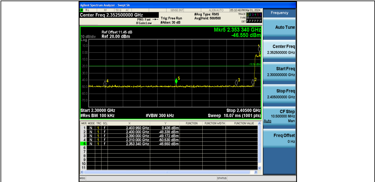
2DH5-Ant1-Hop_2402-PASS
