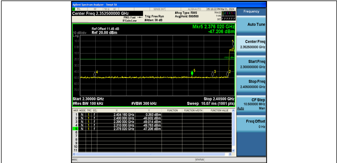
3DH5-Ant1-Hop_2402-PASS
