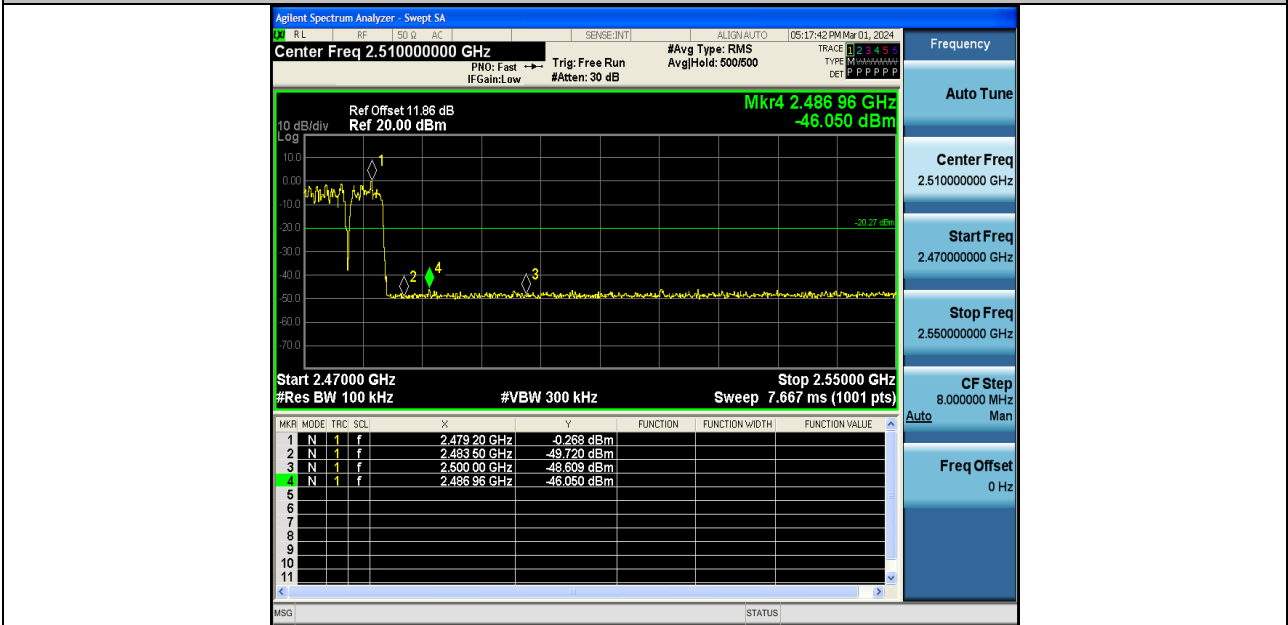
2DH5-Ant1-Hop_2480-PASS
