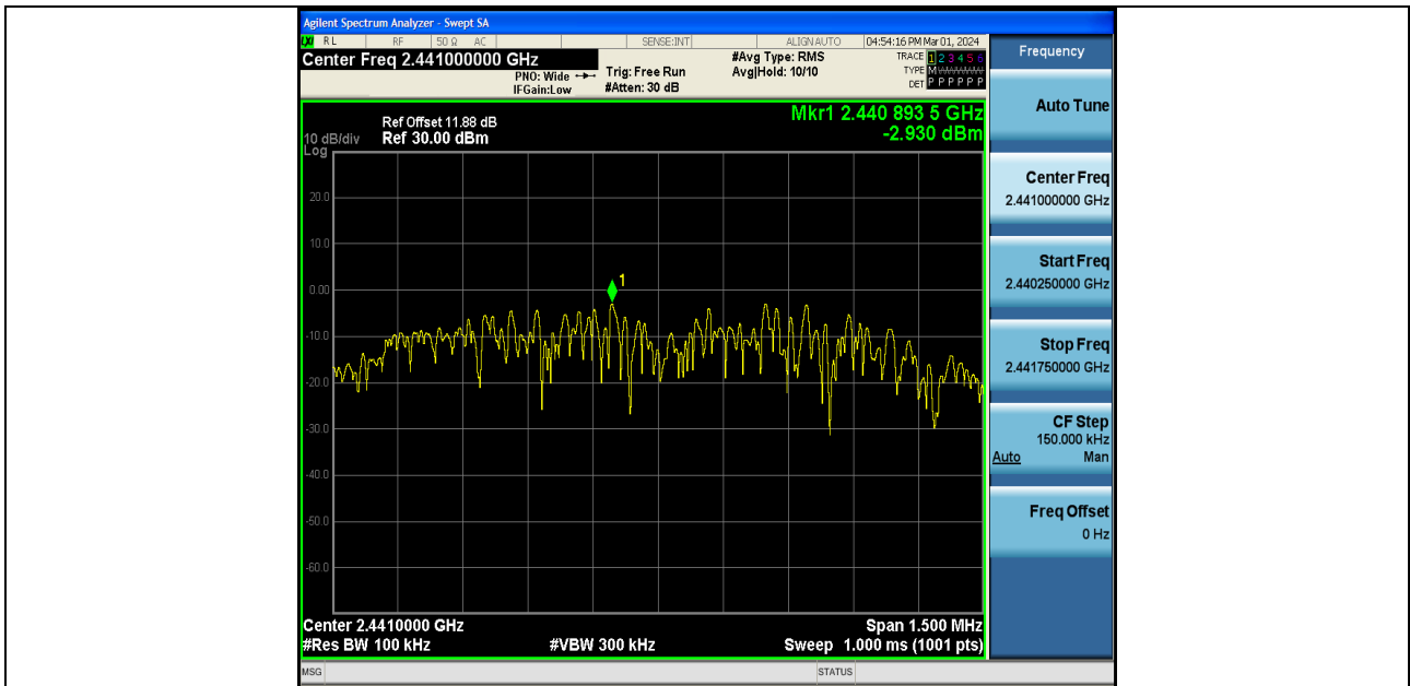
2DH5-Ant1-2441-0~Reference-PASS
