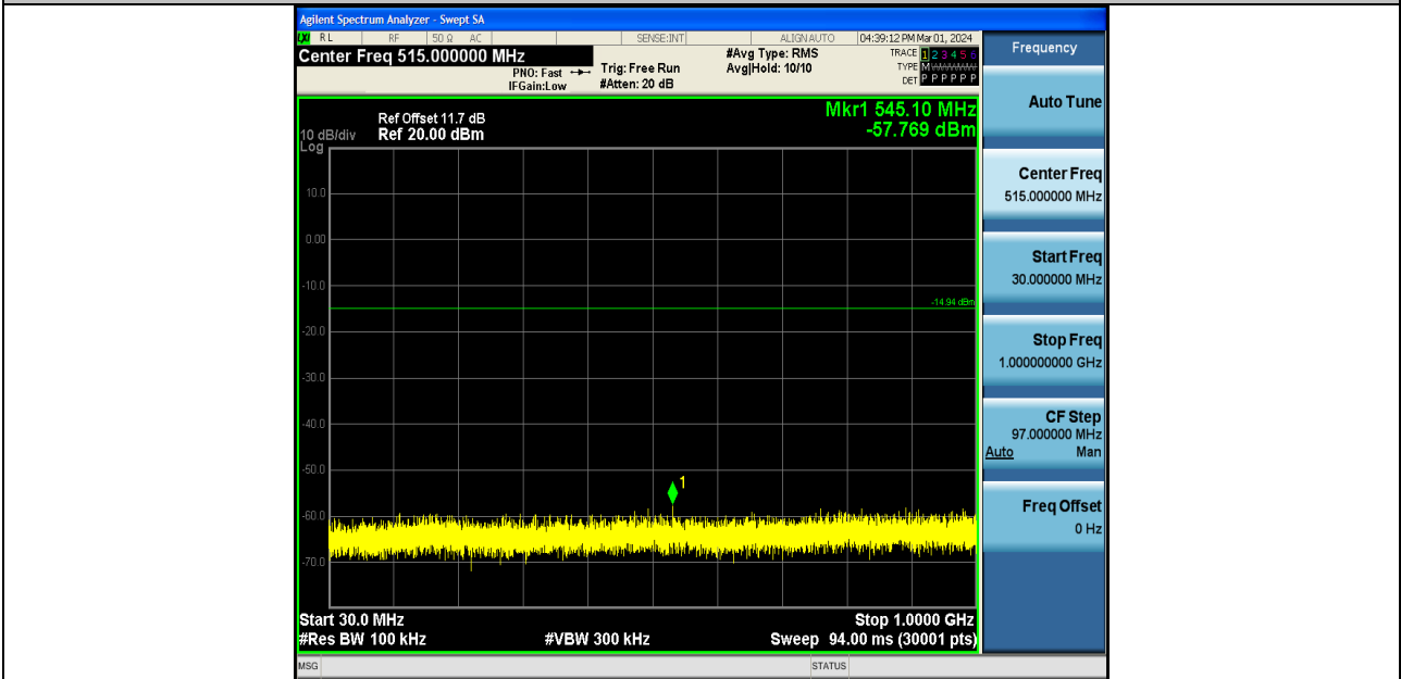
DH5-Ant1-2480-30~1000-PASS
