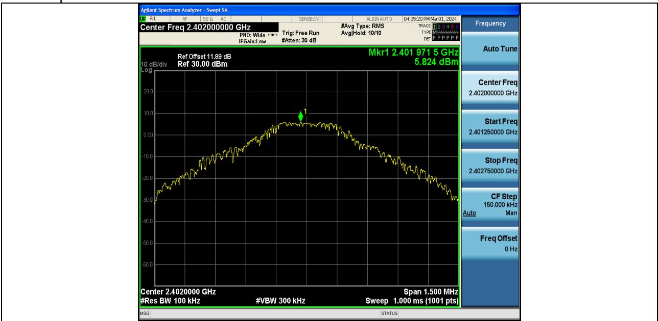
DH5-Ant1-2402-0~Reference-PASS
