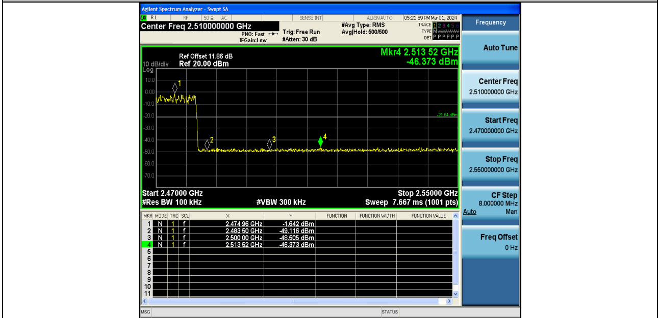
3DH5-Ant1-Hop_2480-PASS
