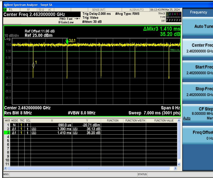
NTVN-11G-Ant1-2462
