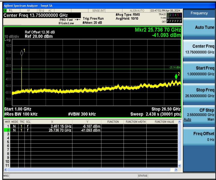
11B-Ant1-2462-1000~26500-PASS
