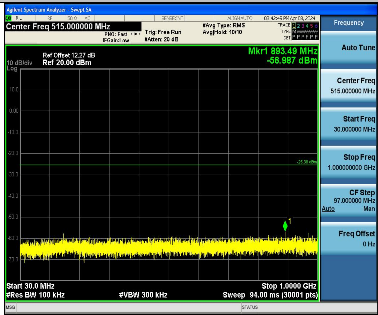
11B-Ant1-2437-30~1000-PASS
