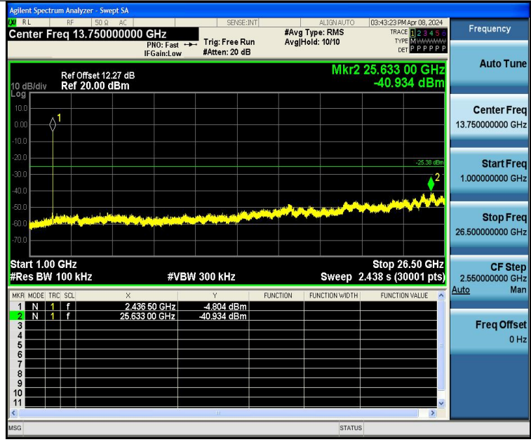
11B-Ant1-2437-1000~26500-PASS
