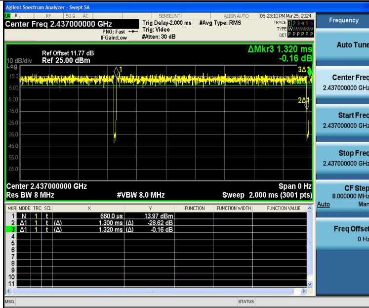
NTNV-11N20SISO-Ant1-2437
