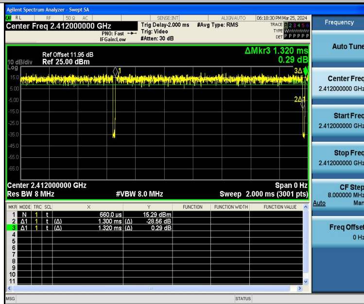
NTVN-11N20SISO-Ant1-2412
