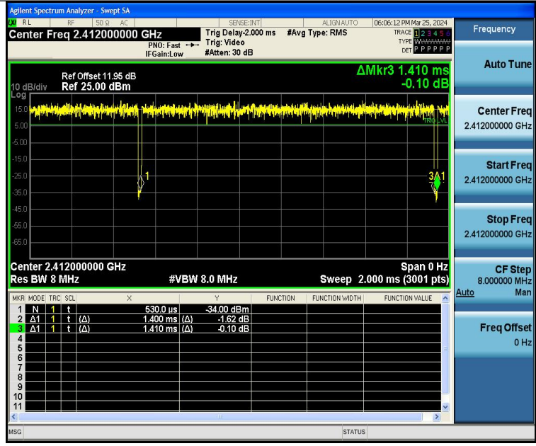
NTNV-11G-Ant1-2412
