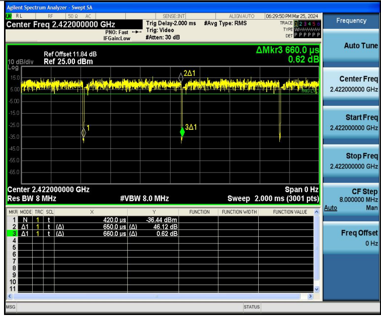
NTNV-11N40SISO-Ant1-2422
