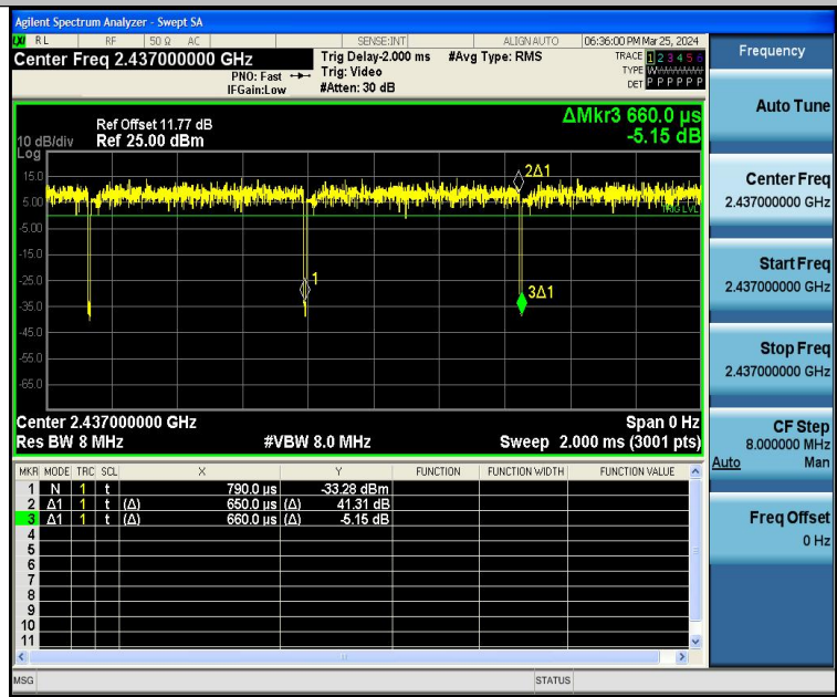
NTNV-11N40SISO-Ant1-2437
