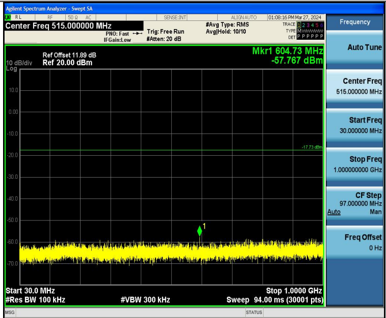
BLE_1M-Ant1-2402-30~1000-PASS
