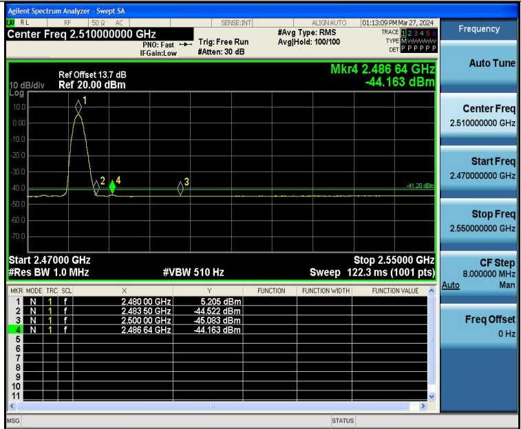
BLE_1M-Ant1-2480-PASS
