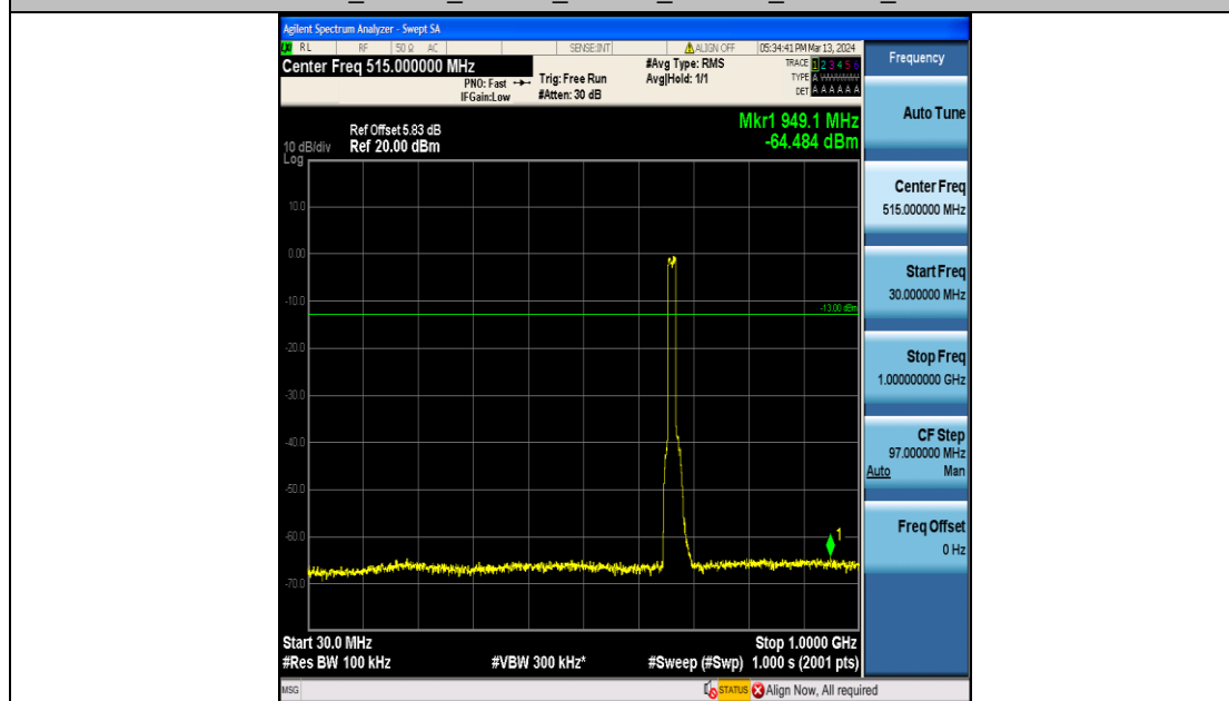
Band71_15MHz_16QAM_133197_75RB#0_30~1000_30~1000
