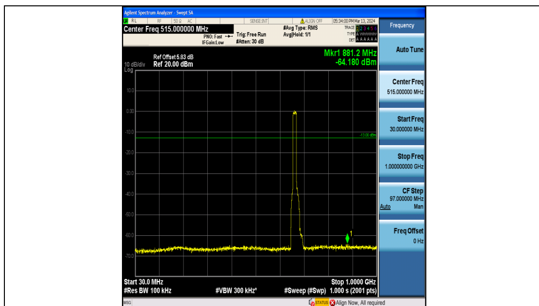
Band71_15MHz_QPSK_133197_75RB#0_30~1000_30~1000
