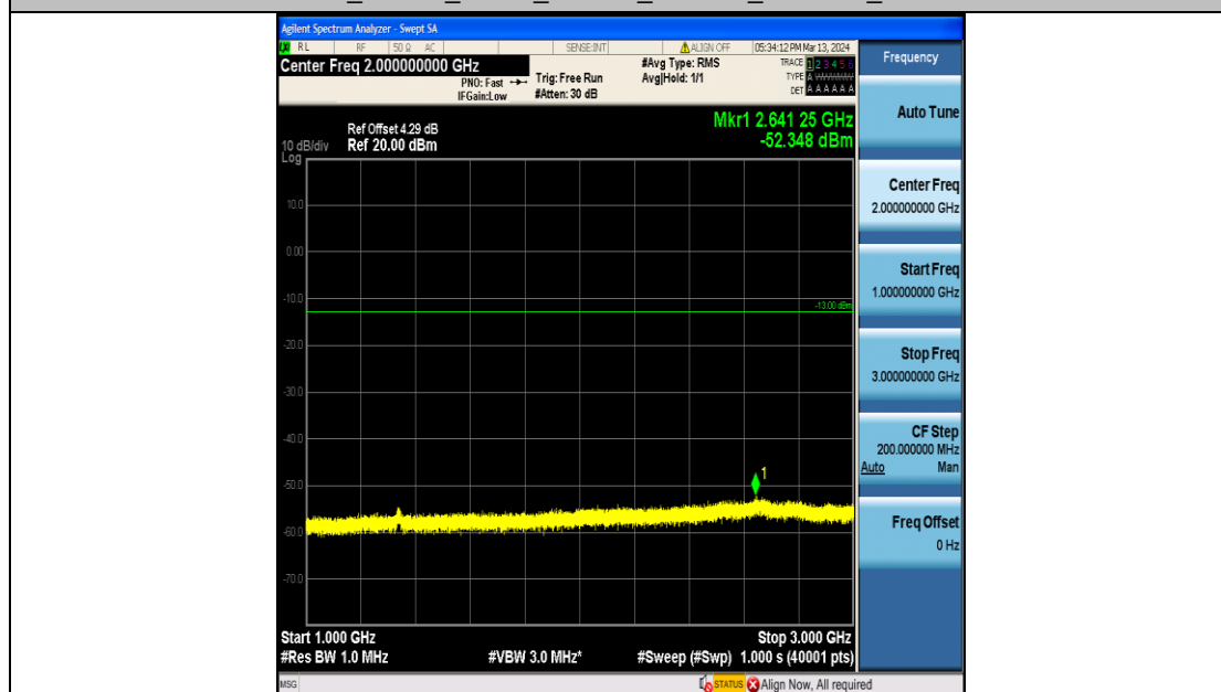
Band71_15MHz_QPSK_133197_75RB#0_1000~3000_1000~3000
