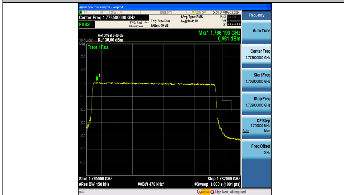
Band66_15MHz_16QAM_132597_75RB#0
