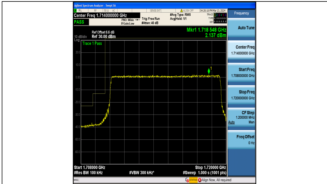
Band66_10MHz_QPSK_132022_50RB#0
