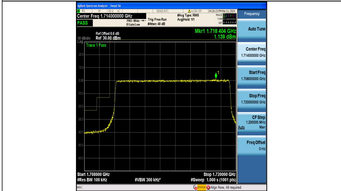
Band66_10MHz_16QAM_132022_50RB#0
