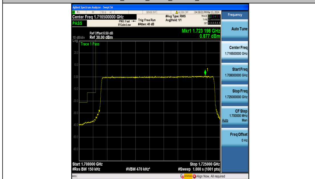
Band66_15MHz_16QAM_132047_75RB#0
