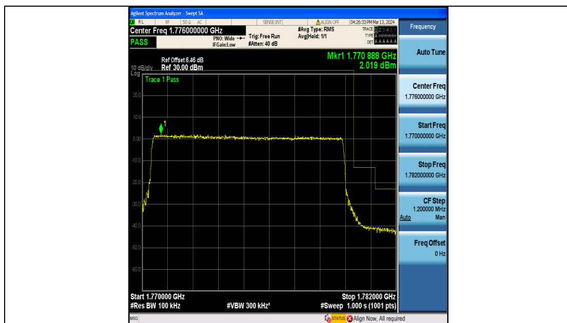
Band66_10MHz_QPSK_132622_50RB#0
