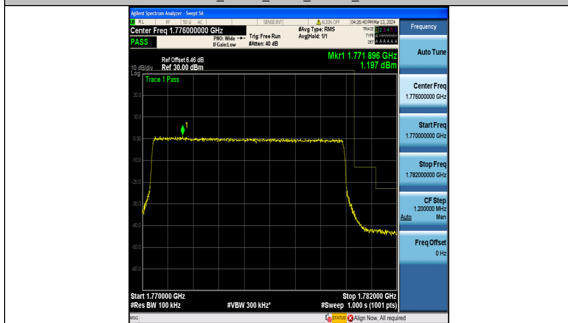
Band66_10MHz_16QAM_132622_50RB#0
