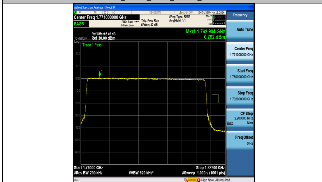
Band66_20MHz_16QAM_132572_100RB#0
