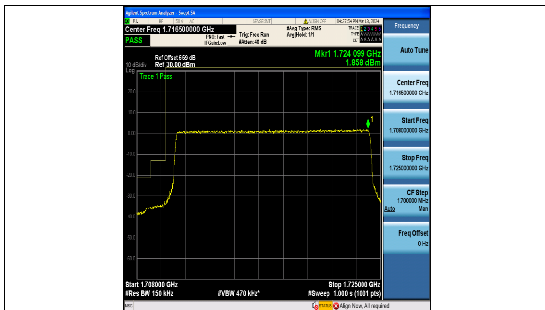
Band66_15MHz_QPSK_132047_75RB#0
