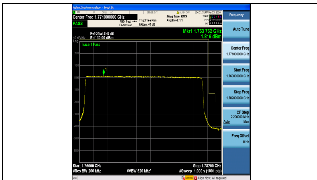
Band66_20MHz_QPSK_132572_100RB#0
