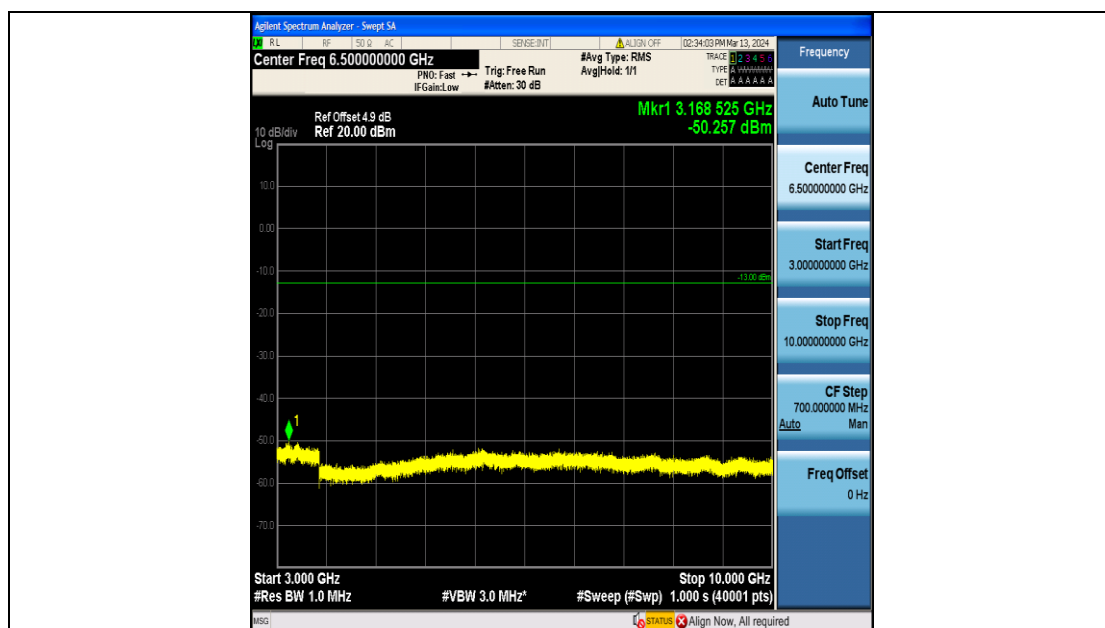
Band12_3MHz_QPSK_23165_15RB#0_3000~10000_3000~10000
