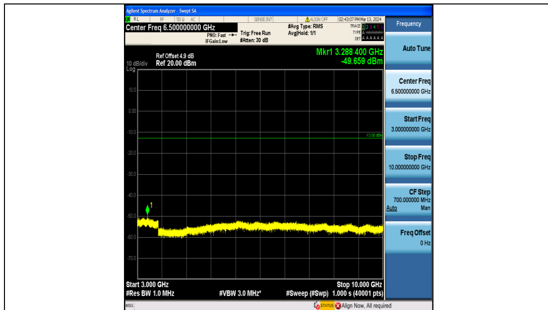
Band12_5MHz_QPSK_23035_25RB#0_3000~10000_3000~10000
