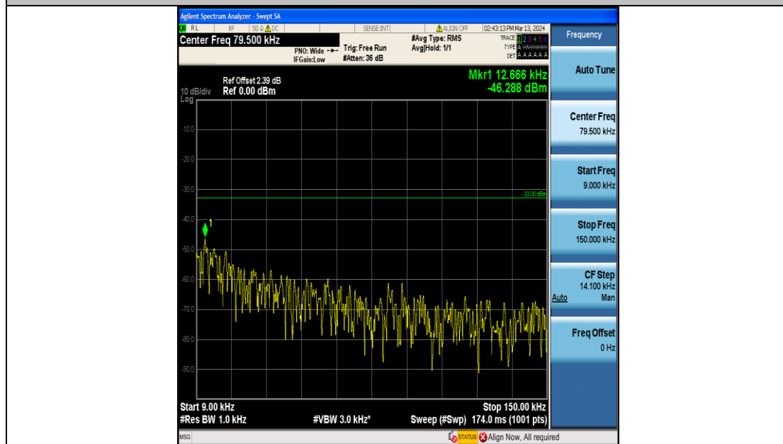
Band12_5MHz_16QAM_23035_25RB#0_0.009~0.15_0.009~0.15
