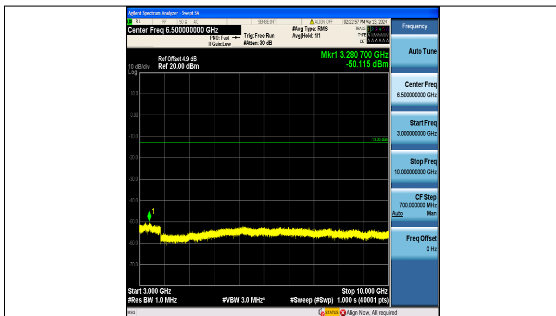
Band12_1.4MHz_QPSK_23173_6RB#0_3000~10000_3000~10000
