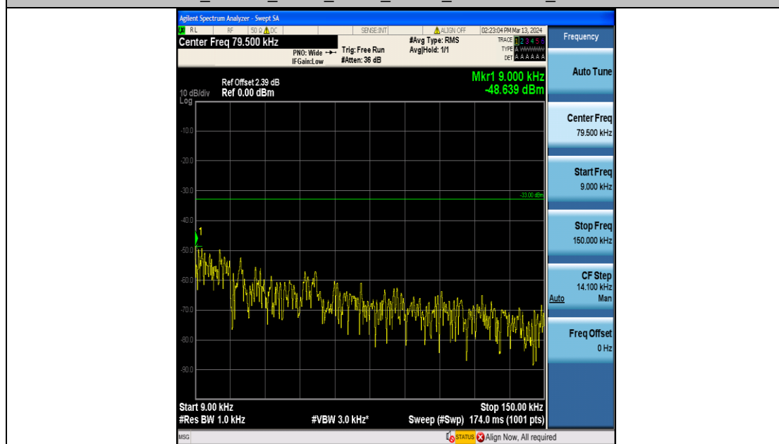
Band12_1.4MHz_16QAM_23173_6RB#0_0.009~0.15_0.009~0.15
