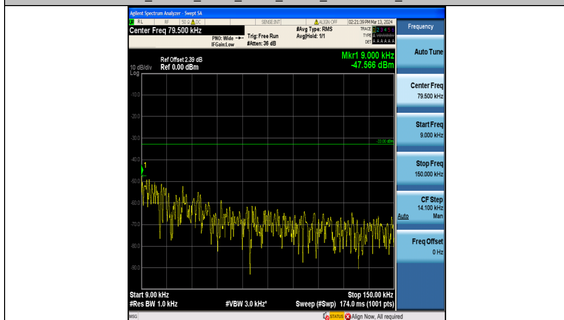
Band12_1.4MHz_16QAM_23095_6RB#0_0.009~0.15_0.009~0.15
