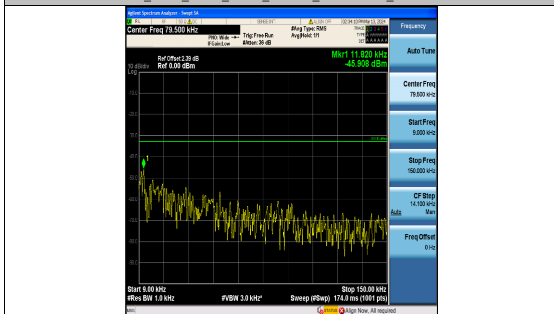
Band12_3MHz_16QAM_23165_15RB#0_0.009~0.15_0.009~0.15
