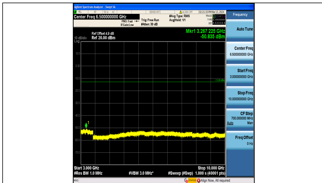
Band12_1.4MHz_QPSK_23095_6RB#0_3000~10000_3000~10000
