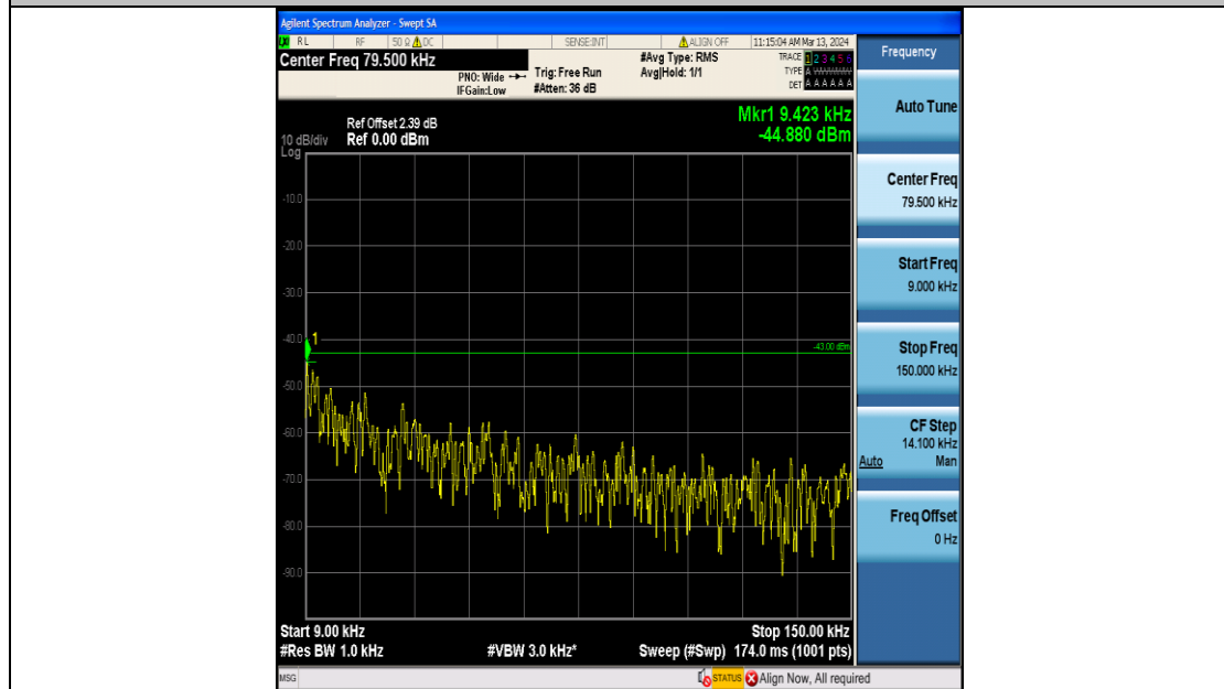
Band4_5MHz_QPSK_20375_25RB#0_0.009~0.15_0.009~0.15
