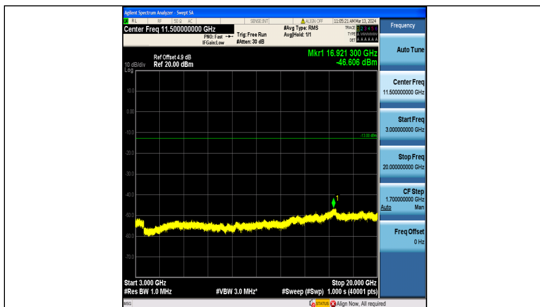
Band4_3MHz_16QAM_20385_15RB#0_3000~20000_3000~20000
