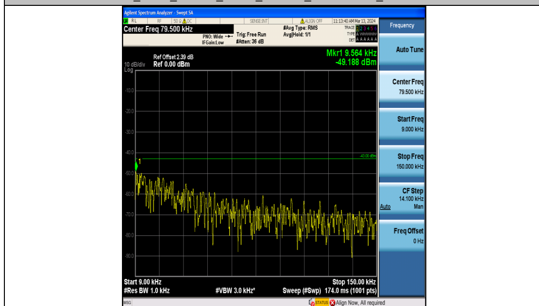
Band4_5MHz_QPSK_20175_25RB#0_0.009~0.15_0.009~0.15
