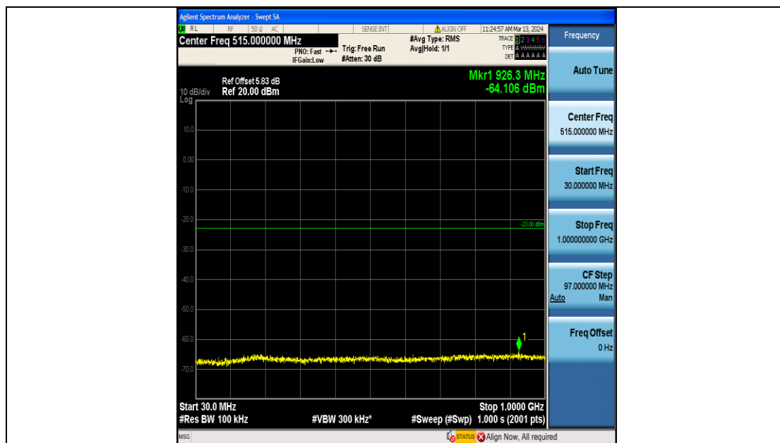
Band4_10MHz_16QAM_20175_50RB#0_30~1000_30~1000
