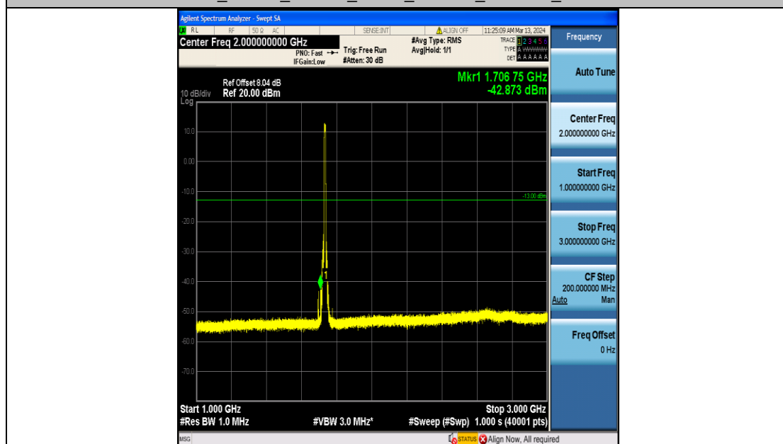
Band4_10MHz_16QAM_20175_50RB#0_1000~3000_1000~3000
