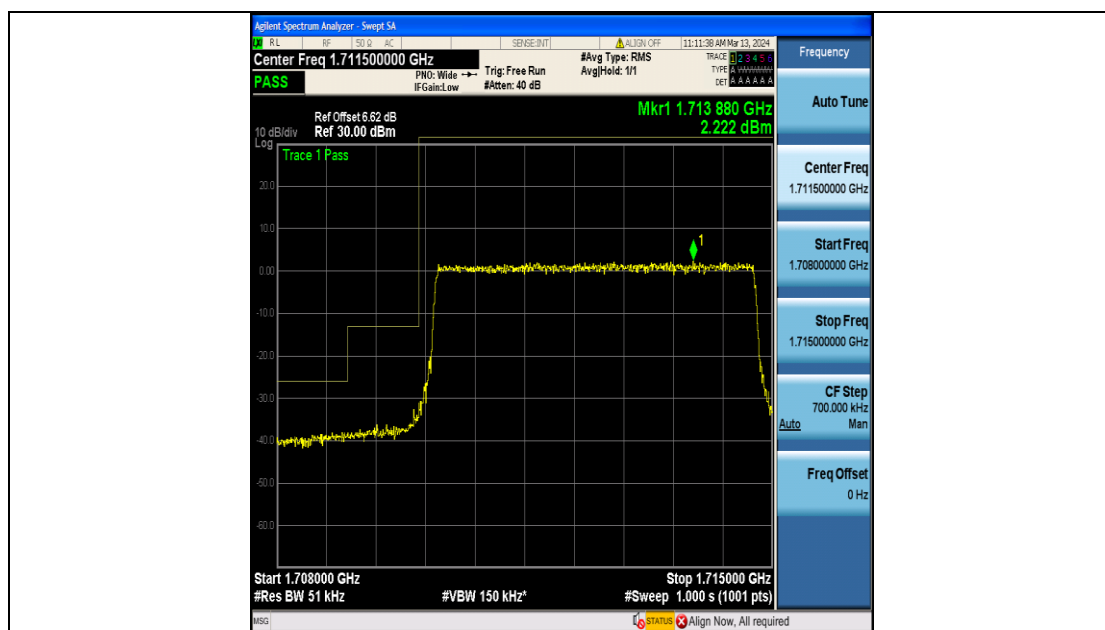
Band4_5MHz_QPSK_19975_25RB#0
