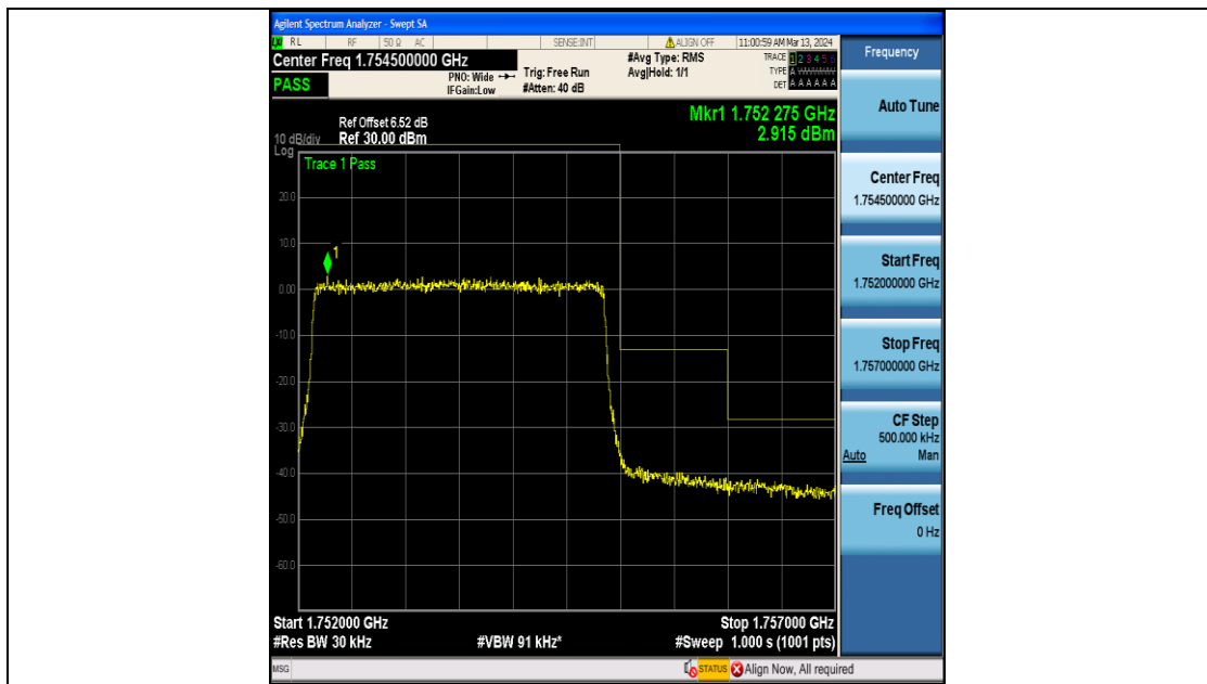
Band4_3MHz_QPSK_20385_15RB#0
