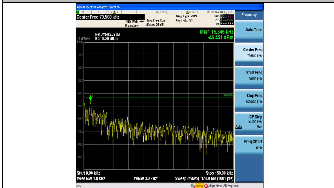
Band4_3MHz_QPSK_20175_15RB#0_0.009~0.15_0.009~0.15
