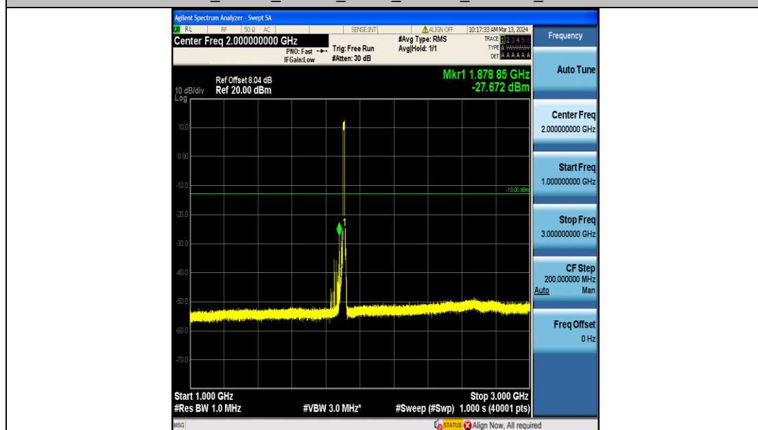
Band2_10MHz_16QAM_19150_50RB#0_1000~3000_1000~3000
