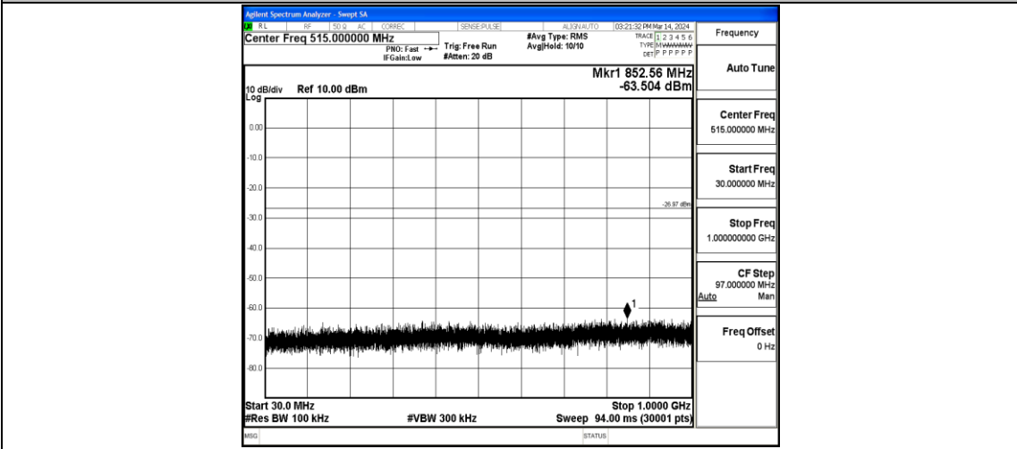
11N40MIMO-Ant1-2452-30~1000-PASS
