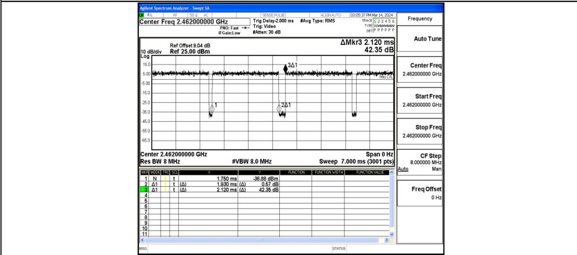
NTVN-11N20MIMO-Ant2-2462
