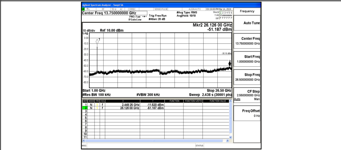
11N40MIMO-Ant2-2437-1000~26500-PASS
