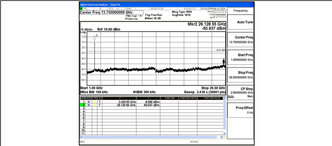
11N40MIMO-Ant1-2437-1000~26500-PASS
