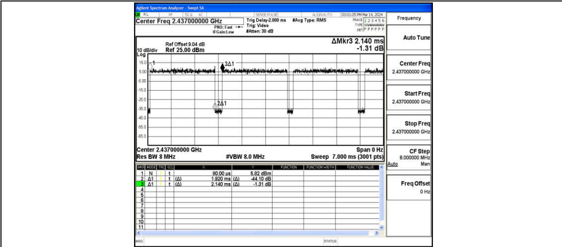
NTVN-11N20MIMO-Ant2-2437
